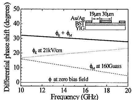
Figure 6. Measured differential phase shift ( \Delta\phi = \phi(\text{no bias}) - \phi(\text{bias}) ) from coplanar transmission lines fabricated on ferroelectric BST films grown on ferrite (111)YIG with electric dc bias field of 21kV/cm and/or magnetic field of 160Gauss.
