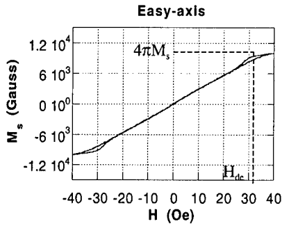
Figure (10a). Easy axis hysteresis loop of the patterned CZN film. H_{dc} \approx 32 \text{ Oe} .
