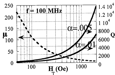
Figure (2a). Variation of \mu_{\text{sr}} and Q_{\text{sr}} of CZN film with H_T as computed from (4) and (6) at 100 MHz.
