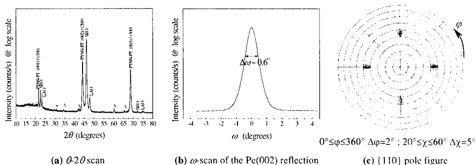
Figure 1 : XRD patterns of a PYbN-PT (60/40) thin film deposited at 655°C on a SRO/LAO substrate *→Perovskite (Pe) \Delta →Pyrochlore (Py), PbO x
