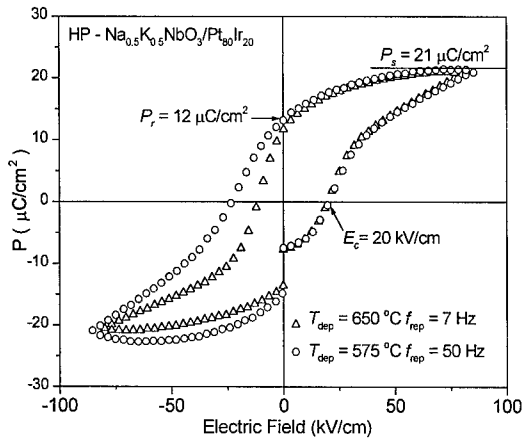
Figure 2. P - E hysteresis loops of HP-NKN/Pt films fabricated at different deposition temperatures T_{\text{dep}} , and laser repetition rates, f_{\text{rep}} , measured at room temperature. Symbols \Delta show the P - E loop for T_{\text{dep}} of 650^\circ\text{C} and f_{\text{rep}} of 7\text{ Hz} , while the symbol \circ corresponds to 575^\circ\text{C} and 50\text{Hz} .
