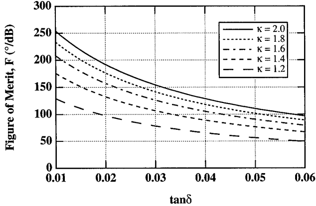
Fig. 5. Figure of merit vs. loss tangent for several values of tunability ( f = 30 GHz, R_s = 0.04 \Omega ).
