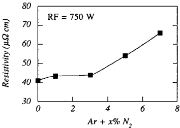
Figure 4. Variation of ρ with N 2 flow ratio.
