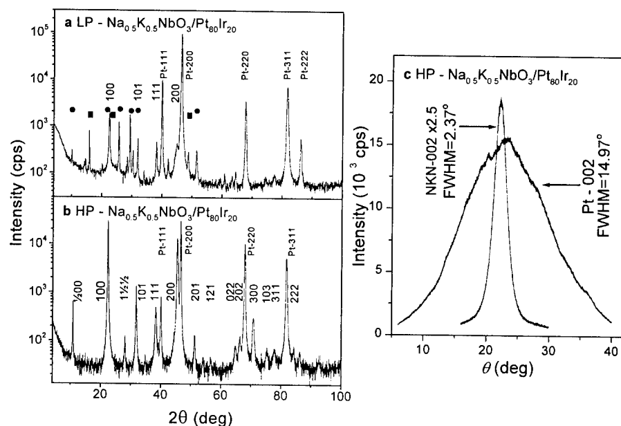
Figure 1. X-ray diffraction (XRD) scans in CuK_{\alpha} radiation for Na_{0.5}K_{0.5}NbO_3 films deposited on Pt_{80}Ir_{20} substrates: a - \theta -2 \theta scan for 0.47 \mu m thick NKN film deposited in 10 mTorr O_2 (LP-film) Symbol \bullet corresponds to K_2Nb_8O_{21} phase, while \blacksquare to K_2Nb_4O_{11} . b - \theta -2 \theta scan for 1.5 \mu m thick NKN film deposited in 400 mTorr O_2 (HP-film). hkl Bragg peaks indicate the Na_{0.5}K_{0.5}NbO_3 reflections. c - XRD rocking curves ( \omega -scans) of the NKN-002 and Pt-002 reflections from the same film shown in Fig. 1b.
