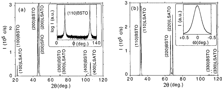
Fig.1. a) An x-ray ( \omega/2\theta , \text{CuK}_\alpha ) scan for a (100)SRO \parallel (100)BSTO \parallel (100)SRO heterostructure grown on (100)LSATO. The substrate plane was normal to the plane formed by incident and scattering x-ray beams during the measurement. * - denotes the (400)SRO x-ray peak. The insert shows a ( \phi , \text{CuK}_\alpha ) scan for the (110)BSTO x-ray reflection. b) The x-ray ( \omega/2\theta , \text{CuK}_\alpha ) scan measured for the same heterostructure as in (a) when the plane formed by incident and scattering x-ray beams was normal to the (110)BSTO. •- and :- (220) and (330)SRO x-ray peaks. The insert plots the rocking curve for the (200)BSTO x-ray reflection.
