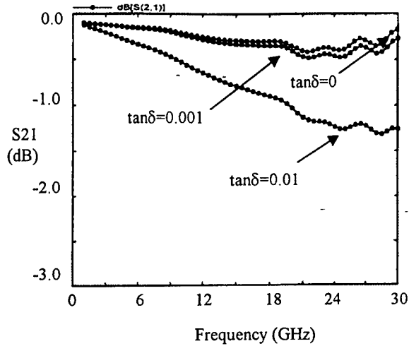
Figure 10. Simulated effect (using IE3D) of substrate loss tangent on insertion loss of a 1 cm long 50\ \Omega microstrip line terminated in a matched source and load on 0.25\ \text{mm}\ \text{LaAlO}_3 . The 2\ \mu\text{m} thick metal strip and ground plane had an electrical conductivity of 4.9 \times 10^7\ \text{S/m} .
