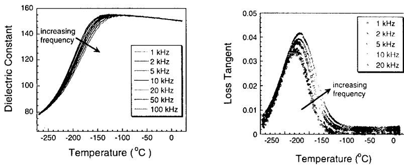
Figure 2: Low temperature relaxation in cubic BZN films.
