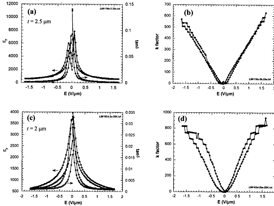
Fig. 8 Electric field dependence of (a) \epsilon_r , \tan\delta and (b) figure of merit k for a STO thin film at a temperature of 25 K. Data from another film at 25 K are shown in (c) and (d). The figure of merit is defined as k \equiv [\epsilon(0) - \epsilon(E)] / [\epsilon(0) \tan \delta(E)] . The data were measured at 10 kHz.
