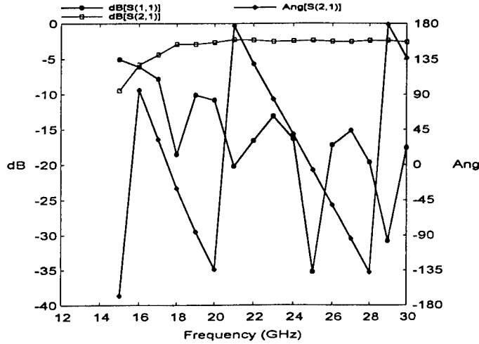
Figure 11. Modeled S-parameters for an 8-section coupled microstrip ferroelectric phase shifter on 0.3\ \text{mm}\ \text{MgO} with 400\ \text{nm}\ \text{Ba}_{0.60}\text{Sr}_{0.40}\text{TiO}_3 film. l=350\ \mu\text{m} , s=7.5\ \mu\text{m} and w=30\ \mu\text{m} . \epsilon_1=2500 , \tan\delta=0.05 , and \sigma=4.9 \times 10^7\ \text{S/m} for the 2.5\ \mu\text{m} metal layers.
