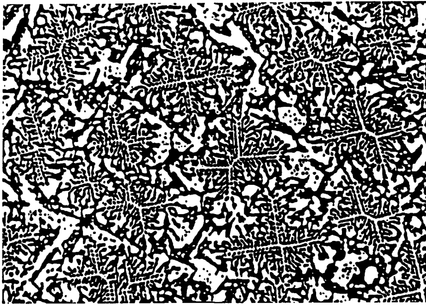
Figure 4 Micrograph of a transverse section of a unidirectionally solidified rod of mixture of magnetostrictive \text{CoFe}_2\text{O}_4 and piezoelectric \text{BaTiO}_3 , with an excess of \text{TiO}_2 (1.5 wt.%) (after Uchino, <14> 1986). <QA:6>
