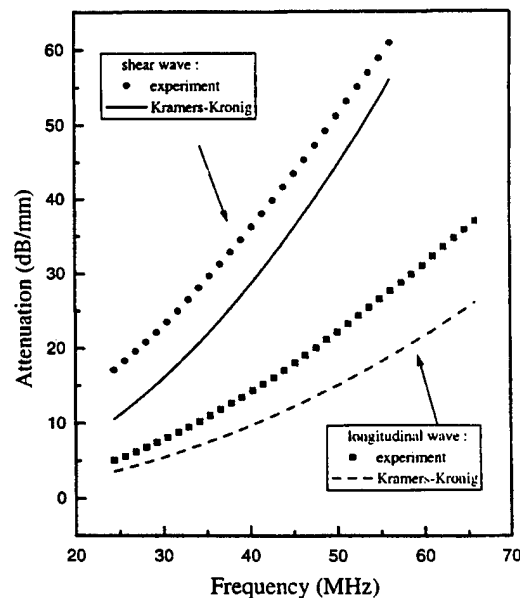
FIG. 8. The attenuation measured by experiment and derived by Kramers-Kronig relationship for a wave propagating in the x-z plane of a PZT sample. The longitudinal and shear velocities were fitted to linear curves: v_L = 4156.8 + 1.44e - 6 * f (Hz) and v_S = 1597 + 8.67e - 7 * f (Hz).
