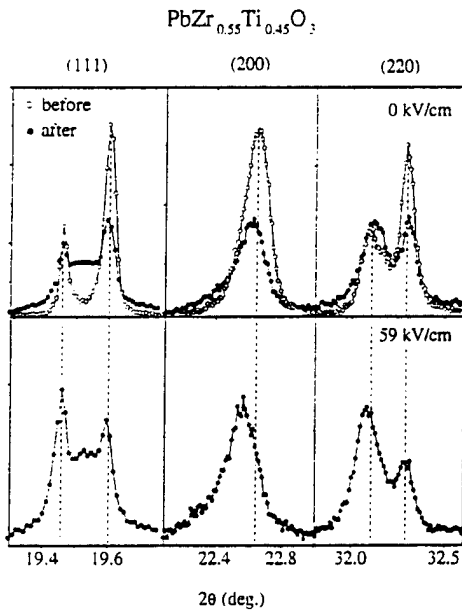
FIG. 3. (111), (200) and (220) pseudocubic reflections for PZT with x=0.45 measured on an unpoled sample (open circles) and on a similar sample after the application and removal of a field of 59 kV/cm at room temperature (solid circles) are plotted in the upper part of the figure. The scattered intensity at 2\theta = 19.52^\circ from the second sample corresponds to the (111) reflection from the silver electrode. Measurements on the latter sample under an electric field of 59 kV/cm applied in situ are plotted in the lower part of the figure.
