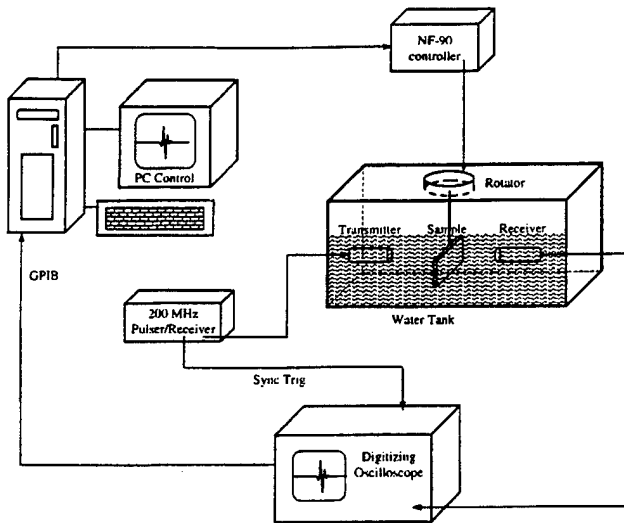
FIG. 3. Experiment setup.
