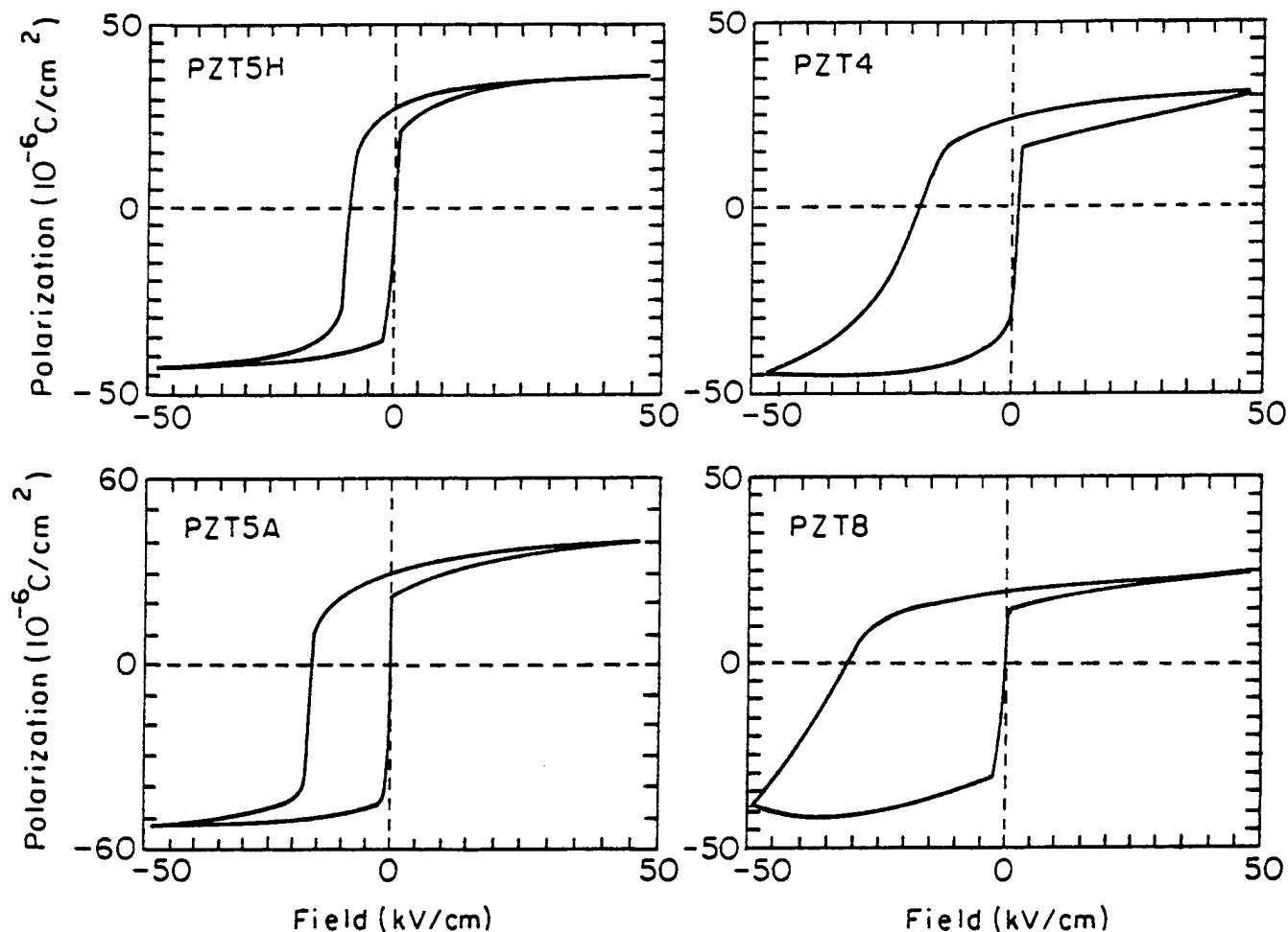
Fig. 1. The polarization hysteresis loops of aged PZT piezoceramics measured at 10 Hz.
