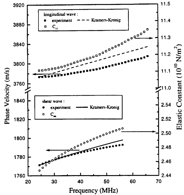
FIG. 7. The phase velocity dispersion measured by experiment and derived by Kramers-Kronig relationship for wave propagating in the x-y plane of a PZT sample and the corresponding elastic constants. The longitudinal and shear velocities were fitted to linear curves: v_L = 3744.4 + 1.00e - 6 * f (Hz) and v_S = 1762.5 + 5.47e - 7 * f (Hz).
