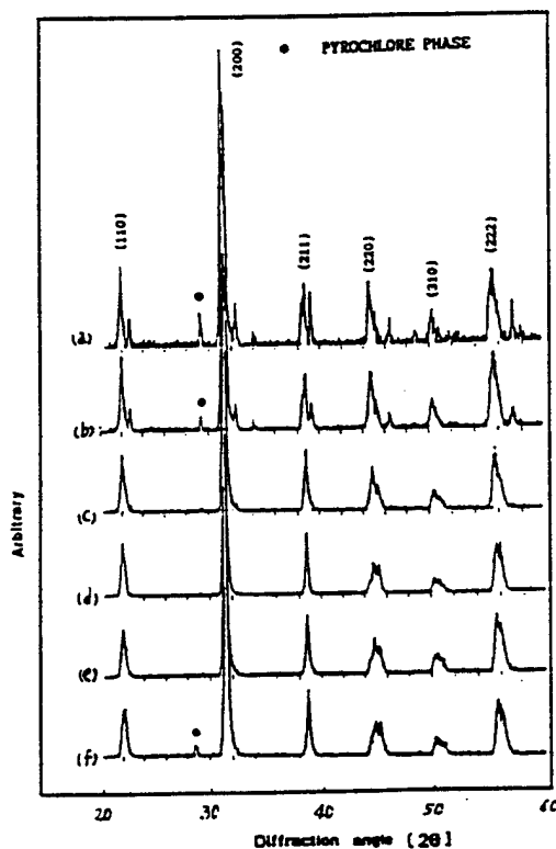
Fig. 1. X-ray diffraction patterns of 0.57PSN-0.43PT- x wt% Fe_2O_3 samples with (a) x = 0 , (b) x = 0.1 , (c) x = 0.3 , (d) x = 0.5 , (e) x = 0.7 and (f) x = 0.9 . The samples were calcined at 850°C for 2 h.
