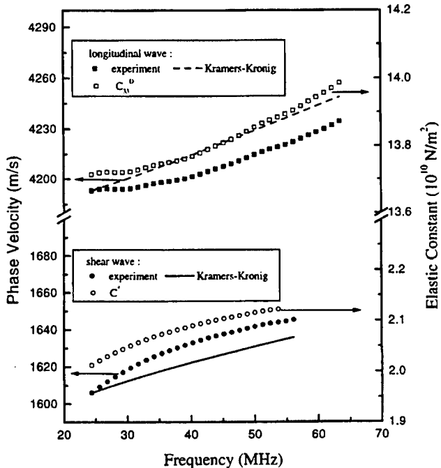
FIG. 6. The phase velocity dispersion measured by experiment and derived by Kramers-Kronig relationship for a wave propagating in the x-z plane of a PZT sample and the corresponding elastic constants.
