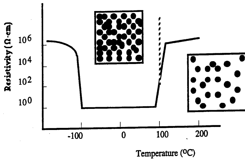
Figure 3 NTC-PTC effect observed in a \text{V}_2\text{O}_3 -epoxy composite (after Uchino, <14> 1986).
