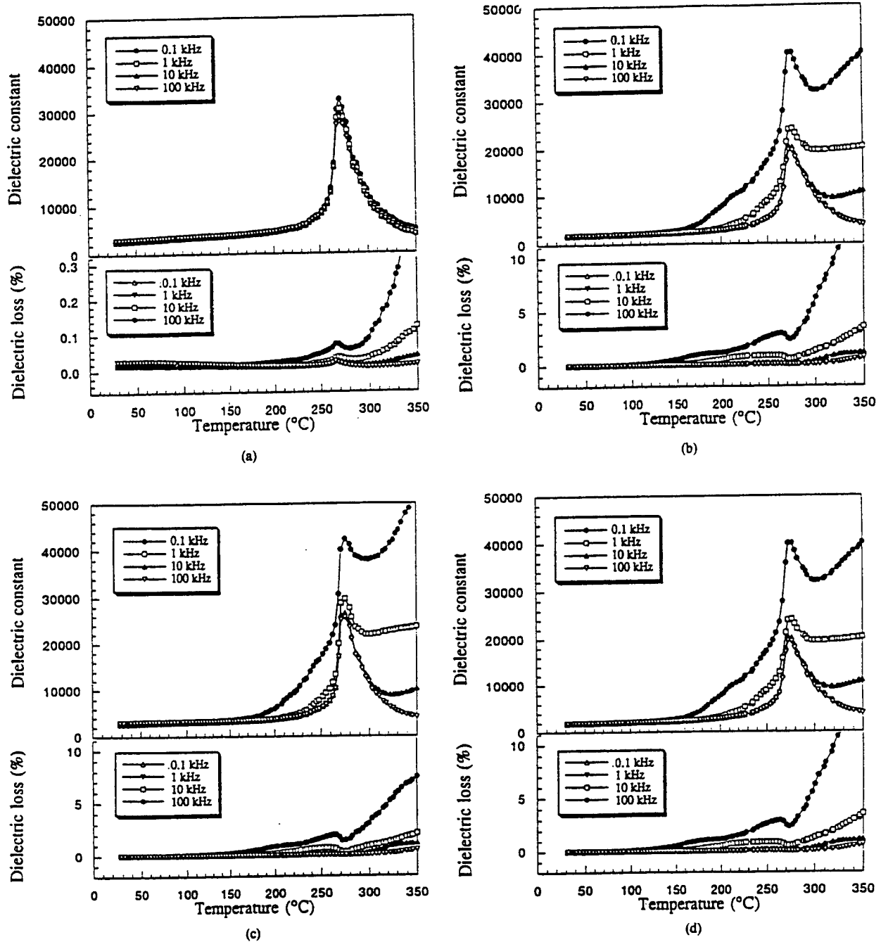
Fig. 3. Temperature dependence of the dielectric constant and the dielectric loss as a function of \text{Fe}_2\text{O}_3 content in 0.57\text{PSN}-0.43\text{PT}+x\text{ wt}\% \text{Fe}_2\text{O}_3 samples. Samples were measured while being heated to 350^\circ\text{C} . (a) x = 0 without \text{Fe}_2\text{O}_3 (b) x = 0.1 with \text{Fe}_2\text{O}_3 (c) x = 0.3 with \text{Fe}_2\text{O}_3 (d) x = 0.7 with \text{Fe}_2\text{O}_3
