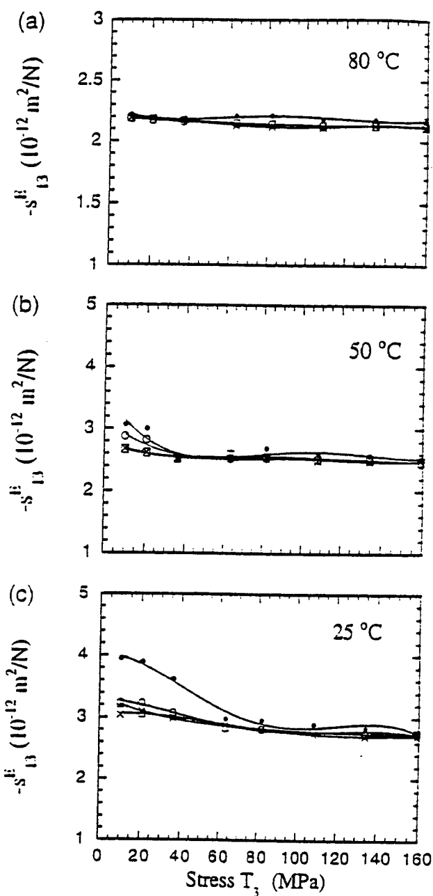
FIG. 7. The elastic compliance s_{13}^E as a function of the compressive T_3 at different temperatures: (a) 80 °C, (b) 50 °C, and (c) 25 °C; and dc electric bias fields: zero bias ( \times ), 1 kV/cm ( \square ), 3 kV/cm ( \circ ), and 5 kV/cm ( \bullet ).
