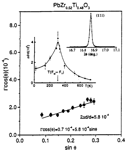
FIG. 2. The Williamson-Hall plot for PZT ( x=0.48 ) derived from the measured diffraction peak widths in the cubic phase ( T=736 K). Particle size and microstrain are estimated from a linear fit (solid line). The plot for the (111) reflection in the cubic phase demonstrates the excellent quality of the ceramic sample (peak width \sim 0.02^\circ ). The plot of \Delta d/d vs temperature is also shown as an inset.
