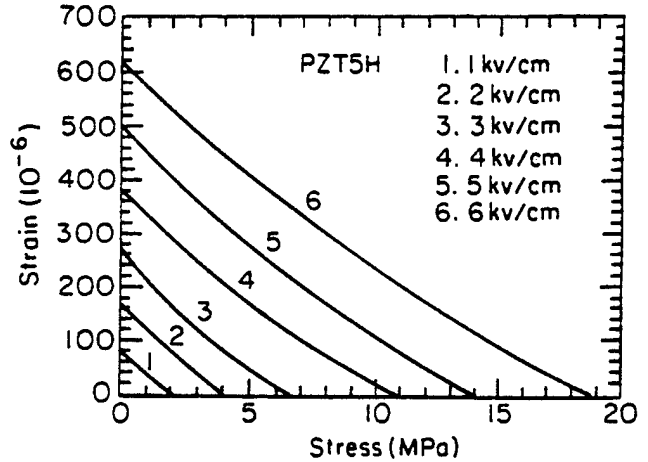
Fig. 11. Load curves of longitudinal strain versus T_3 for PZT-5H and PZT-8 piezoceramics. The applied DC electric fields are indicated.
