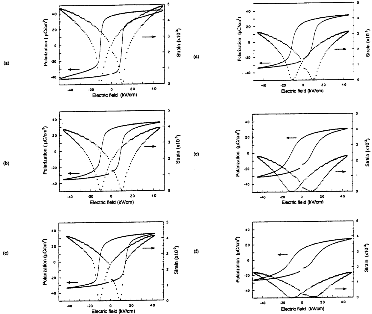
Fig. 4. P - E and S - E hysteresis loops (a) x = 0 , (b) x = 0.1 , (c) x = 0.3 , (d) x = 0.5 , (e) x = 0.7 and (f) x = 0.9 in 0.57\text{PSN}-0.43\text{PT}+x\text{ wt}\% \text{Fe}_2\text{O}_3 samples at room temperature and at 1.0 Hz.
