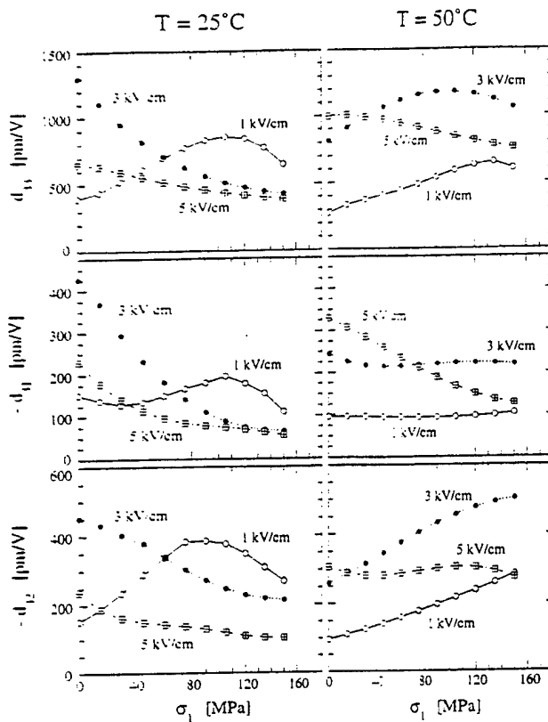
FIG. 2. Effective piezoelectric coefficients, d_{33} , d_{31} , and d_{32} , of 0.9PMN:0.1PT in the electric field biased state measured as a function of compressive stress, \sigma_1 , and dc bias at two temperatures: 25 °C (left column) and 50 °C (right column). The frequency of small ac probing field is 10 Hz. Symbols show experimental data, and the lines are drawn to guide the eye.
