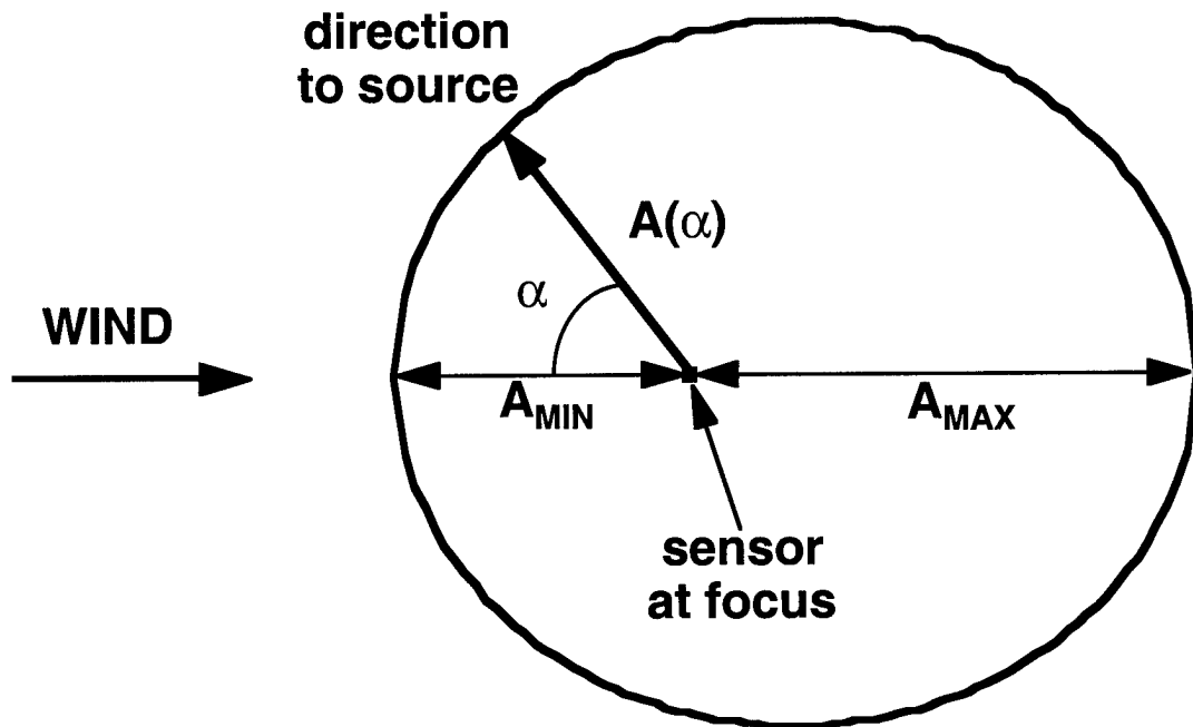
Figure A.2—Elliptical Interpolation Based on Wind Angle ( \alpha )
