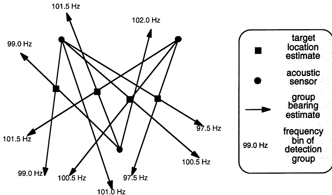
Figure A.3—Target Location by a Three-Sensor Network Using Triangulation
