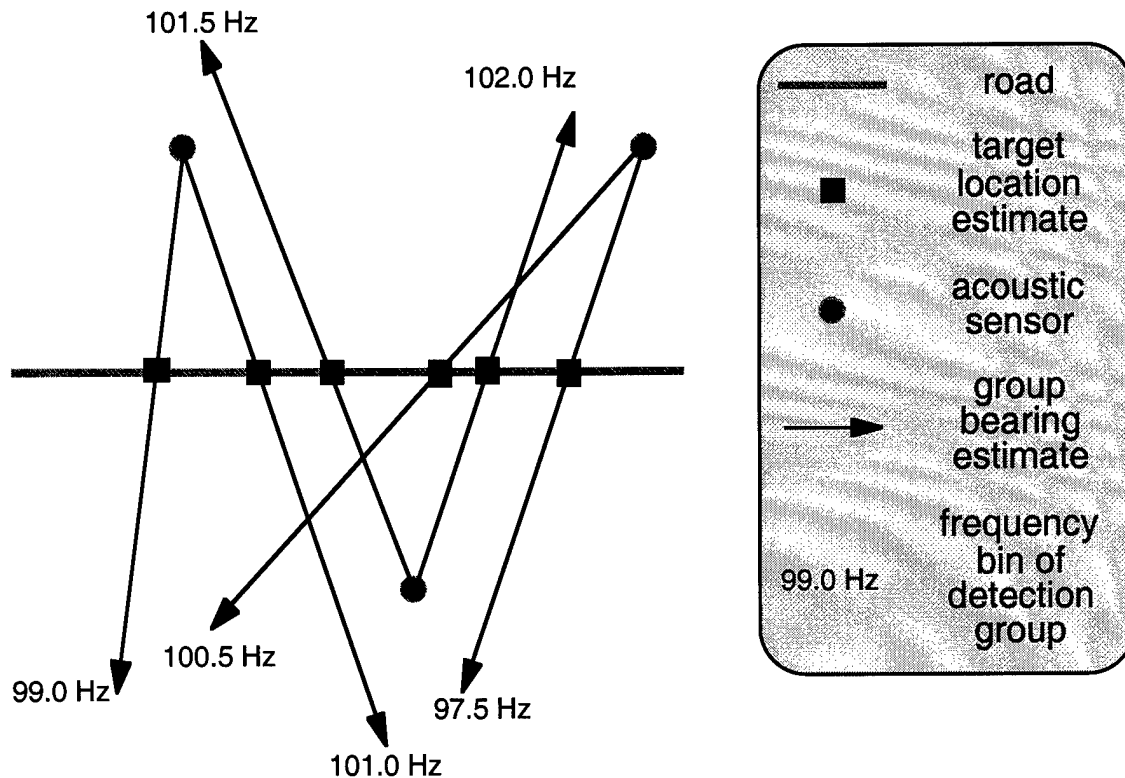
Figure A.5—Target Location by a Three-Sensor Network Using Road Fusion
