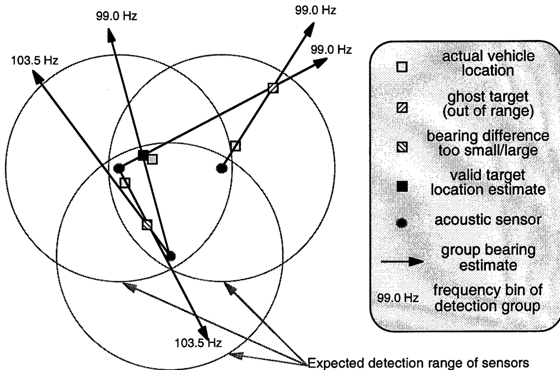
Figure A.4—Elimination of Potential Triangulation Points to Avoid Ghost Targets and Reduce Geometrical Location Errors
