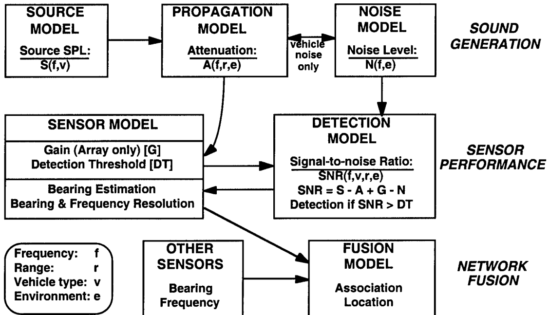
Figure A.1—Framework for Acoustic Sensor Network Model
