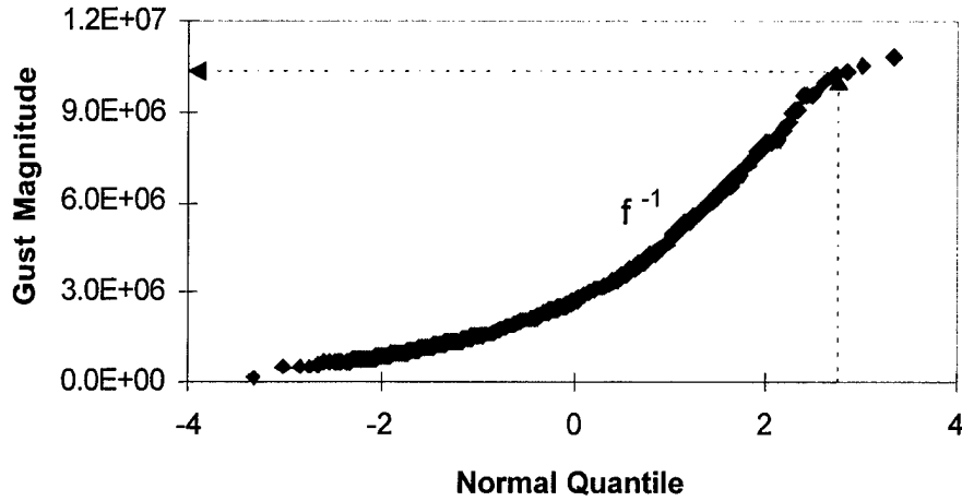
Figure 5. Nonparametric procedure for tolerance bounds. K-value for 0.997/0.90 normal tolerance interval is 2.83 for sample of 1131. From the figure, this corresponds to 1.05e+07 for a 0.997/0.90 tolerance bound for the gust loads data shown. This can be converted to k-value by using the sample mean and standard deviation of the gust.
