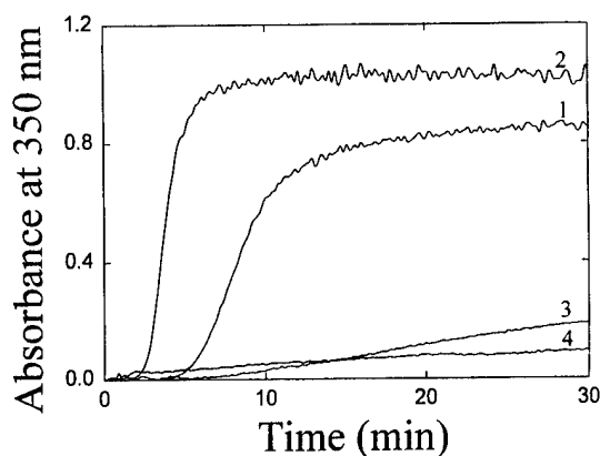
FIGURE 9: Assembly of \alpha -tubulin isoforms in the presence of glycerol and magnesium. Aliquots of tubulin fractions (1 mg/mL) in buffer A containing 16 mM \text{MgCl}_2 and 4 M glycerol were incubated at 37 °C, and the assembly was studied by monitoring the turbidity of the samples at 350 nm. Different curves are as follows: curve 1, PC-tubulin; curve 2, fraction A; curve 3, fraction B; curve 4, fraction C.
