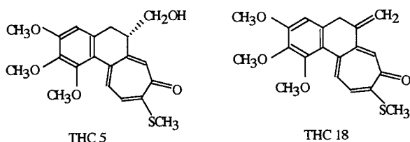
FIG. 1. Chemical structures of the thicolchicine analogs.
