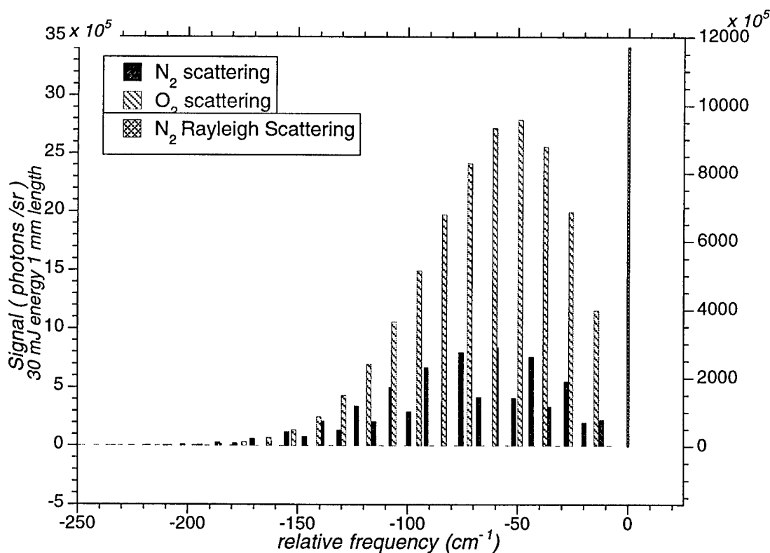
Figure 3: Rotational Raman scattering signal for \text{N}_2 and \text{O}_2 each at STP (left axis) compared with \text{N}_2 Rayleigh scattering signal (right axis)
