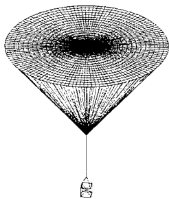
G-12 canopy "cut pattern" initial structural model geometry
