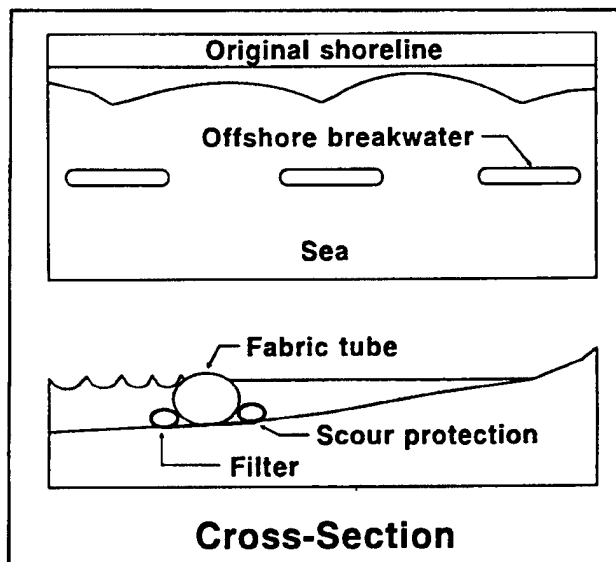
Figure 8. Offshore breakwater
