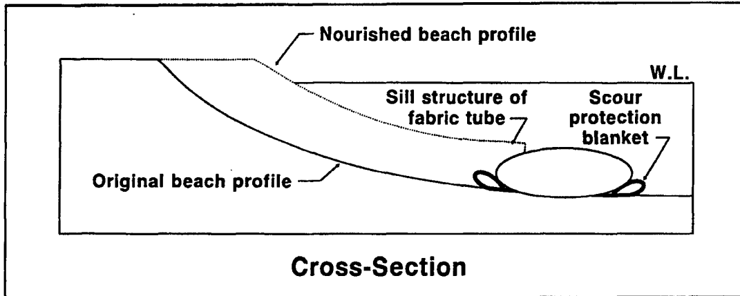
Figure 9. Sill structure
