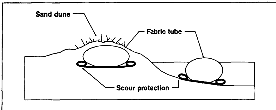
Figure 10. Sand dune
