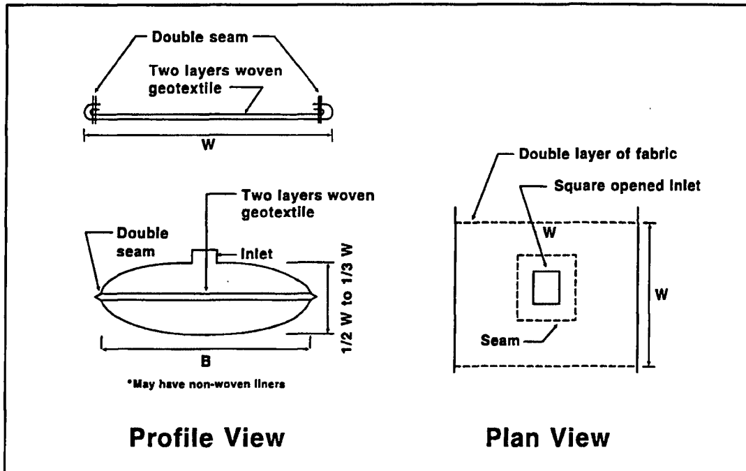
Figure 1. GeoTube construction
