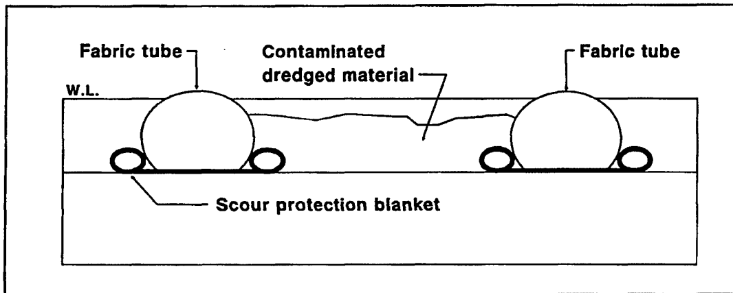
Figure 6. Containment dike
