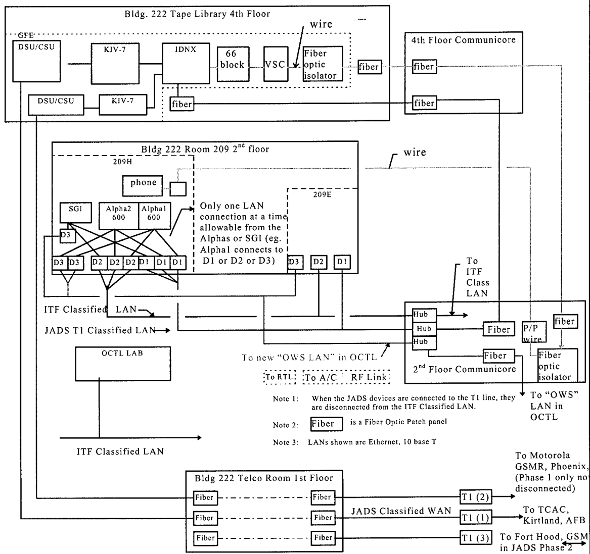
Figure 0-1 - JADS Communications Connections In Northrop Grumman ITF
