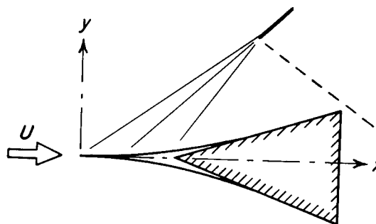
Sketch (c).- Steady flow past a smoothed wedge.
