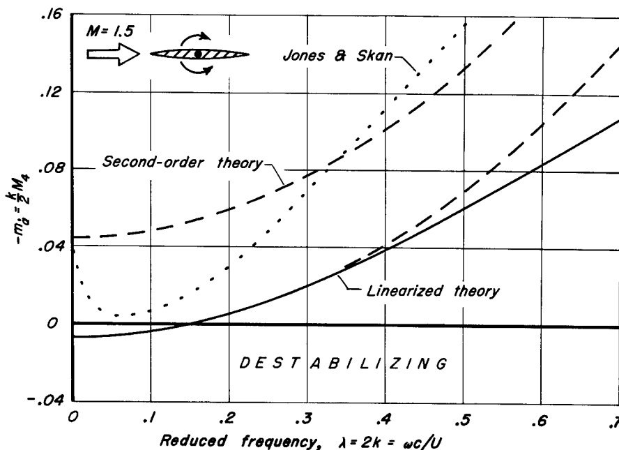
Sketch (1).- Effect of frequency upon damping moment coefficient for 5-percent-thick biconvex airfoil pivoted at midchord.
