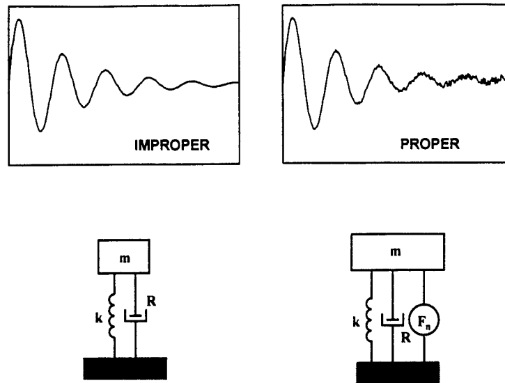
Figure 2.2. Damped mass-spring oscillator with an impulsive input. The system on the left is unrealizable; its amplitude decays to arbitrarily small values with sufficient time. The system on the right decays into the background of molecular-vibration induced fluctuations.
