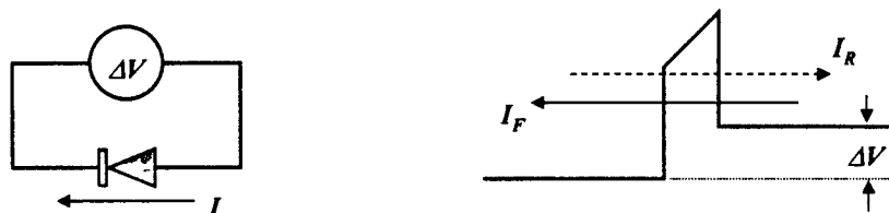
Figure 3.1. Current flow through a potential barrier. On the left, a voltage is applied to a semiconductor diode. The schematic representation of the potential barrier associated with the semiconductor junction and the forward and reverse currents is shown on the right.
