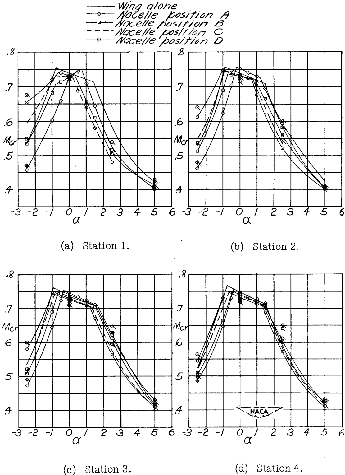
Figure 31.- Variation of critical Mach number with angle of attack for the wing with four horizontal nacelle positions. Untailed symbols refer to points extrapolated from M = 0.4 results.
