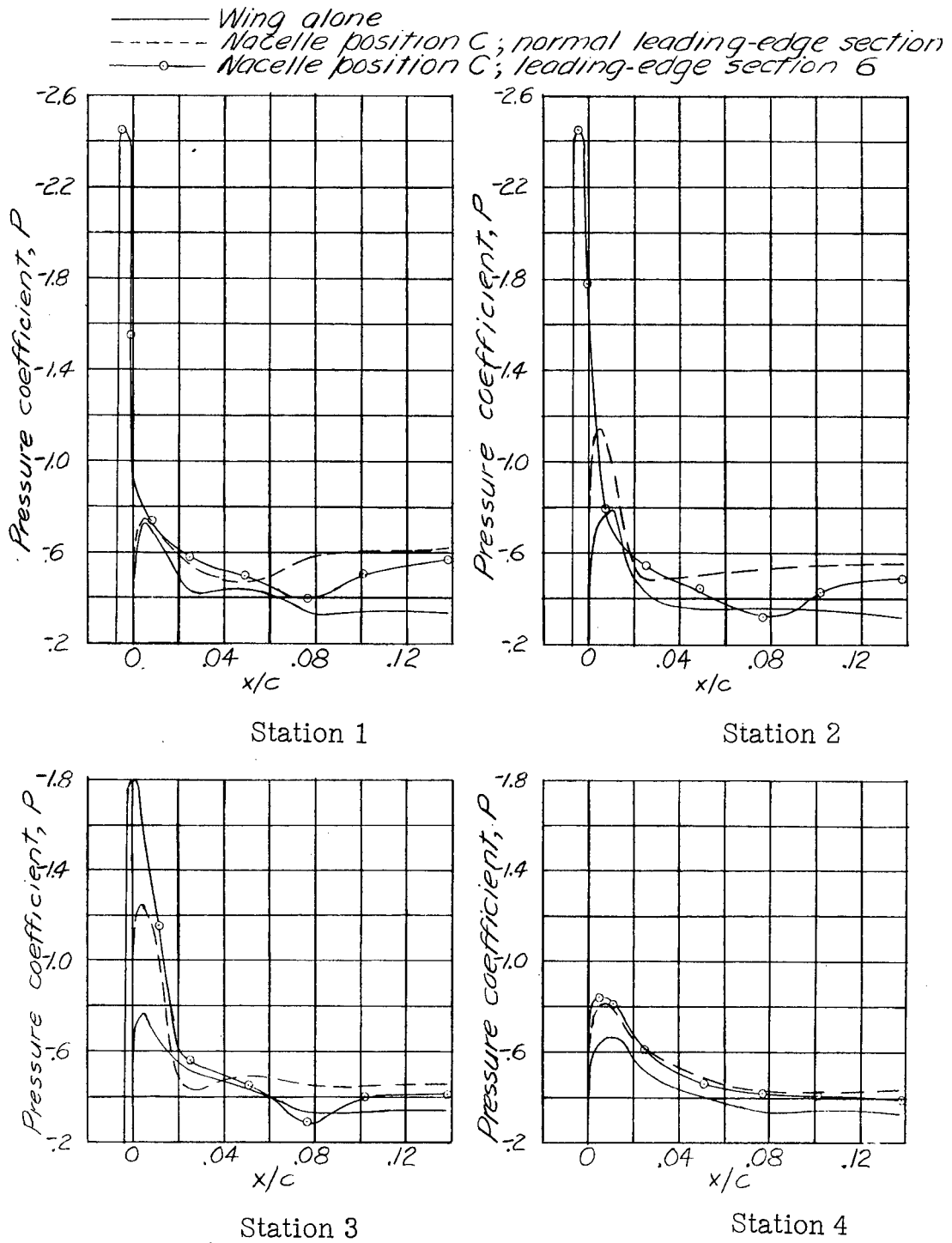
(c) Lower surface; \alpha = -1.5^\circ .
