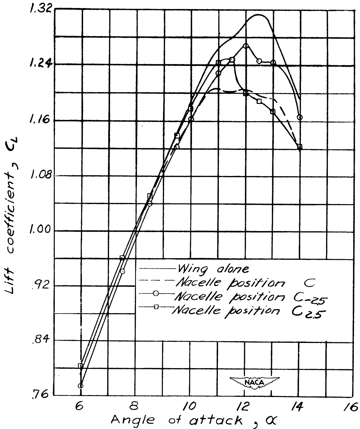
Figure 41.- Variation of lift coefficient with angle of attack for three angular nacelle positions. M = 0.2 . (Second series of tests.)
