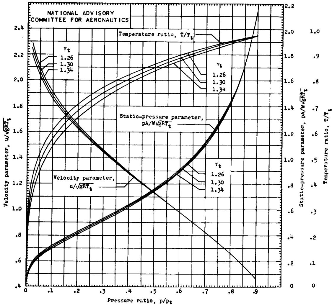
(b) Variable specific heats.
