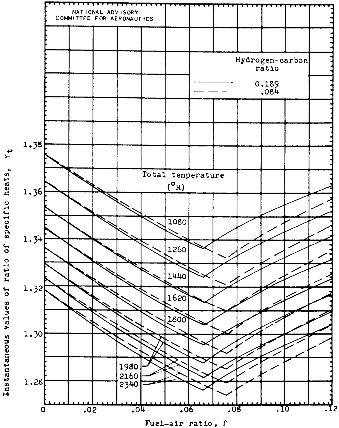
Figure 4. - Instantaneous values of ratio of specific heats \gamma_t for combustion gas. (Replotted from reference 1.)
