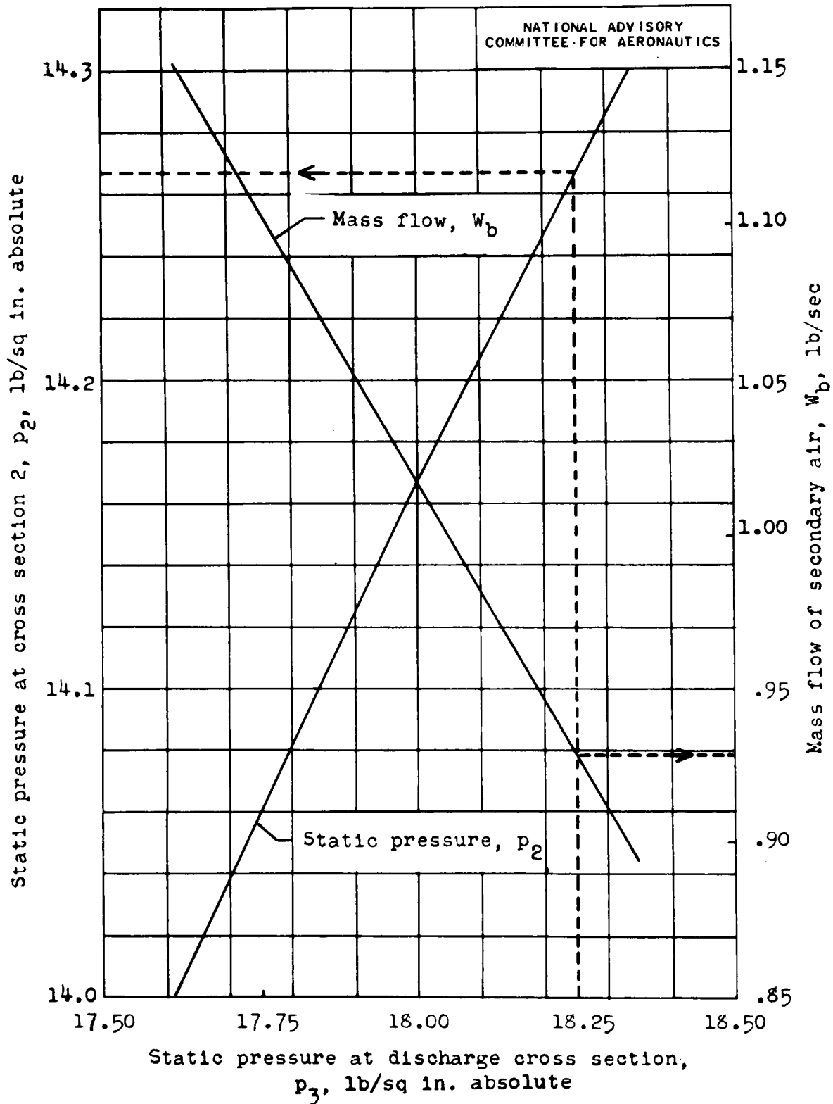
Figure 9. - Effect of static pressure at discharge cross section p_3 on static pressure p_2 at cross section 2 and mass flow of secondary air W_b for jet pump.
