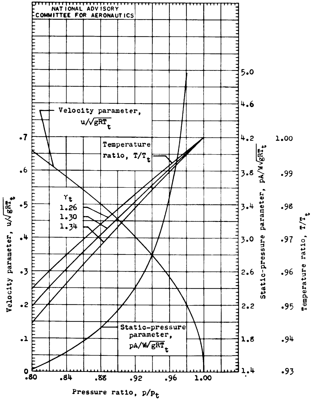
(b) Concluded. Variable specific heats.
