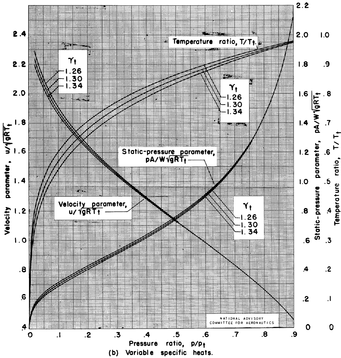
Figure 3.- Continued. Relations between flow parameters and pressure ratio.
