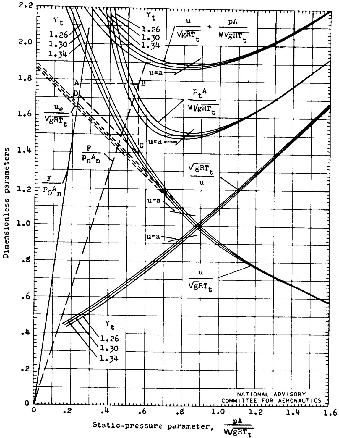
Figure 6. - Use of one-dimensional flow chart to determine total temperature of fluid from jet thrust.
