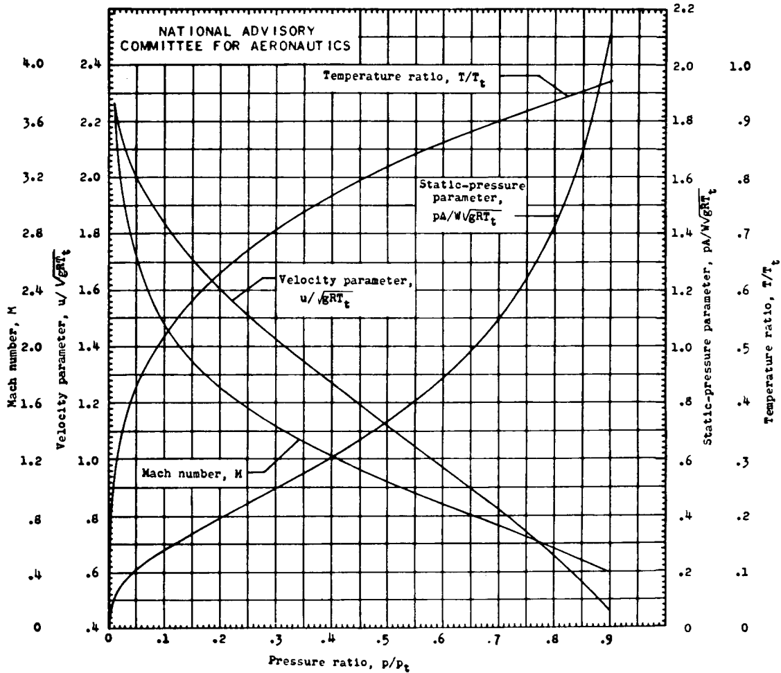
(a) Constant ratio of specific heats; \gamma, 1.40 .
