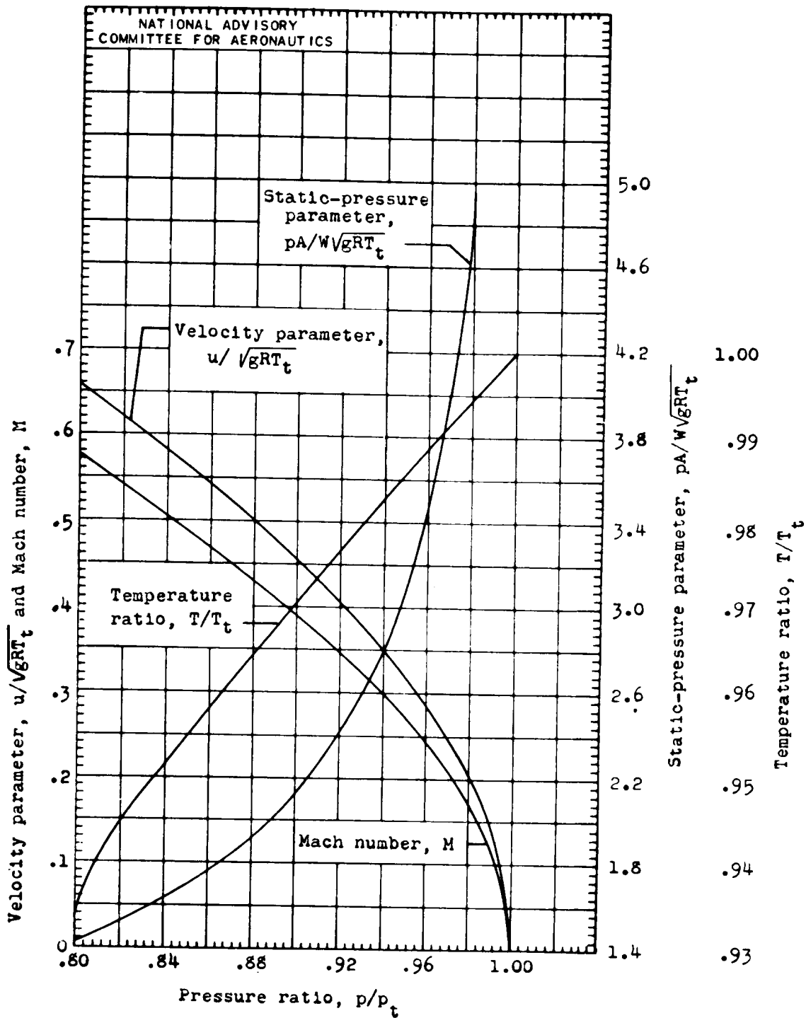
(a) Concluded. Constant ratio of specific heats; \gamma , 1.40.
