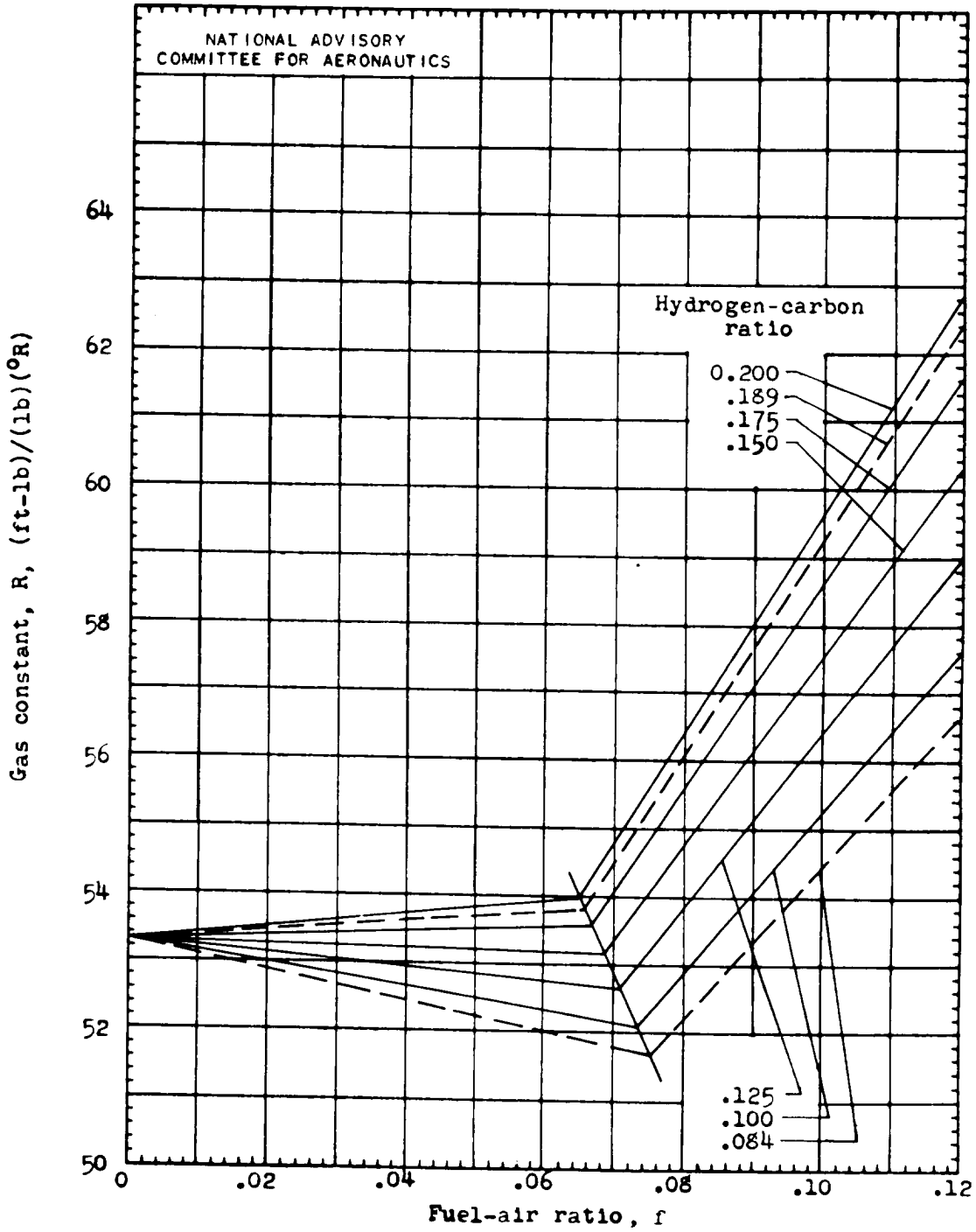
Figure 5. - Gas constant of combustion gas. (Replotted from reference 1.)
