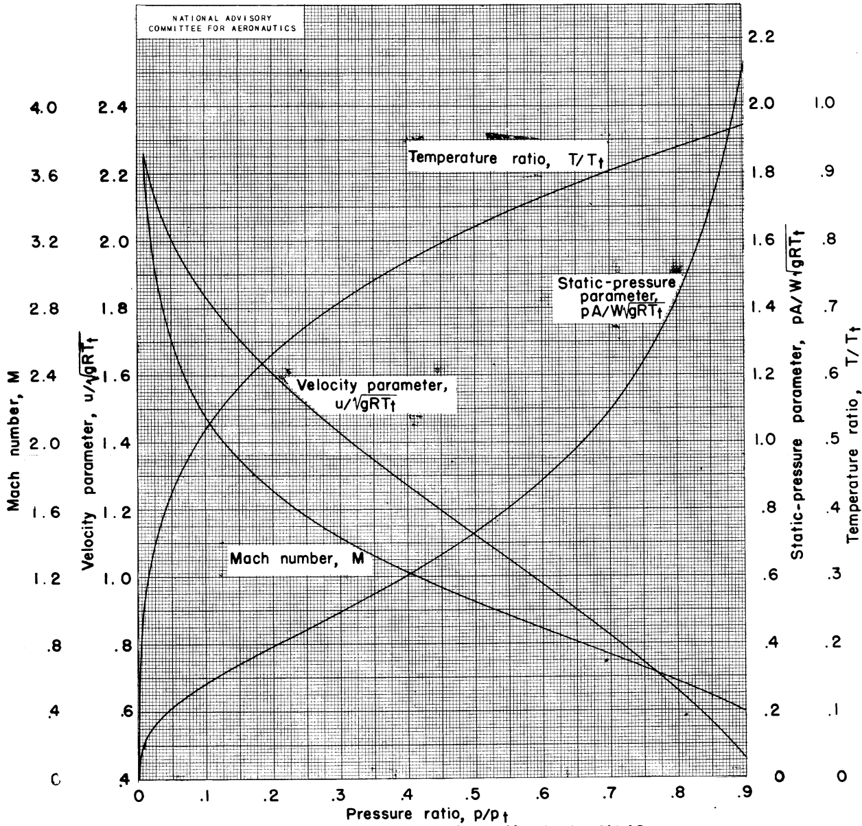
Figure 3. - Relations between flow parameters and pressure ratio.
