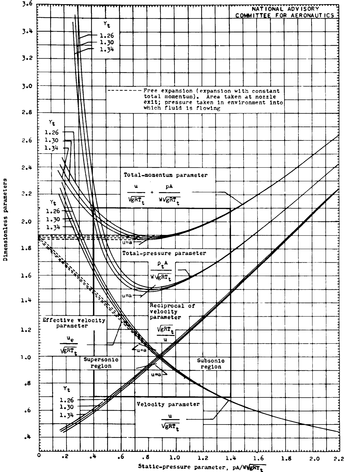
(b) Variable specific heats for range of static-pressure parameter from 0 to 2.2. Over-all plot; enclosed area enlarged in figure 2(b) concluded.
