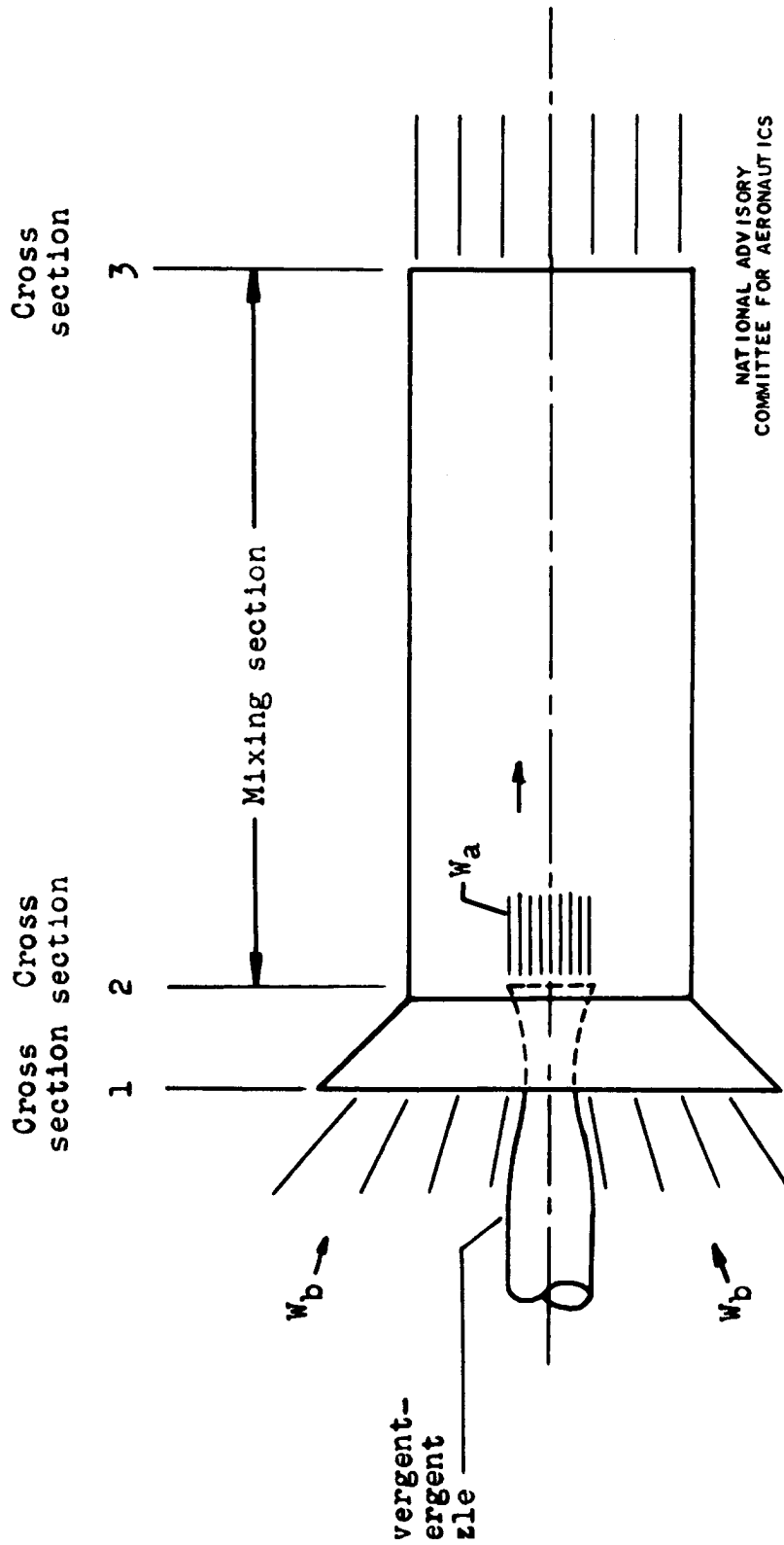
Figure 8. - Diagrammatic sketch of jet pump.
