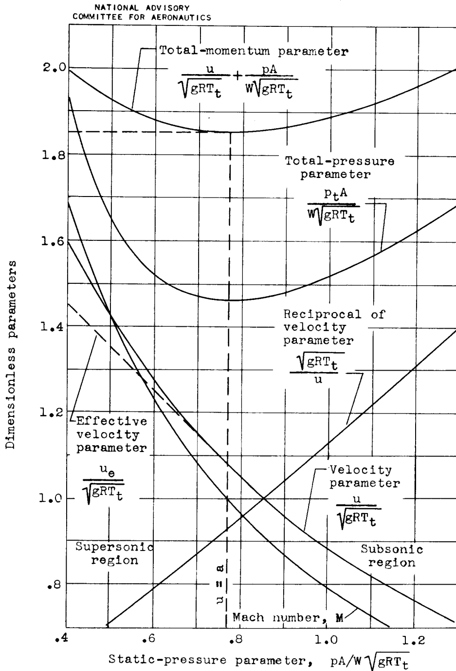
(a) Concluded. Constant ratio of specific heats of 1.40 for range of static-pressure parameter from 0 to 2.2. Enlargement of area shown in figure 2(a).
