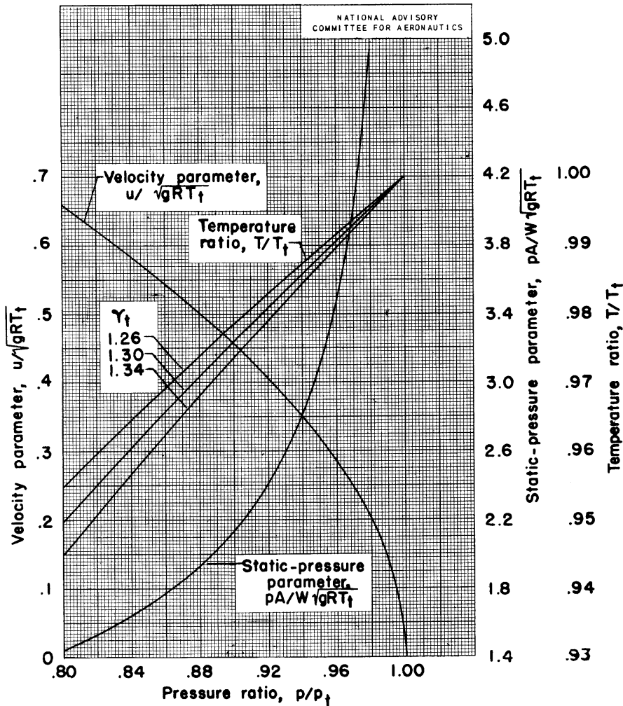
Figure 3. - Concluded. Relations between flow parameters and pressure ratio.
