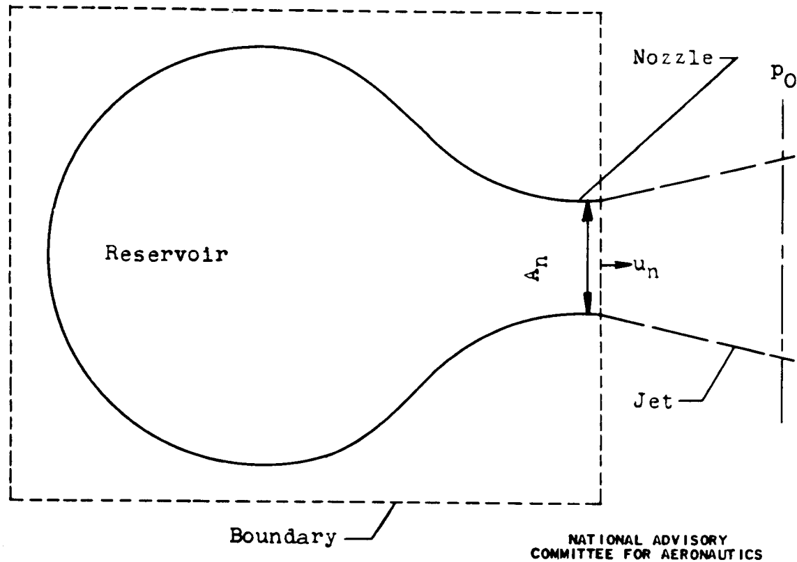
Figure 1. - Free expansion of compressible fluid from nozzle.
