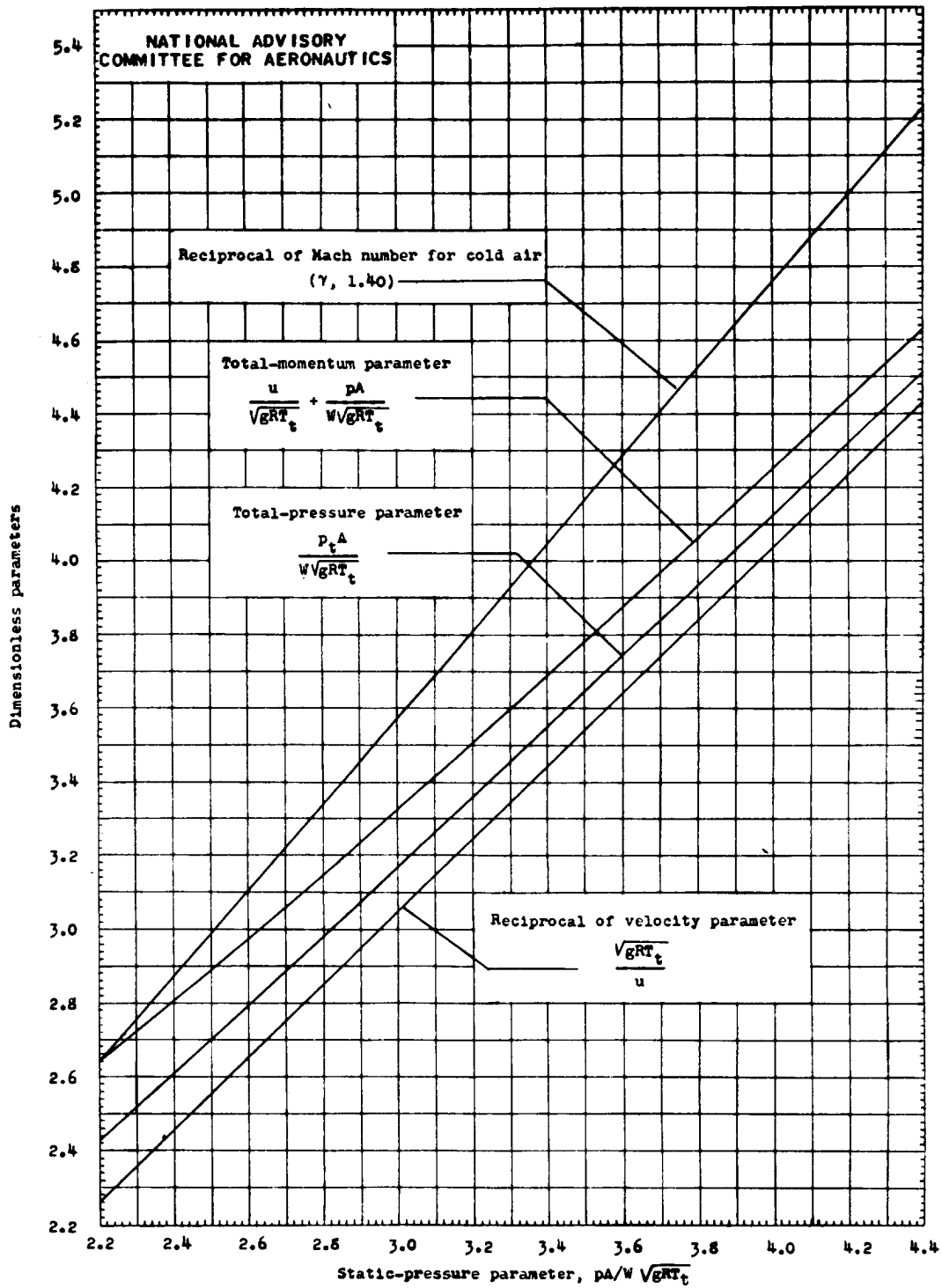
(c) Variable specific heats for range of static-pressure parameter from 2.2 to 4.4. On this figure the curves of total-momentum parameter, total-pressure parameter, and reciprocal of velocity parameter are applicable for all values of \gamma_t between 1.26 and 1.40.
