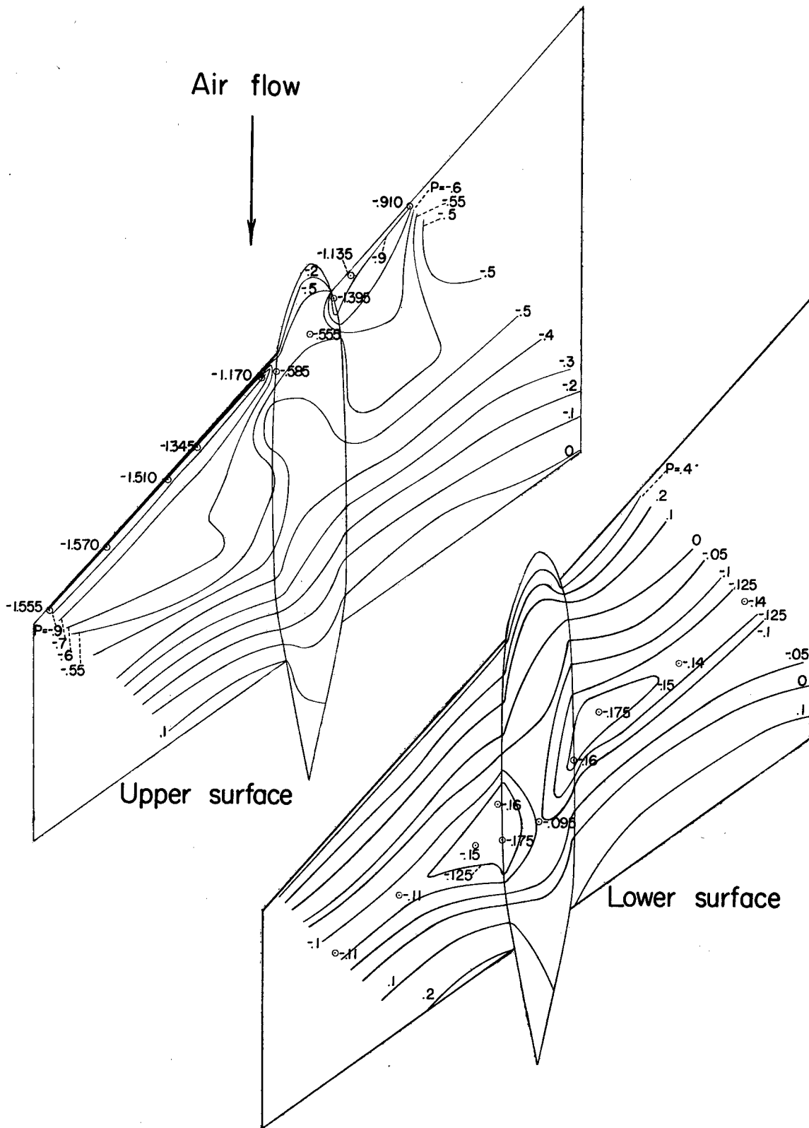
Figure 52.—Pressure contours for the wing-nacelle combination \Lambda=45^\circ ; C_L=0.40 ; M=0.61 .
