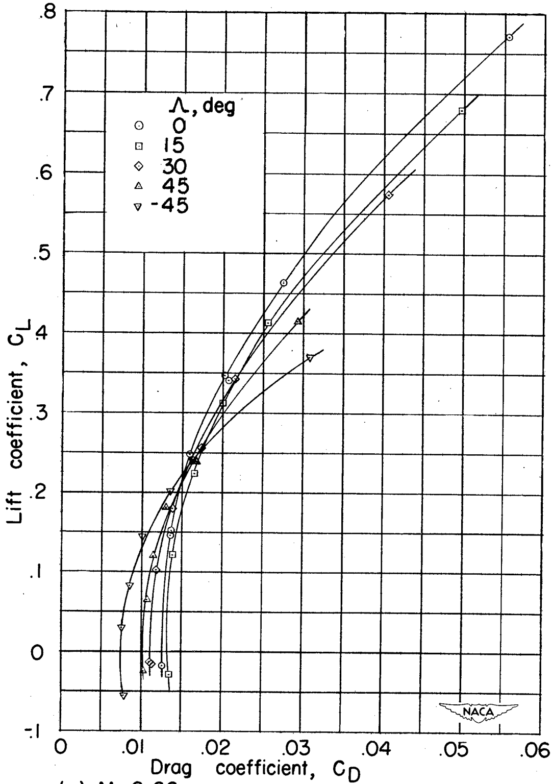
(g) M=0.66 . Figure 17.— Continued.
