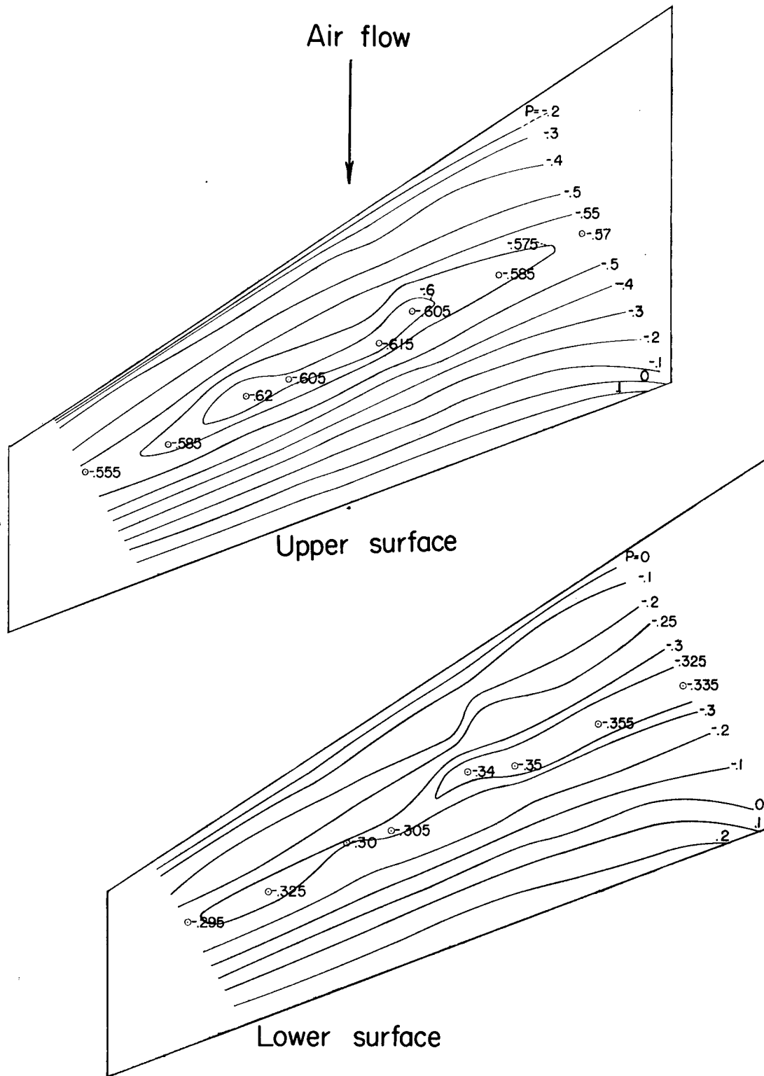
Figure 35.—Pressure contours for the wing alone. \Lambda = 30^\circ ; C_L = 0.20 ; M = 0.61 .
