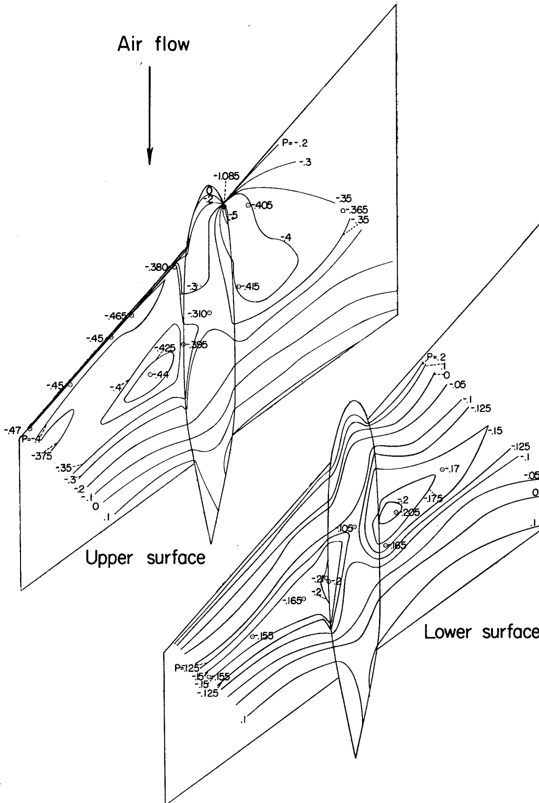
Figure 47.—Pressure contours for the wing-nacelle combination.
