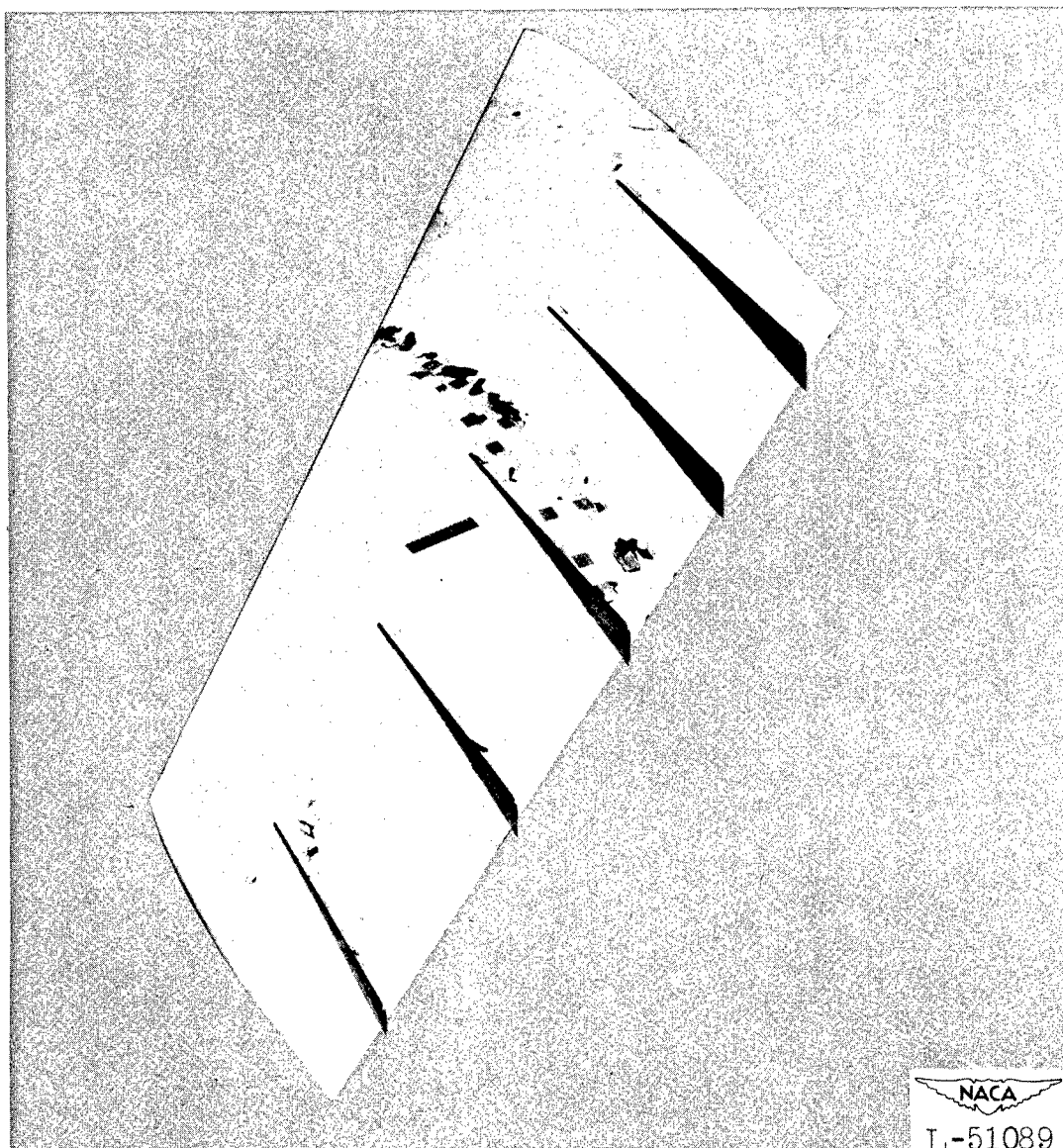
Figure 7.- Wing at 45° sweepback with vertical plates installed on upper surface.
