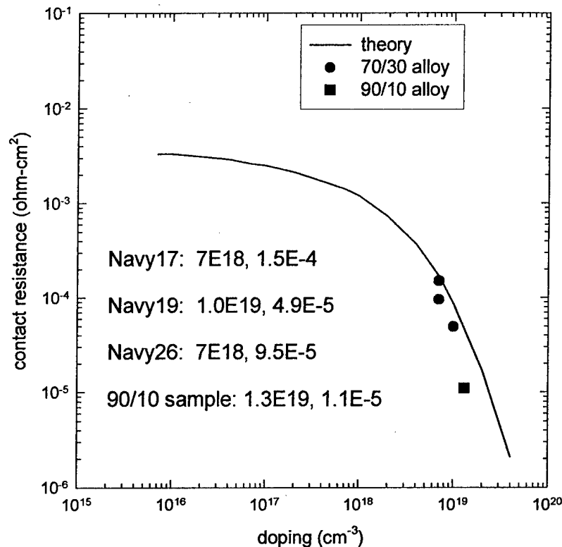
Figure 2. Theoretical curve of specific contact resistance verses doping for p-type SiC along with a typical (best case) 90/10 and three 70/30 Al-Ti alloy results.
