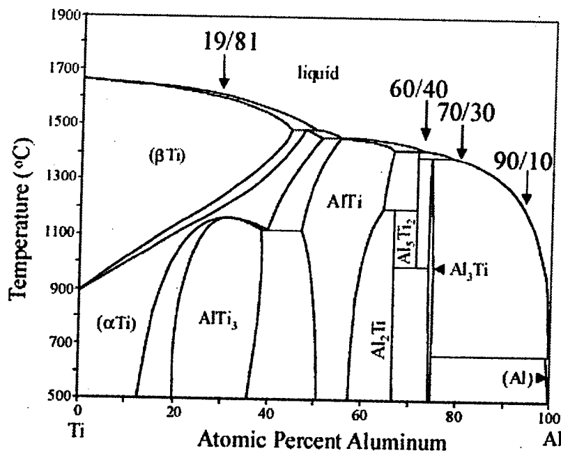
Figure 1. Al-Ti binary phase diagram.
