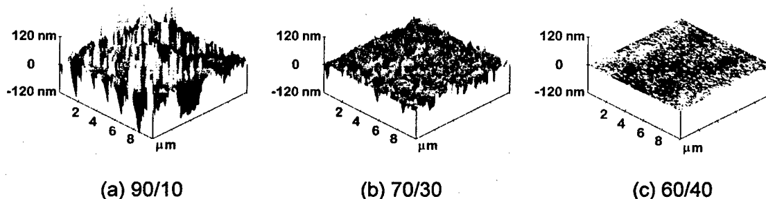
Figure 4. AFM image of the SiC surface revealed after the annealed (a) 90/10, (b) 70/30, and (c) 60/40 contacts were etched away. All samples were annealed at 1000 °C for 2 minutes in vacuum.
