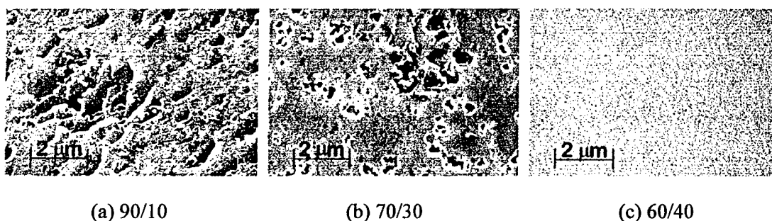
Figure 3. SEM image of the SiC surface revealed after the annealed (a) 90/10, (b) 70/30, and (c) 60/40 contacts were etched away. All samples were annealed at 1000 °C for 2 minutes in vacuum.
