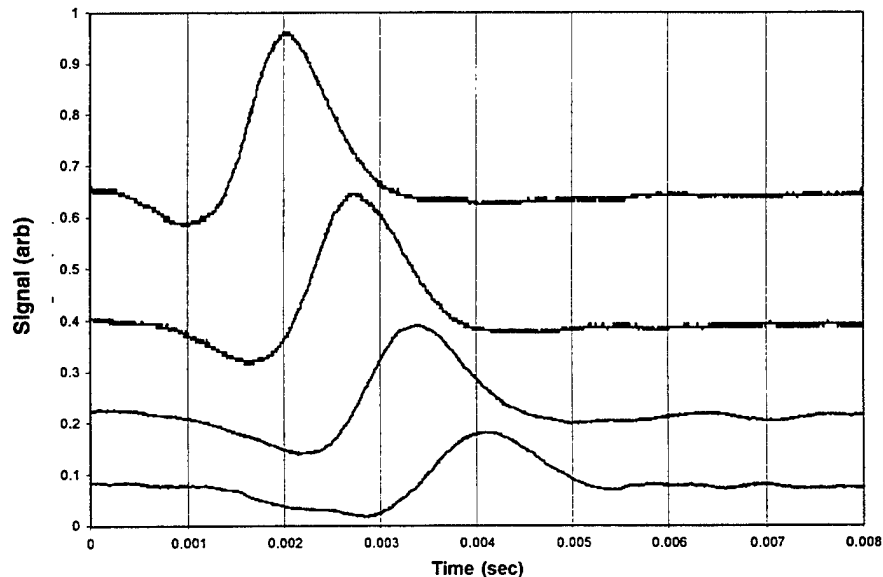
Figure 3-1. Observed impact-induced transient strain signals from one Bragg sensor. Impacts from top to bottom are at distances of 12.5, 25, 37.5, and 50 cm from the sensor.
