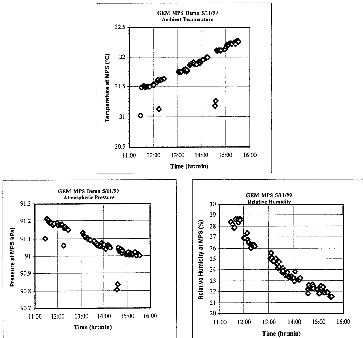
Figure 6-9. MPS ambient temperature, pressure, and relative humidity during impact testing at AFRL/EAFB rocket laboratory.
