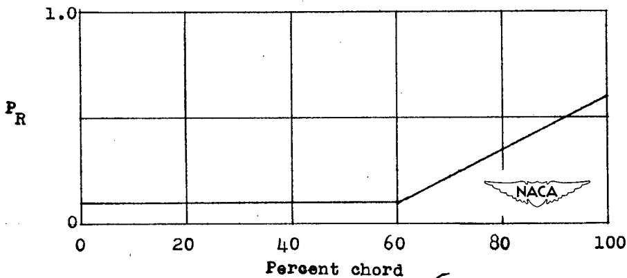
(c) Load distribution of the NACA \left. \begin{matrix} a = 1.0, & c_{l_1} = 0.6 \\ a = 0.6, & c_{l_1} = -0.4 \end{matrix} \right\} mean line (formed by superposition of the load distributions of the NACA a = 1.0 , c_{l_1} = 0.6 and NACA a = 0.6 , c_{l_1} = -0.4 mean lines).
