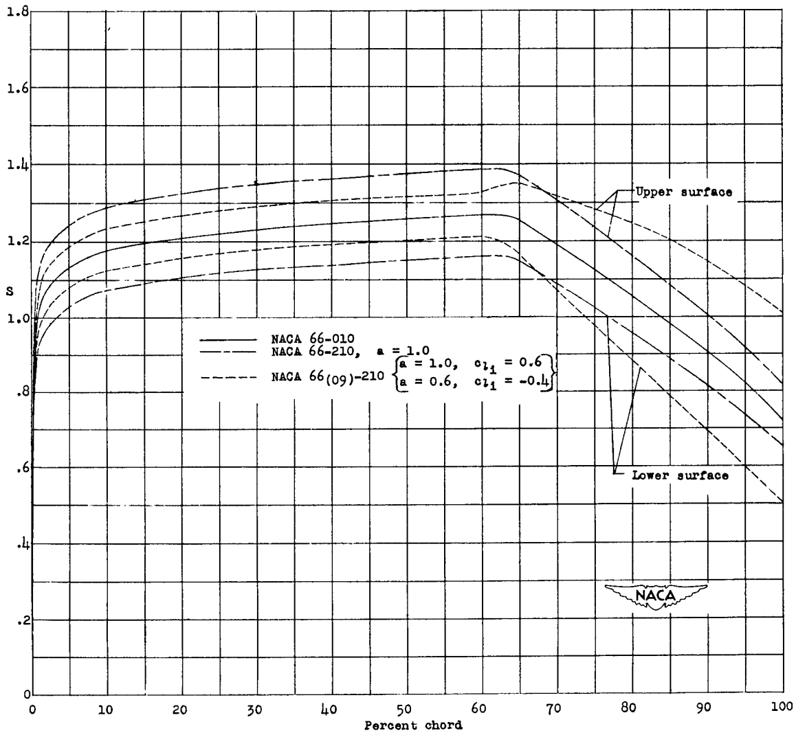
Figure 2.- Comparison of theoretical pressure distributions of several airfoils. at their design lift coefficient.
