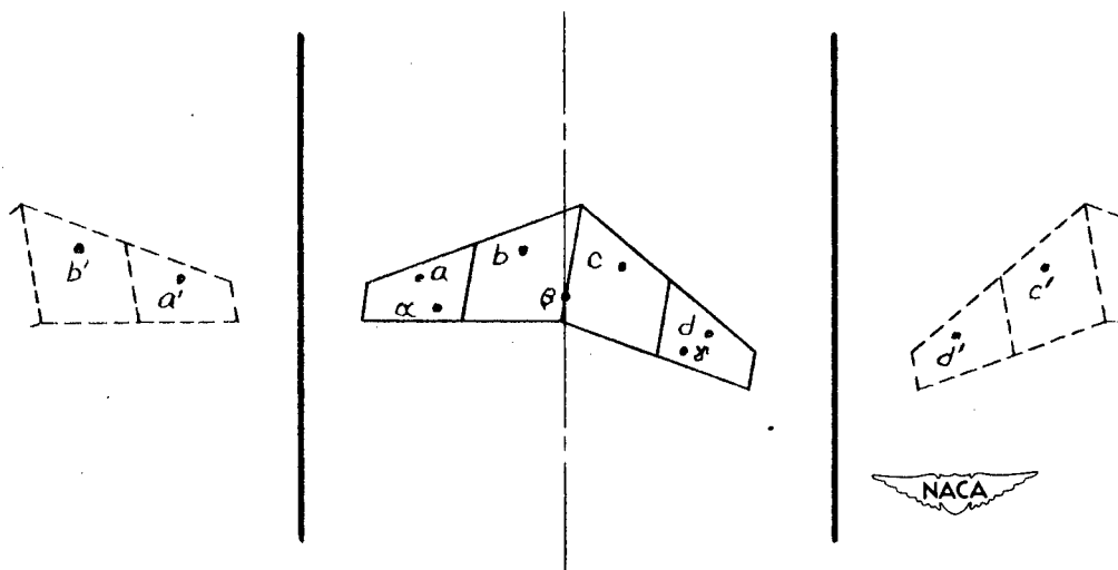
Figure 8.- Sketch used with charts A and B for determining tunnel-induced upwash angles. Sketch shows points a , b , c , and d where lift is assumed to be concentrated, the nearest images a' , b' , c' , and d' , and points \alpha , \beta , and \gamma where the tunnel-induced upwash angles are to be determined.
