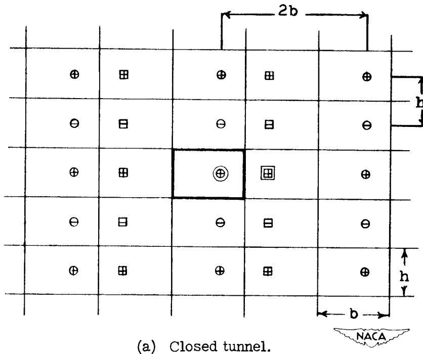
Figure 2.- Image configurations for doublet lines in rectangular tunnels. Doublet in tunnel is indicated by double circle; nearest lateral image is indicated by double square.
