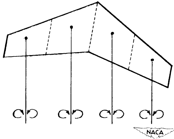
Figure 1.- Field of a lifting wing represented as the field of four doublet lines extending downstream from four points where the lift is assumed to be concentrated.
