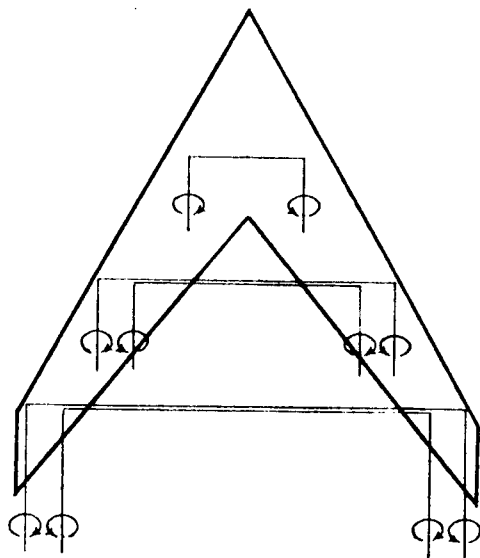
(a) Approximation by horseshoe vortices of 0^\circ sweep.
