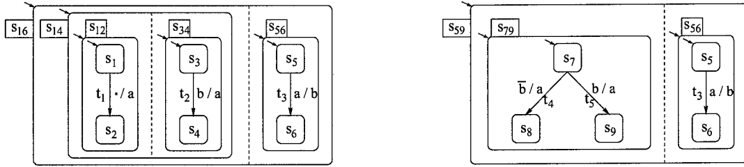
FIG. 2.1. Two example Statecharts
