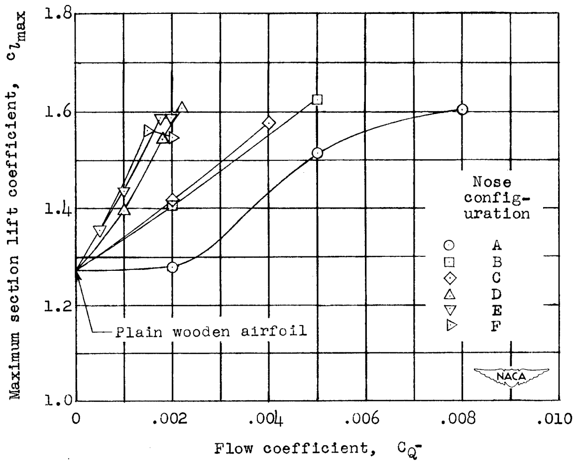
Figure 4.- Variation of maximum section lift coefficient with flow coefficient for the NACA 64 1 A212 airfoil with permeable nose. R \approx 1.5 \times 10^6 .
