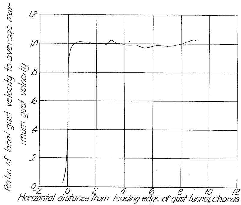
(a) 45° sweptback-wing model.
