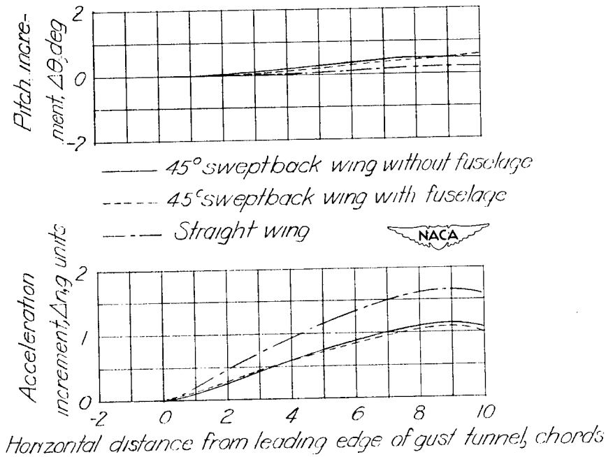
(b) Gust with 9-chord gradient distance. (Computed from experimental data for sharp-edge gust.) Figure 8.— History of events in test gusts.
