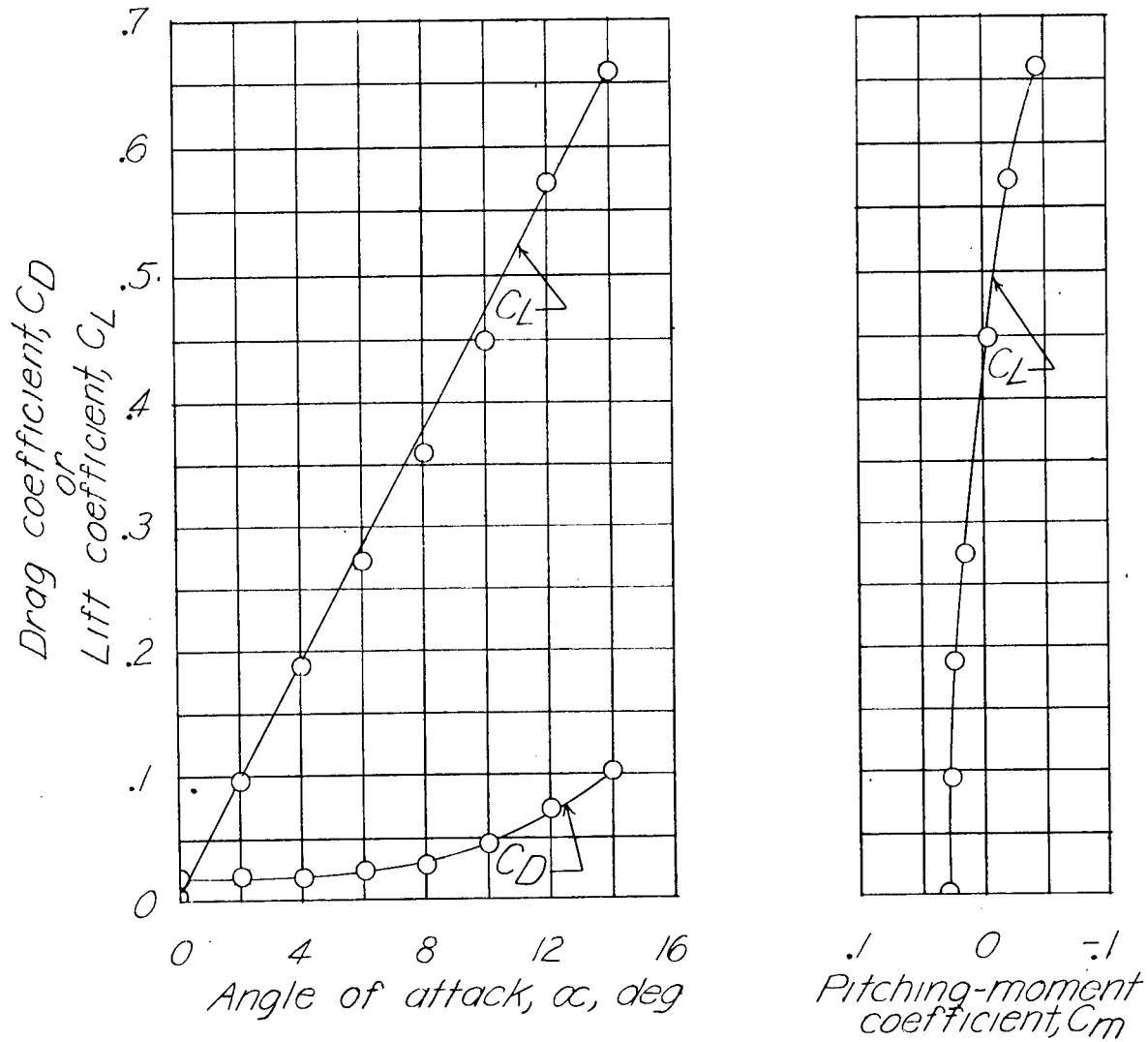
(b) 45° sweptback-wing model. Figure 6.- Concluded.
