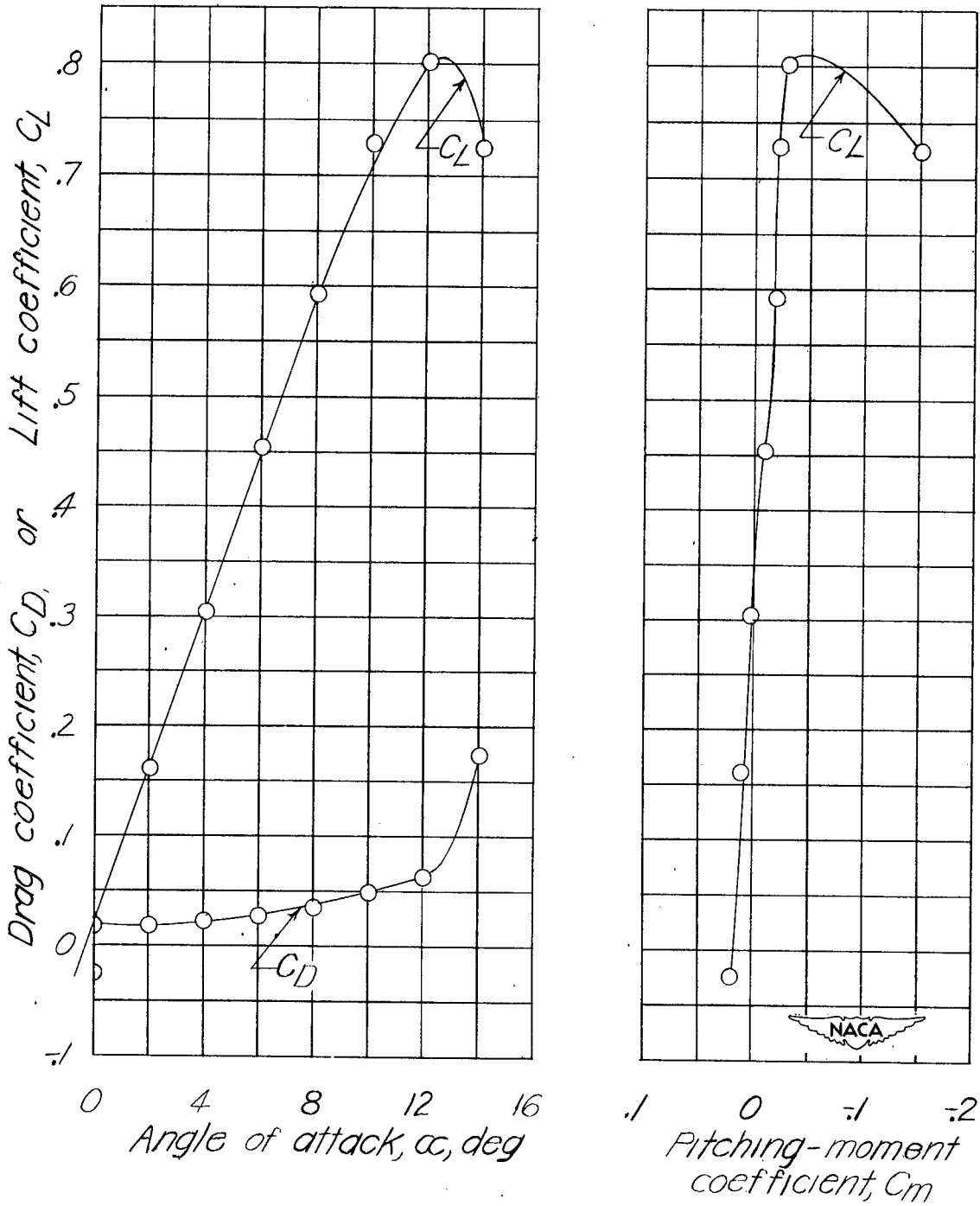
(a) Equivalent straight-wing model. Figure 6.— Force tests of models.
