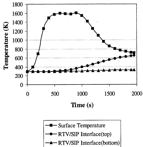
Figure 24: Temperature Distribution for TPS Stack of Five Materials.
