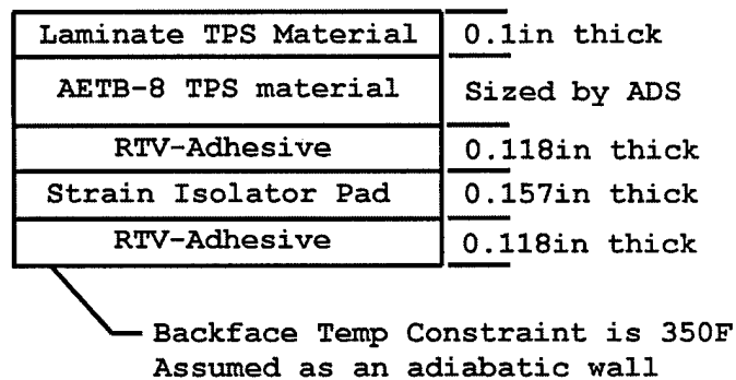
Figure 32. Schematic for Laminate Materials.
