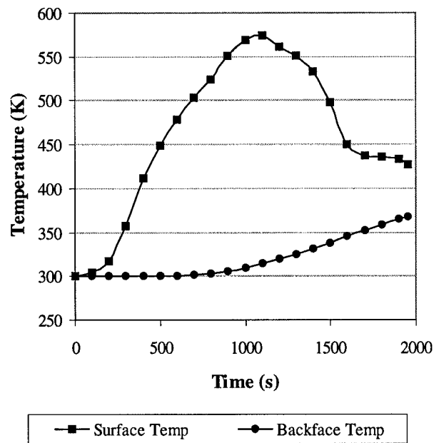
Figure 20. Leeward Body Point Temperature History Case 2.
