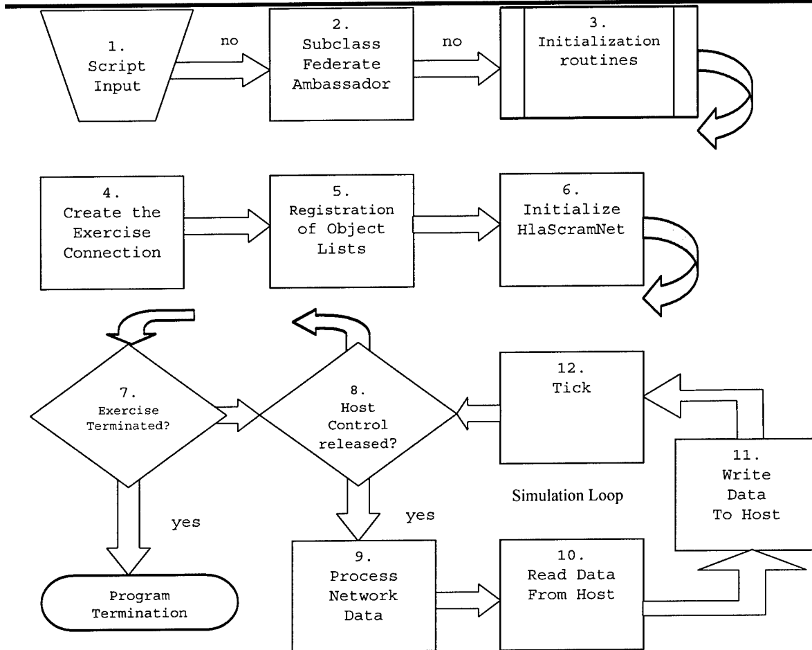
Figure 2. HLA-IU Software Flowchart
