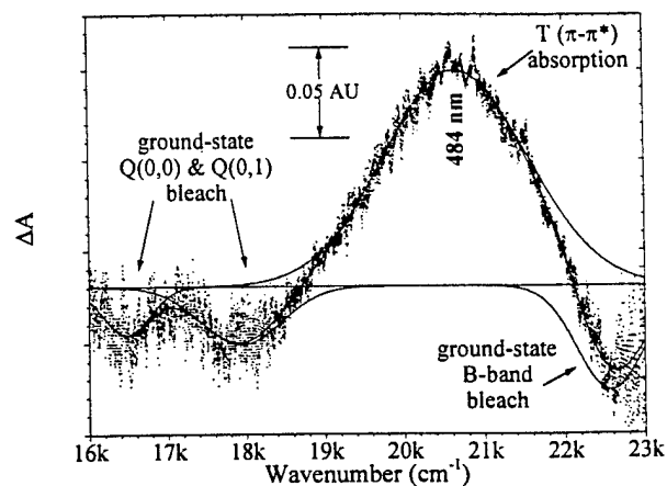
Figure 2. \Delta A spectrum showing \lambda_{\max} of the triplet \pi - \pi^* transition for a [\text{Zn}(\text{PyP})_2]_2 in toluene. This transition is red shifted from its monomeric analogues.
