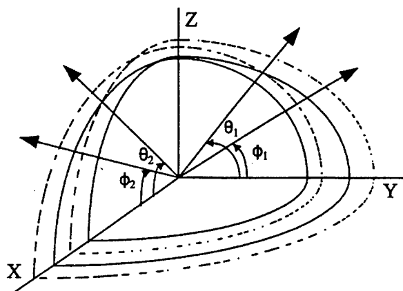
Fig. 12. Optical indicatrix (refractive index) surfaces for ABP, and the phase-matched propagation directions. \theta_1 and \theta_2 represent type-I, \phi_1 and \phi_2 represent type-II phase-matching. The continuous and dashed lines represent 1064 and 532 nm, respectively.
