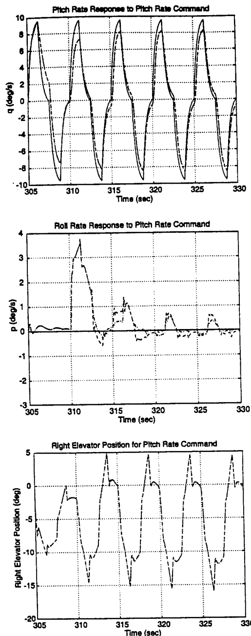
Fig. 3 Responses to a large pitch rate command: methods 1 and 2.
