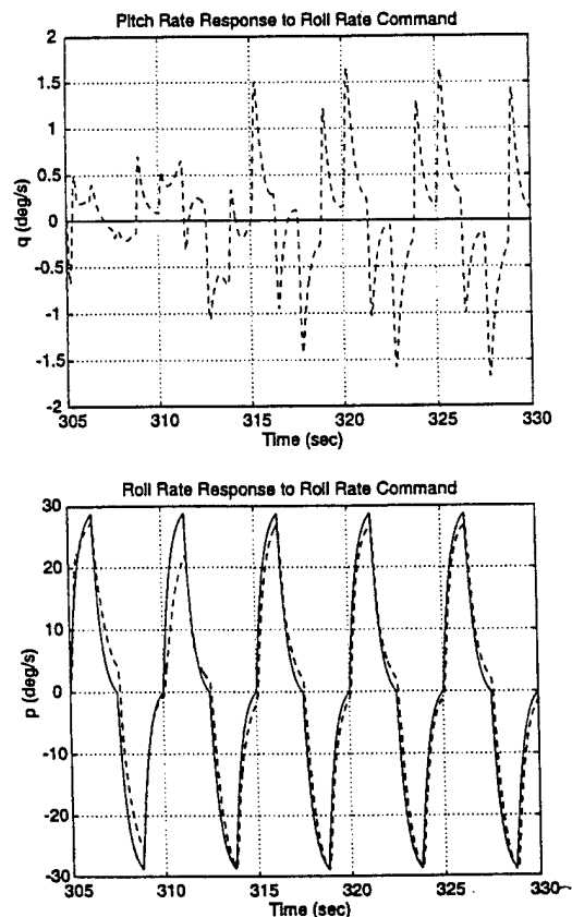
Fig. 5 Responses to a large roll rate command with locked stabilator and aileron: method 4.
