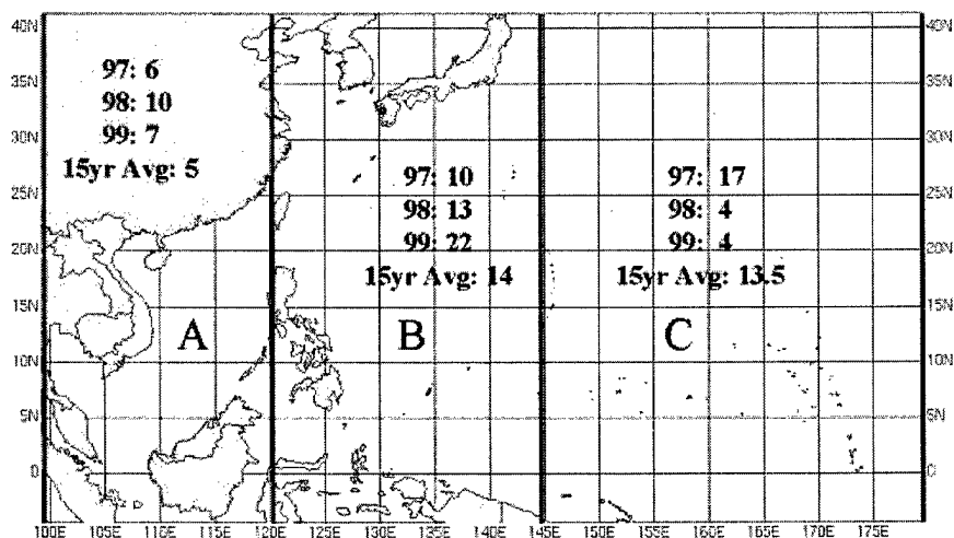
Figure 1-1. Comparison of the number of tropical cyclones that developed within 3 designated areas for 1997, 1998, 1999 and the 15-year average.
