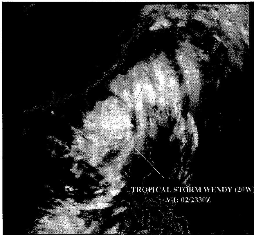
Fig 1-20-2. 022330Z September visible satellite image of Tropical Storm Wendy (20W) at its maximum intensity (40 kt), southwest of Taiwan.
