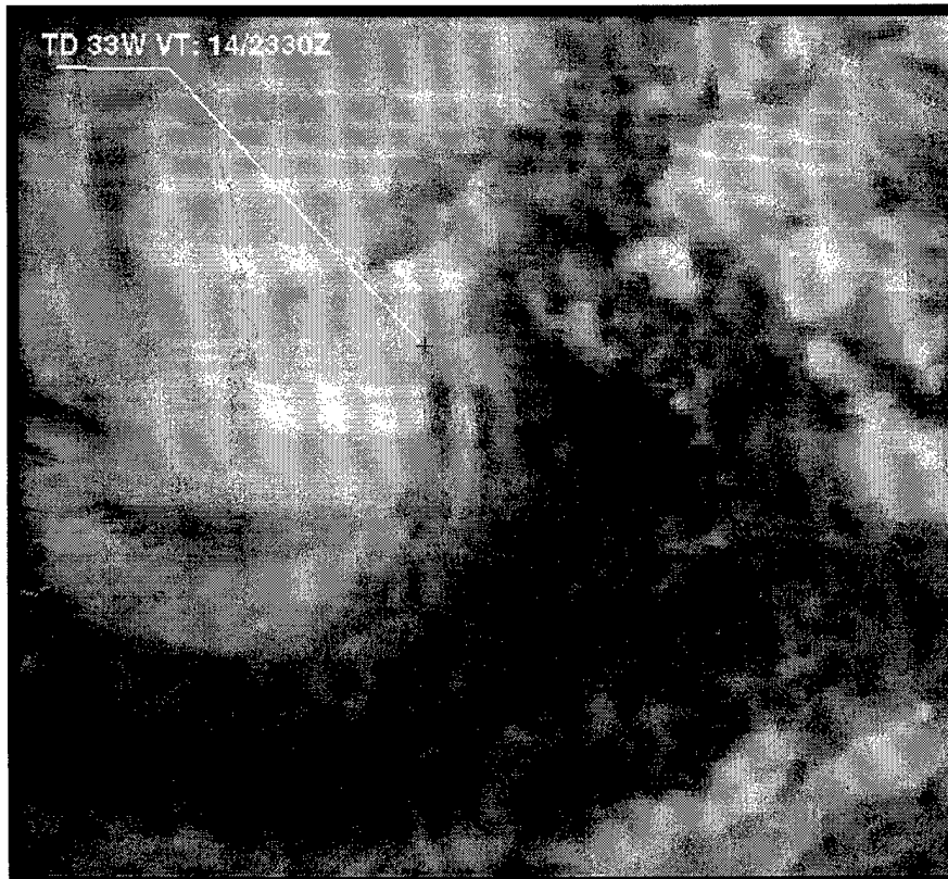
Figure 1-33-1. 142330Z December GMS-5 visible image of TD 33W as it approached the Vietnam coast. Current intensity is 30 kt.
