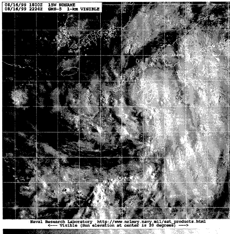
Figure 1-15-2. 162224Z August GMS-5 visible image. TD 15W was a 25 kt TD as it approached Kyushu, Japan. TD 15W made landfall 4 hours later over Kyushu.
