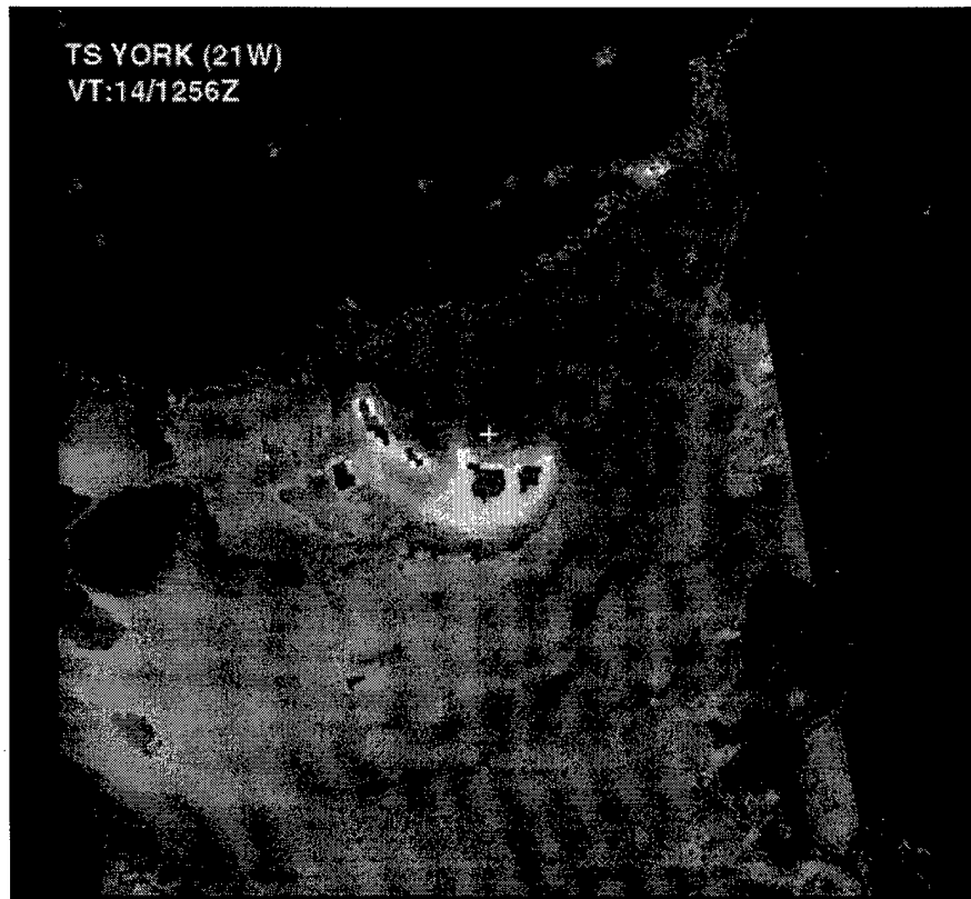
Figure 1-21-1. A special sensor microwave satellite image of developing Tropical Storm York (21W) at 141256Z September, in the South China Sea southeast of Hong Kong.
