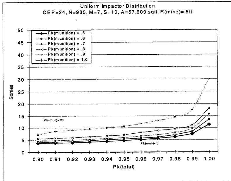
Figure 14: Effect of Increased CEP on Uniform Distribution
