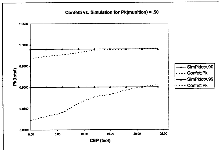
Figure 9: Confetti Approximation vs. Simulation Results at Pk_{munition} = .5
