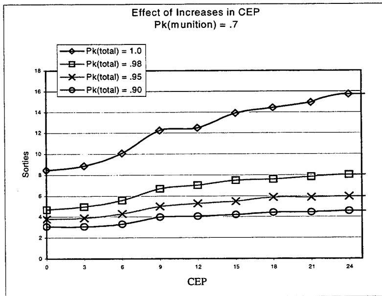
Figure 15: Effect of Increased CEP on Pk_{munition} = .7
