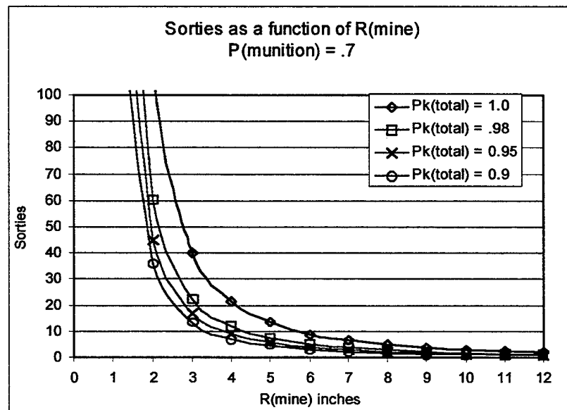
Figure 22: Effect of Decreased R_{mine} on Uniform Distribution A change in R_{mine} to 3 inches. Note that the scale of the y axis has been changed from the base case graph (Fig(11)) to account for the large increase in sorties.
