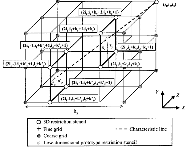
FIG. 5. Full-dimensional stencil of the restriction operator.
