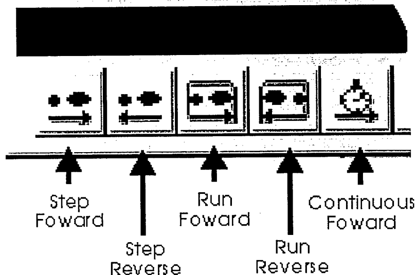
Figure 30. Simulation Toolbar.
