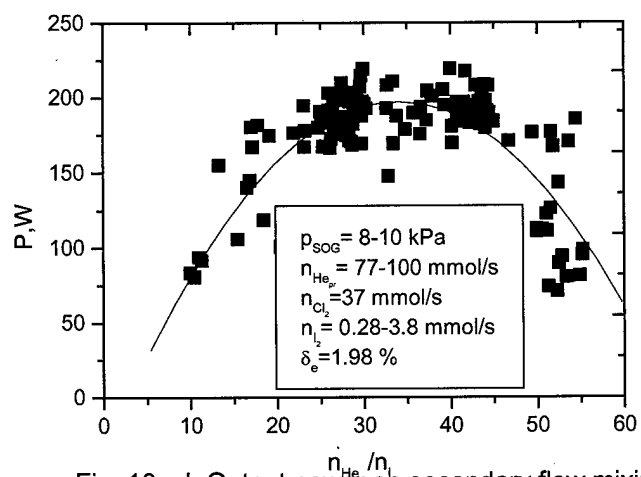
Fig. 10c,d: Output power on secondary flow mixing
