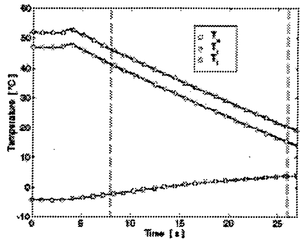
Figure 7: Time History of T_r , T_r , T_w , h , q (Uncooled Run #6) (Dashed Lines Indicate Range of Useful Data)
