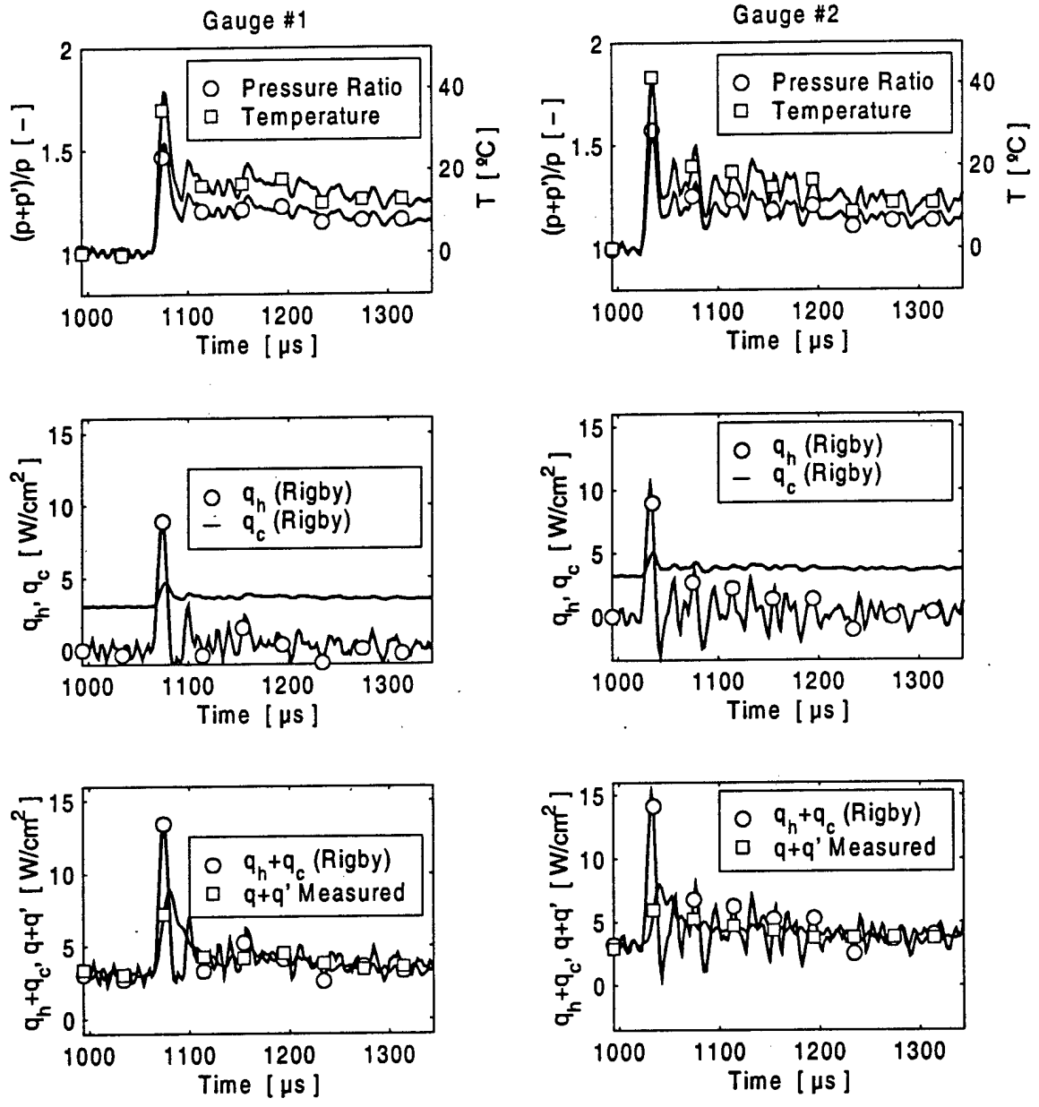
Figure 3.54: Shock Passing Event from Run #3 Without Film Cooling. Rigby's Model And Comparison with Data. Pressure and Heat Flux Signals Corrected According to Section "Signal Processing" 3.4.
