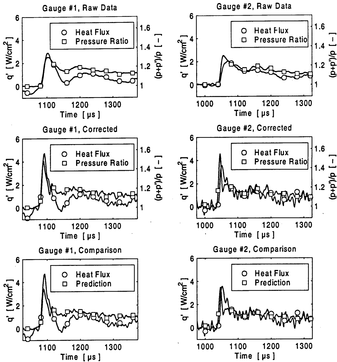
Figure 3.43: Shock Passing Event from Run #3 without Film Cooling. Moss' Model And Comparison with Data.
