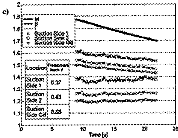
Figure 10: Time Histories from Cooled Run #5 a) Heat Transfer and Heat Transfer Coefficient b) All Relevant Temperatures c) Density Ratio, Blowing Ratio, Momentum Ratio (Dashed Lines Indicate Range of Useful Data)
