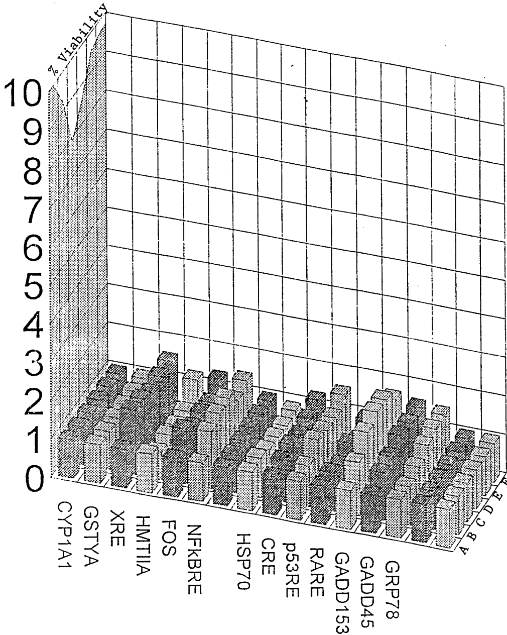
FIG. 1. Fold Induction of 13 Human Stress Response genes after laser-light exposure. The vertical scale represents fold induction of the genes designated in the foreground and percent survival the parental cell line as shown on the left wall. The exposure treatments are along the right floor (A-F) and described in Table 1.
