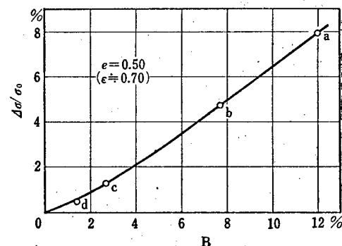
Fig. 1·22 Relation Between the Barreling Coefficient B and Compression Stress-Deviation.
