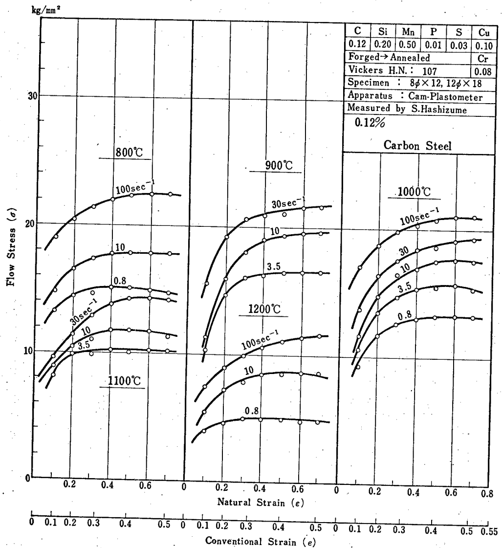
Fig. 4-23 Flow Stress-Strain Curves of 0.12% C Steel. Temperature Range: 800~1200°C, Strain Rate Range: 0.8~100 \text{sec}^{-1} .
