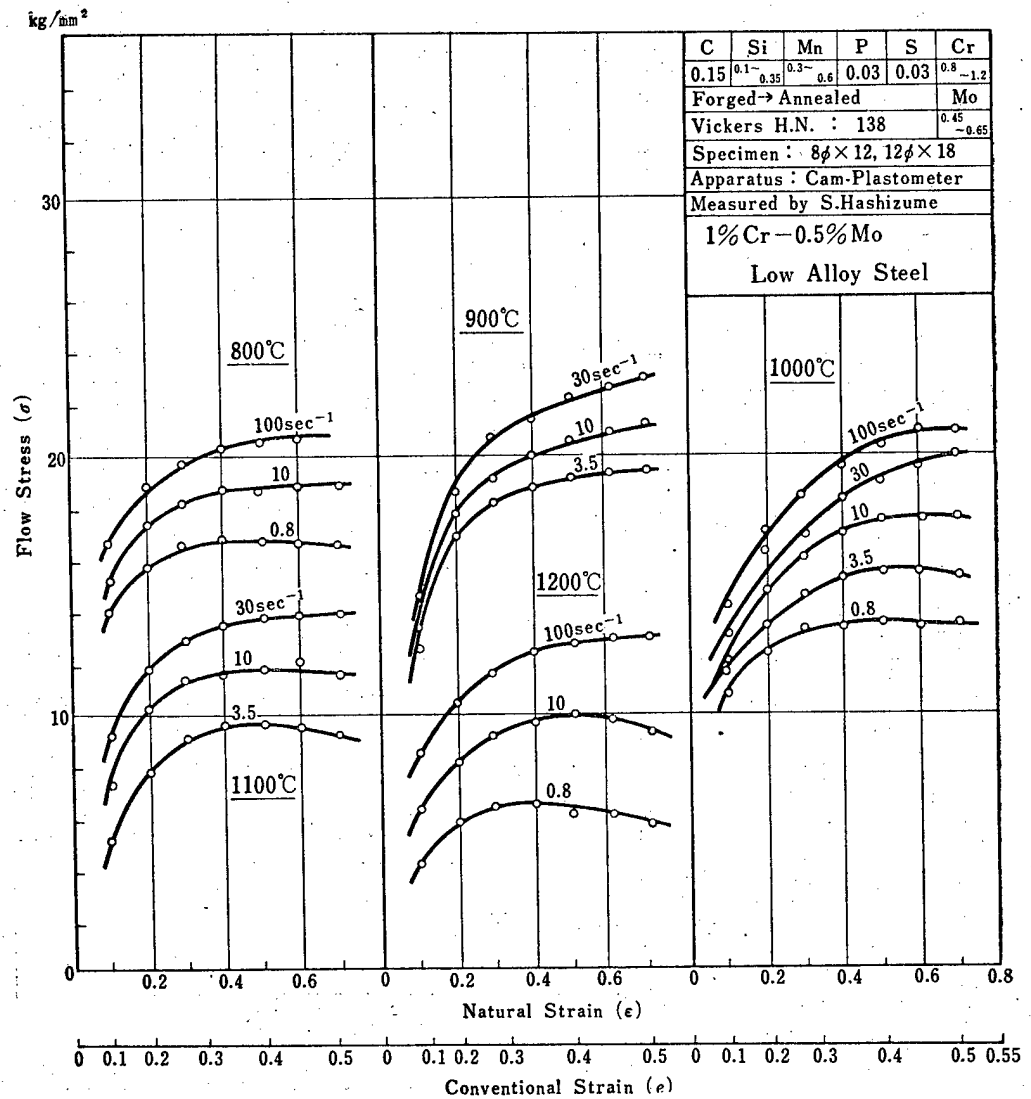
Fig. 4-54 Flow Stress-Strain Curves of 1%Cr-0.5%Mo Low Alloy Steel. Temperature Range: 800~1200°C, Strain Rate Range: 0.8~100 sec -1 .
