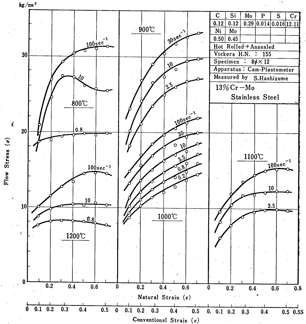
Fig. 4-59 Flow Stress-Strain Curves of 13% Cr-Mo Stainless Steel. Temperature Range: 800~1200°C, Strain Rate Range: 0.2~100 sec -1 .
