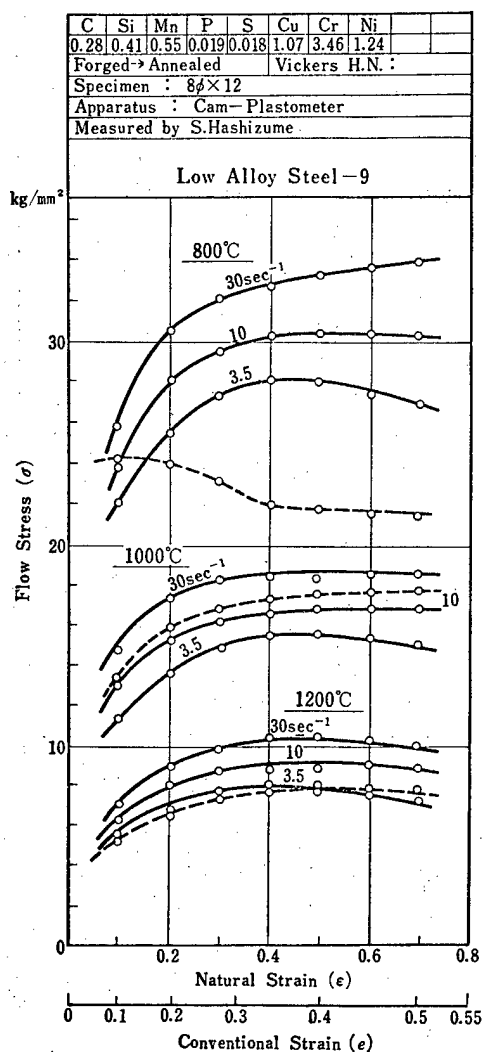
Fig. 4-46 Flow Stress-Strain Curves of Low Alloy Steel-9. Temperature Range: 800~1200°C, Strain Rate Range: 3.5~30 sec -1 .
