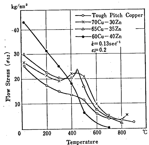
Fig. 2-5 Temperature Dependence of the Compression Stress of Copper and Copper-Zinc Alloys at \epsilon = 0.2 . Strain Rate: 0.13 \text{ sec}^{-1} .
