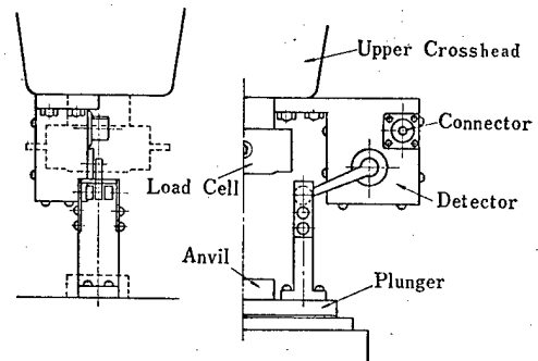
Fig. 1-11 Apparatus for Compression Strain Measurement.
