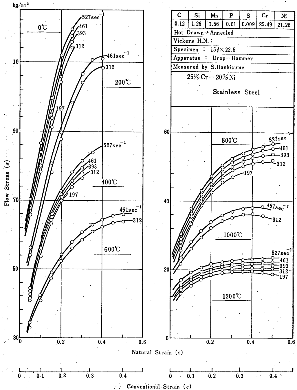
Fig. 4-70 Flow Stress-Strain Curves of 25% Cr-20% Ni Stainless Steel. Temperature Range: 0~1200°C, Strain Rate Range: 197~527 sec -1 .
