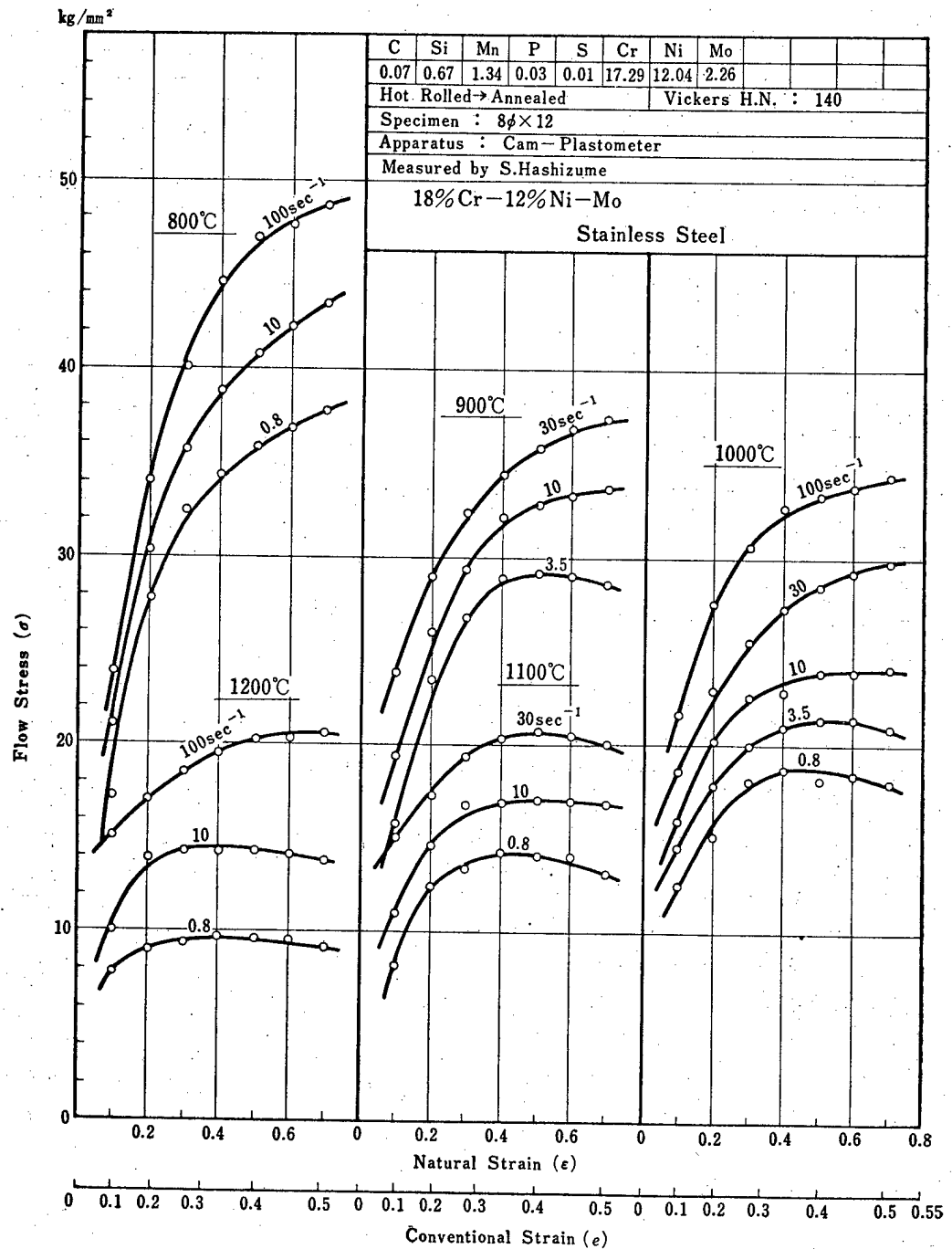
Fig. 4-68 Flow Stress-Strain Curves of 18%Cr-12%Ni-Mo Stainless Steel. Temperature Range: 800~1200°C, Strain Rate Range: 0.8~100 sec -1 .
