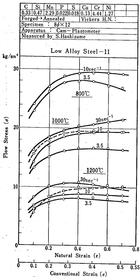
Fig. 4-48 Flow Stress-Strain Curves of Low Alloy Steel-11. Temperature Range: 800~1200°C, Strain Rate Range: 3.5~30 sec -1 .
