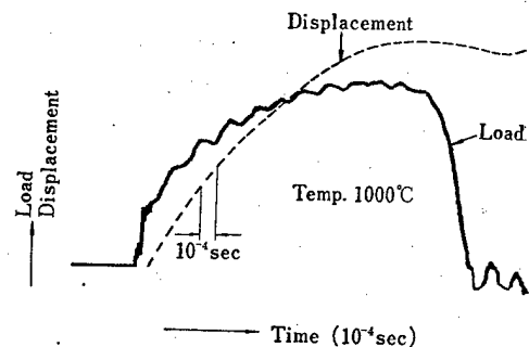
Fig. 1-12 Load & Displacement-Time Curve. Testing Machine..... Drop-Hammer Specimen ..... 0.12% C, Steel Hammer Weight..... 25 kg Height of Fall ..... 1 m X Axis ..... Time Y_1 Axis ..... Load Y_2 Axis ..... Displacement
