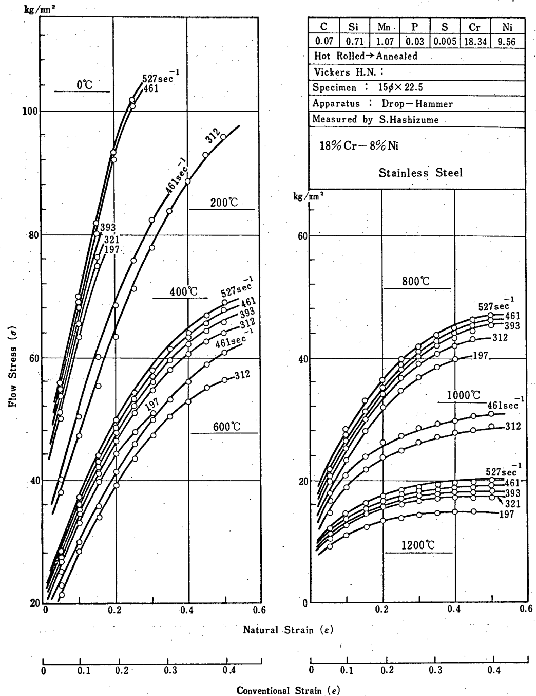
Fig. 4-67 Flow Stress-Strain Curves of 18%Cr-8%Ni Stainless Steel. Temperature Range: 0~1200°C, Strain Rate Range: 197~527 \text{sec}^{-1} .
