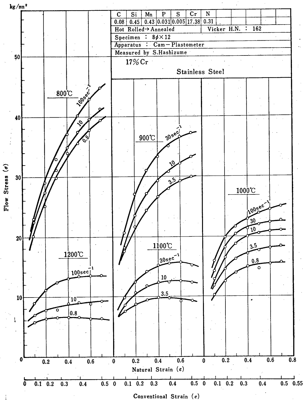
Fig. 4-60 Flow Stress-Strain Curves of 17%Cr Stainless Steel. Temperature Range: 800~1200°C, Strain Rate Range: 0.8~100 sec -1 .
