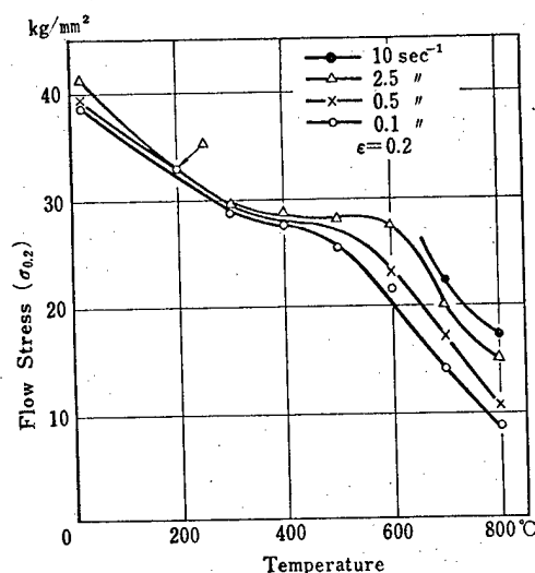
Fig. 2-9 Temperature Dependence of the Compression Stress of 93%Cu-7%Sn Alloys at \epsilon=0.2 .
