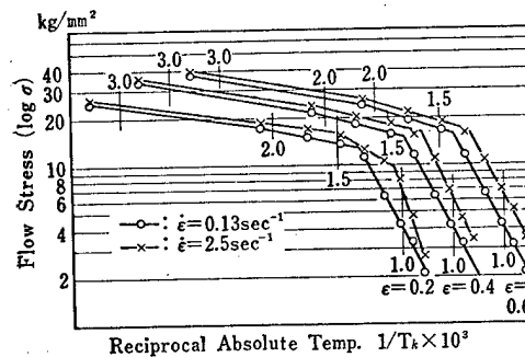
Fig. 2-3 Arrhenius Plot of the Flow Stress of Tough Pitch Copper.
