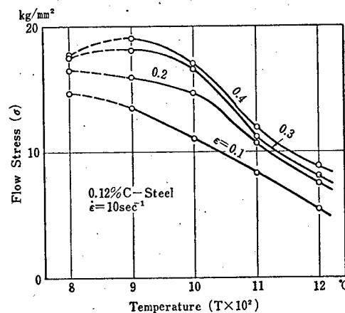
Fig. 3.4 Temperature dependence of the Flow Stress of 0.12% C-Steel. Strain ( \epsilon ) = 0.1–0.4, Strain rate ( \dot{\epsilon} ) = 10 sec ^{-1} .
