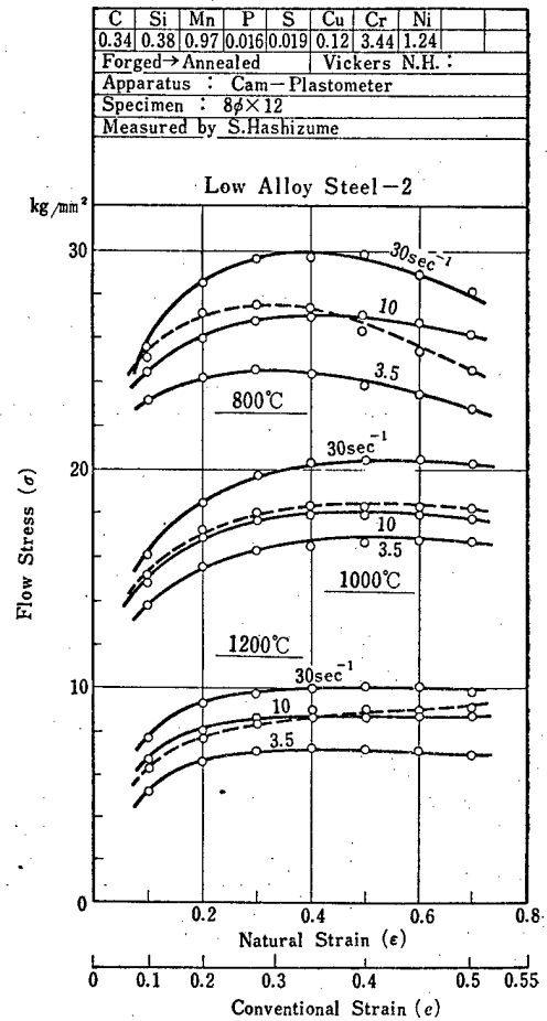
Fig. 4-39 Flow Stress-Strain Curves of Low Alloy Steel-2. Temperature Range: 800~1200°C, Strain Rate Range: 3.5~30 sec -1 .
