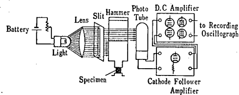
Fig. 1-10 Apparatus for Strain Measurement. (Drop-Hammer)
