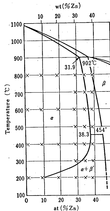
Fig. 2-4 Phase Diagram of the Cu-Zn System. Crosses denote the Positions at which Measurements were Made.
