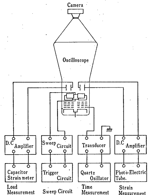
Fig. 1-6 Arrangement of the Measuring Instruments.
