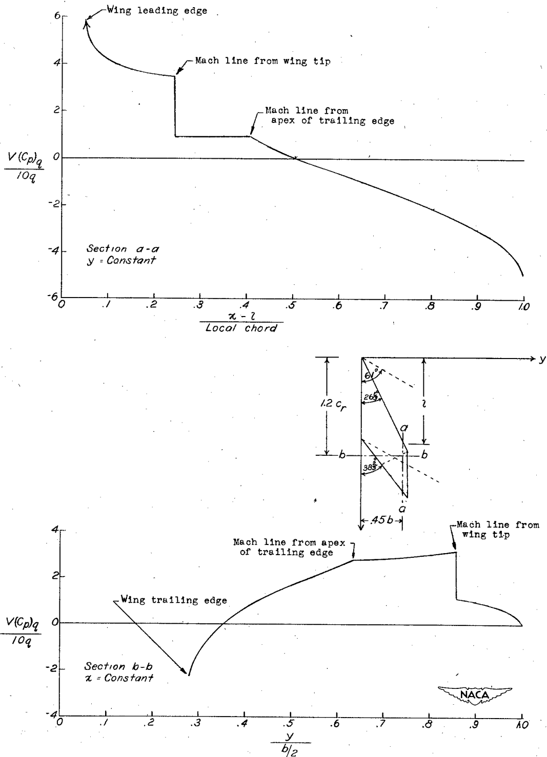
Figure 5.- Sectional chordwise and spanwise pressure distributions for a typical wing pitching about its apex. Intersection of the sectional planes a-a and b-b with the wing edges and Mach lines are noted on pressure curves.
