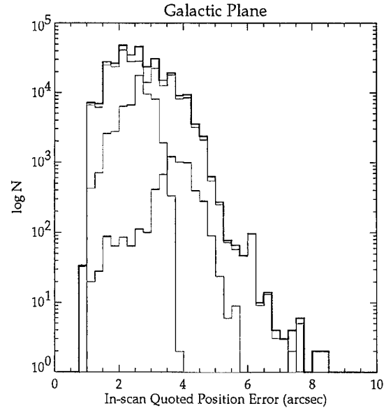
Figure 23: Quoted in-scan position uncertainties ( 1\sigma ) of the Galactic plane sources.
