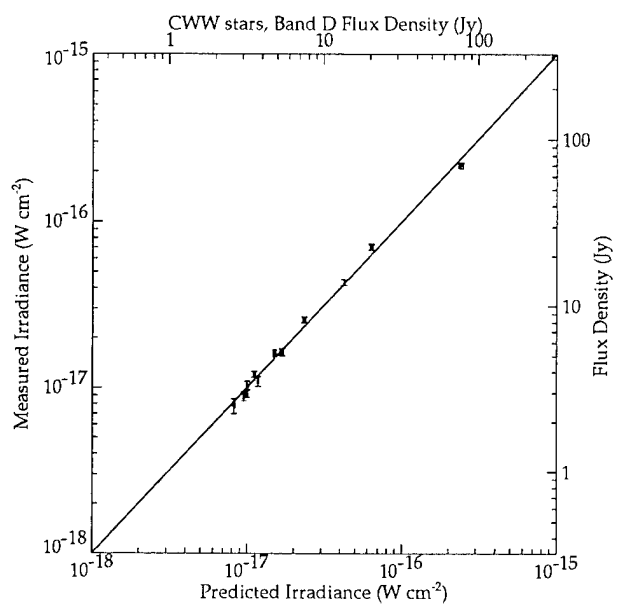
Figure 9: Band D calibration stars.
