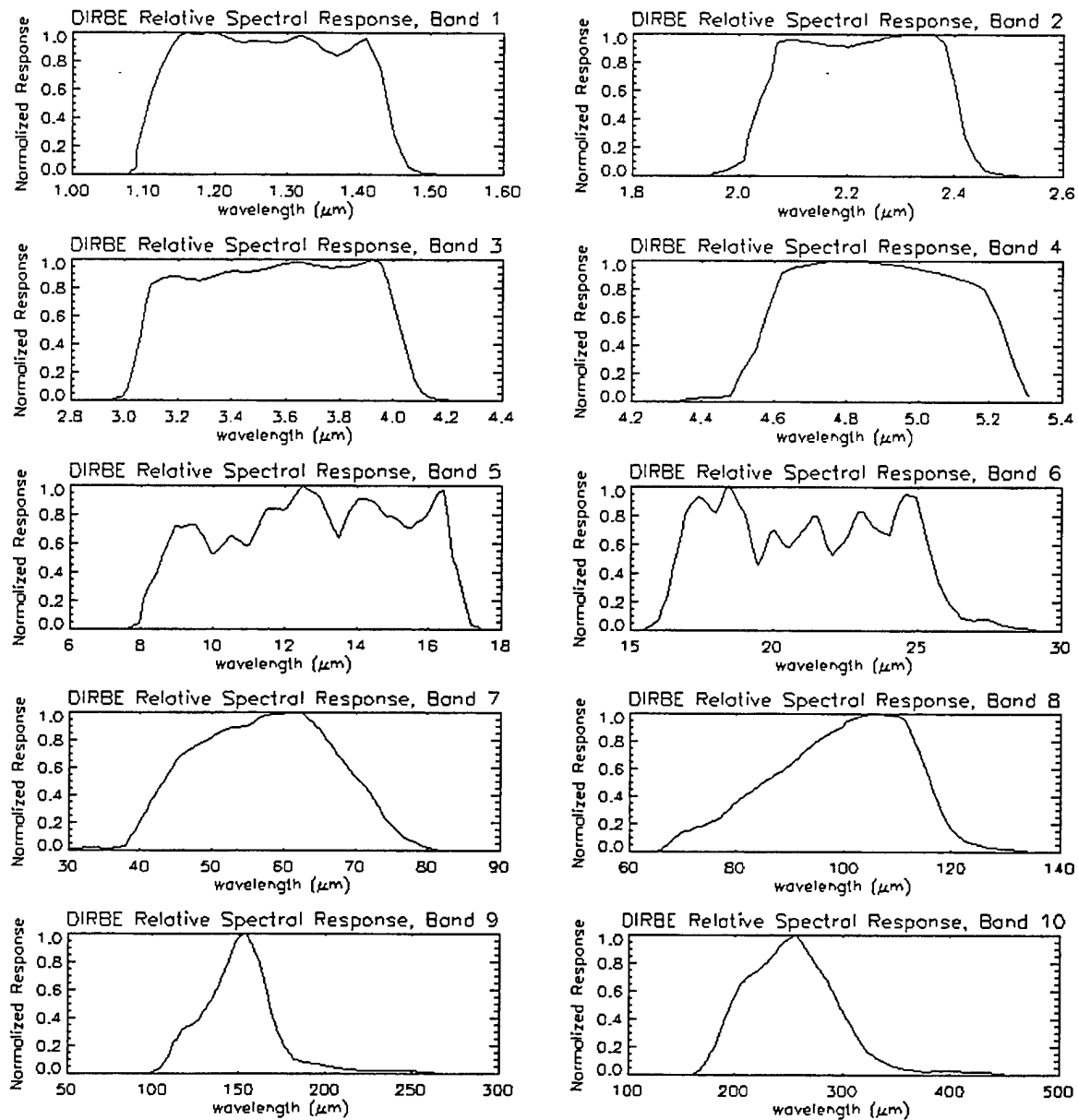
Figure C-2 DIRBE Wavebands
