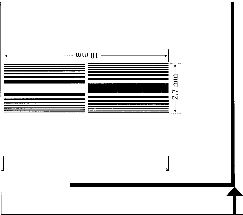
Figure 3.2 : Mask layout for phase modulator (in-line openings) (C1)
