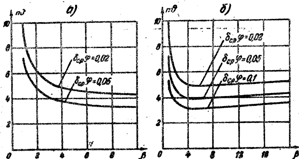
Fig. 2. Pulse length needed to give a specified \delta_m \phi a) fixed bias ( \sin \theta_o = 1, \theta_g = 0 ), b) self-bias ( \sin \theta_o = 1, \theta_g = 0 )
