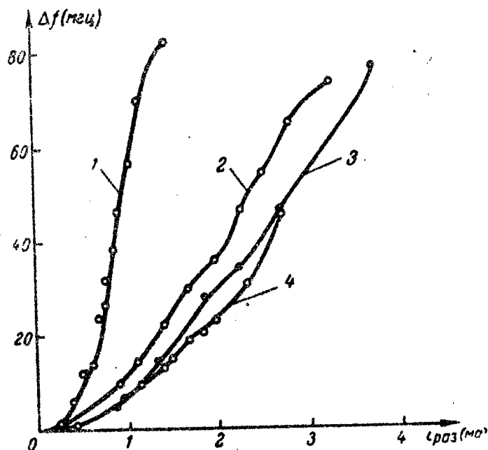
Fig. 7: Resonator retuning as a function of the discharge current in the 10 cm range (neon-filled):
