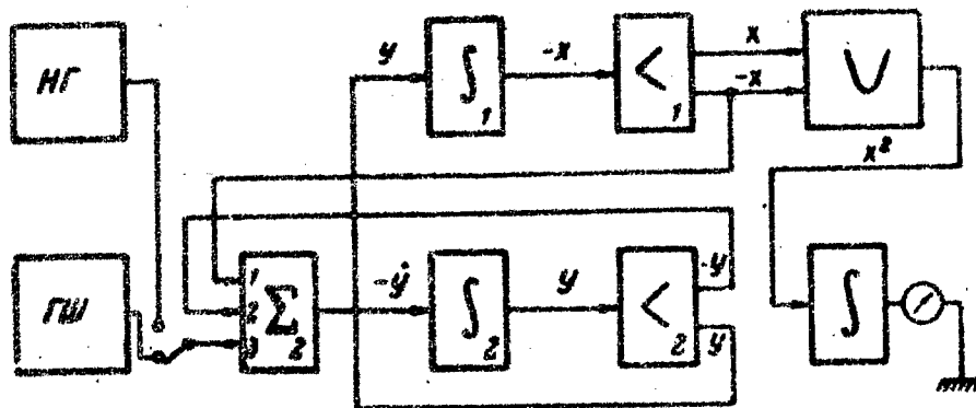
Fig. 2. Block diagram of the analog used in the noise-level measurements
