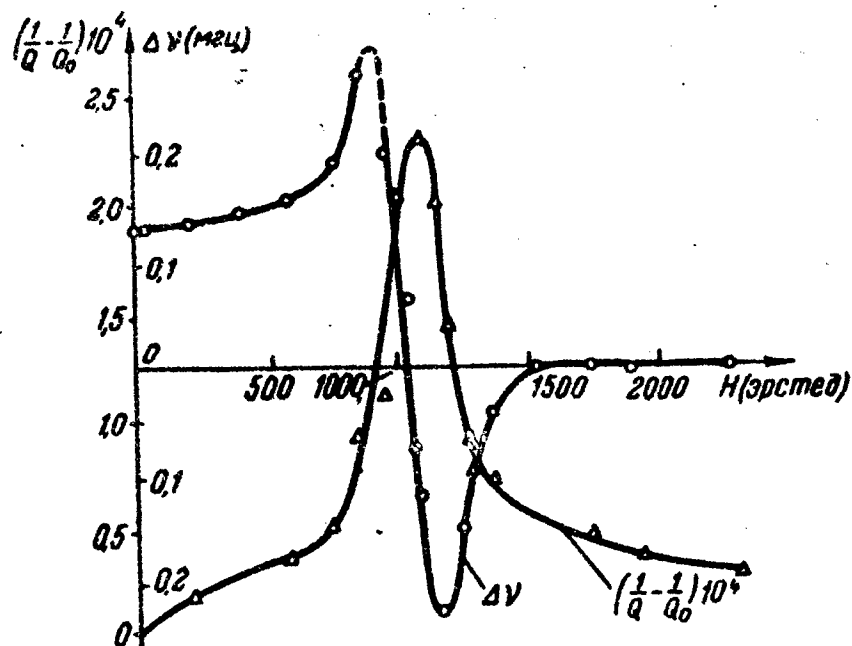
Fig. 2: High-frequency losses in discharge (1/Q - 1/Q_0) and resonator retuning \Delta f as functions of the value of the external steady magnetic field H (Ne 0.95 mm Hg).
