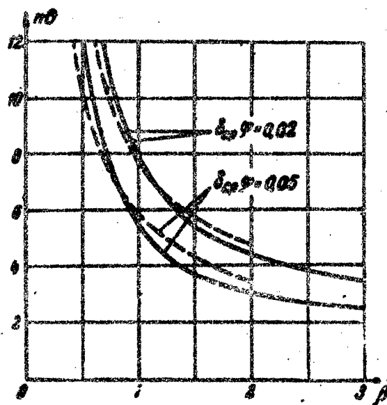
Fig. 3. Time taken for an external signal to pull an oscillator with self-bias into phase ( \sin \theta_o = 1, \theta_g = 0 )
