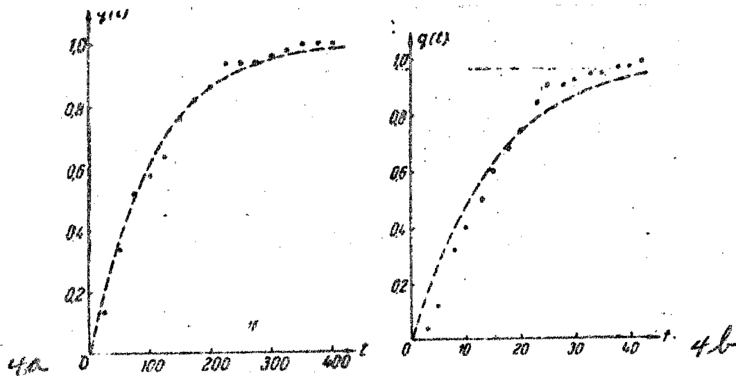
Fig. 4. Excitation probability.
