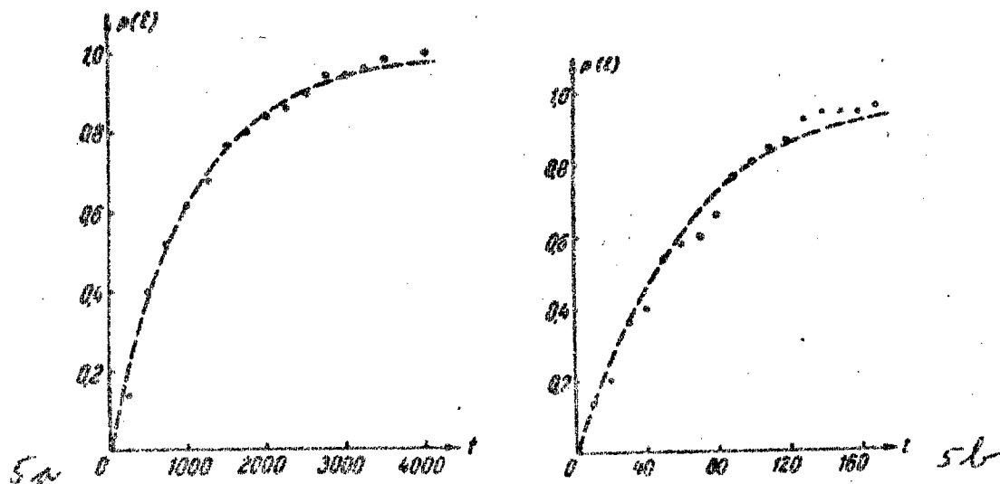
Fig. 5. Quenching probability.
