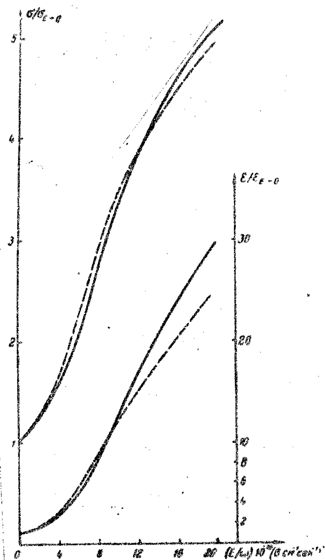
Fig. 5 Dependence of \epsilon/\epsilon_{E \rightarrow 0} and \sigma/\sigma_{E \rightarrow 0} on E/\omega in hydrogen in a high-frequency field. Broken lines represent the results of calculations in accordance with the formulas of the elementary theory.
