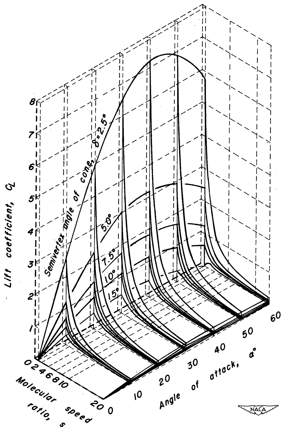
Figure 11.— Cone lift coefficient, diffuse reflection.
