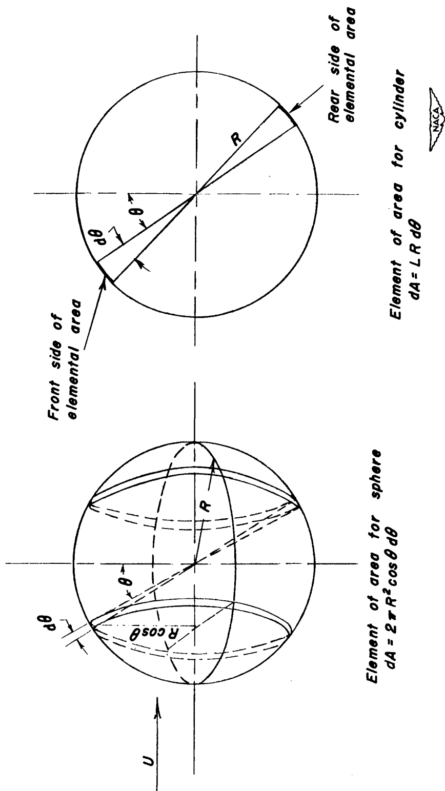
Figure 2.-Elemental areas for sphere and cylinder.
