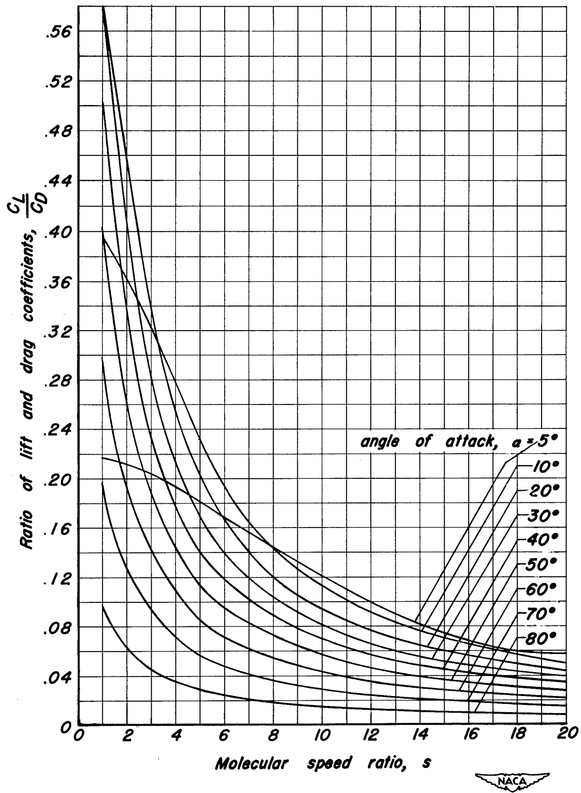
Figure 6.- Flat-plate lift-drag ratio, diffuse reflection.
