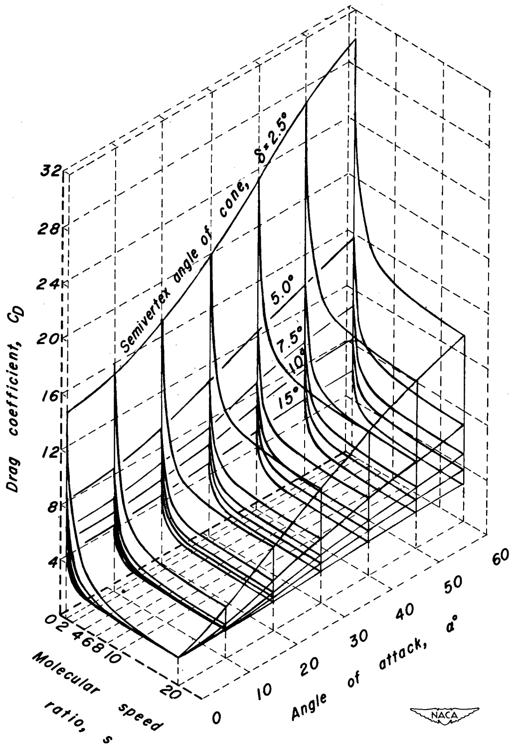
Figure 10.— Cone drag coefficient, diffuse reflection.
