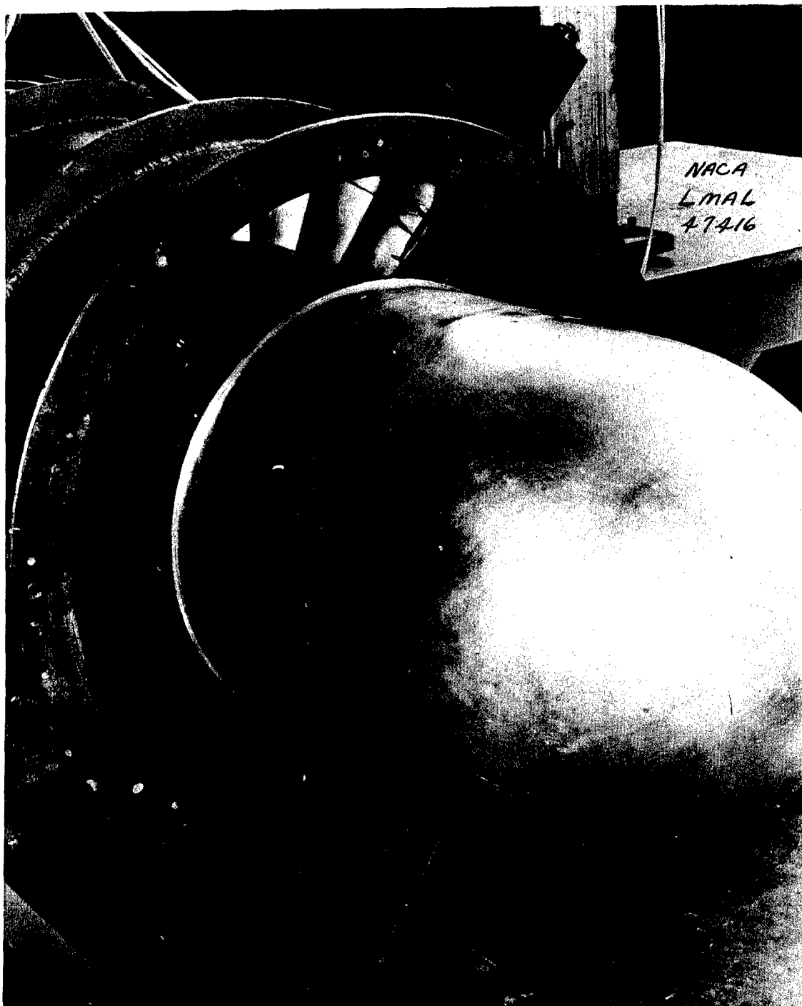
Figure 3.- View of fan showing \frac{1}{4} -inch inner spoiler.
