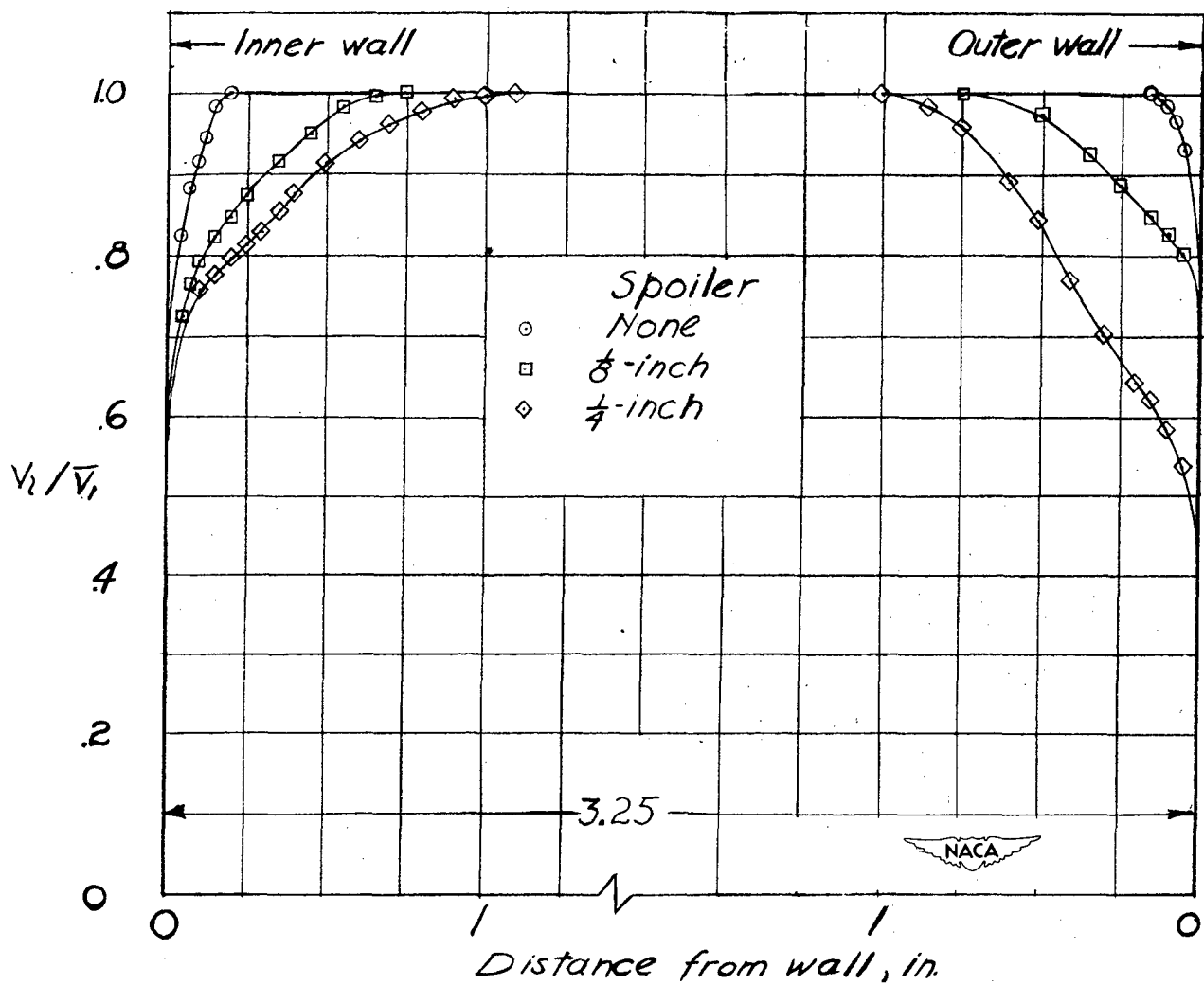
Figure 5.- Boundary-layer profiles upstream of fan and 4 inches downstream of spoiler. Maximum air-flow condition.
