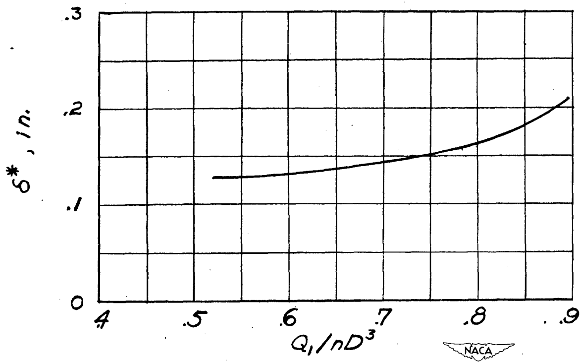
Figure 6.- Variation of \delta^* with Q_1/nD^3 upstream of fan. Rotational speed, 3020 rpm; \frac{1}{4} -inch outer spoiler.
