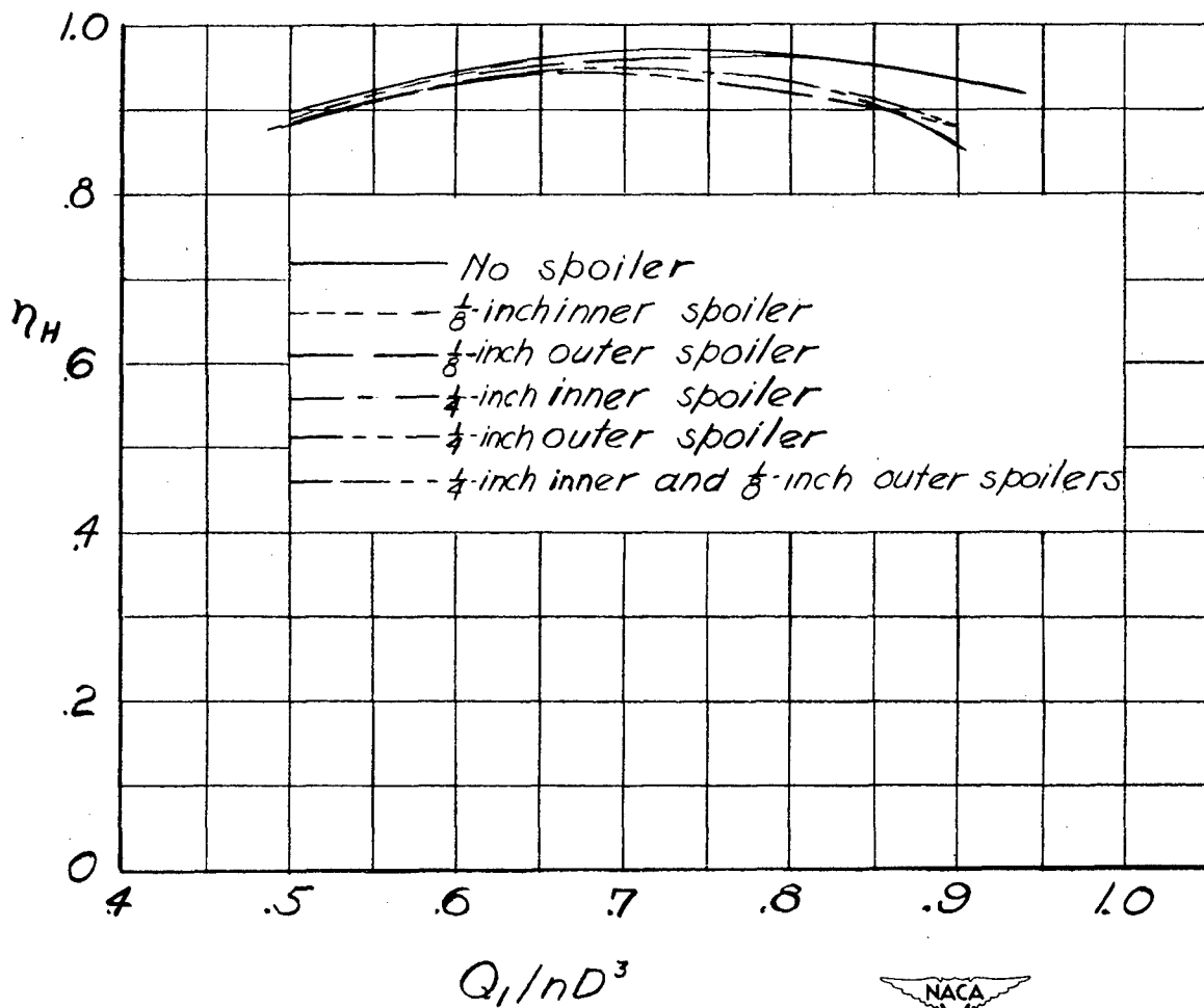
Figure 8.- Fan efficiencies.
