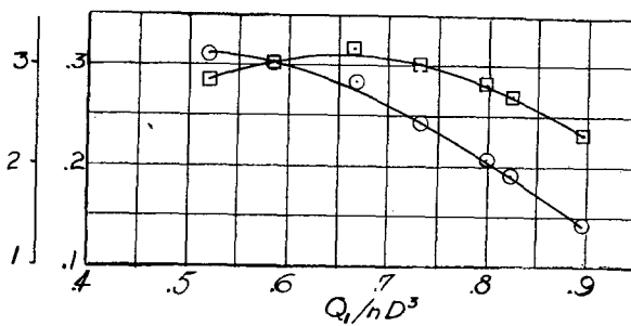
(e) \frac{1}{4} -inch outer spoiler.
