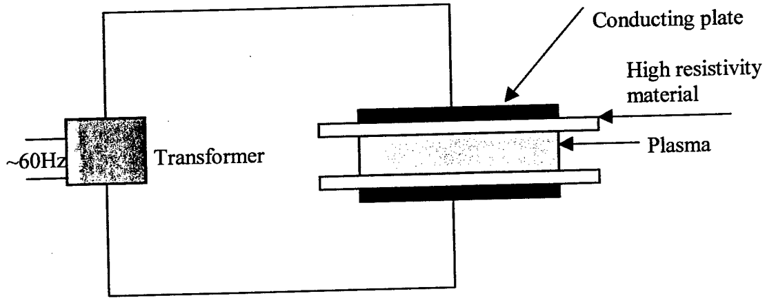
Fig. 3b AC (60 Hz) Driven RBD at Atmospheric Pressure
