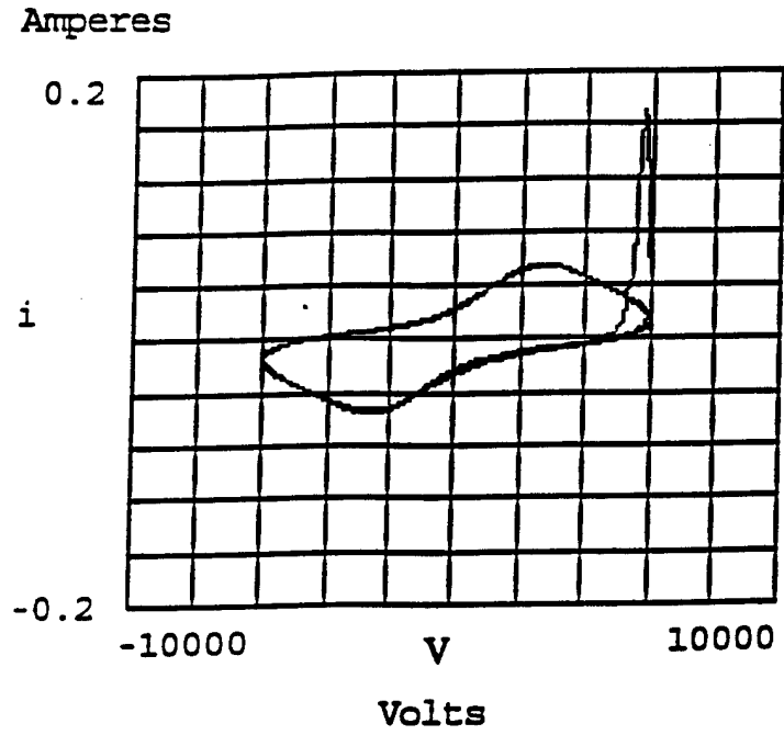
Fig. 4a Current-Voltage plot for f = 15.6 kHz.
