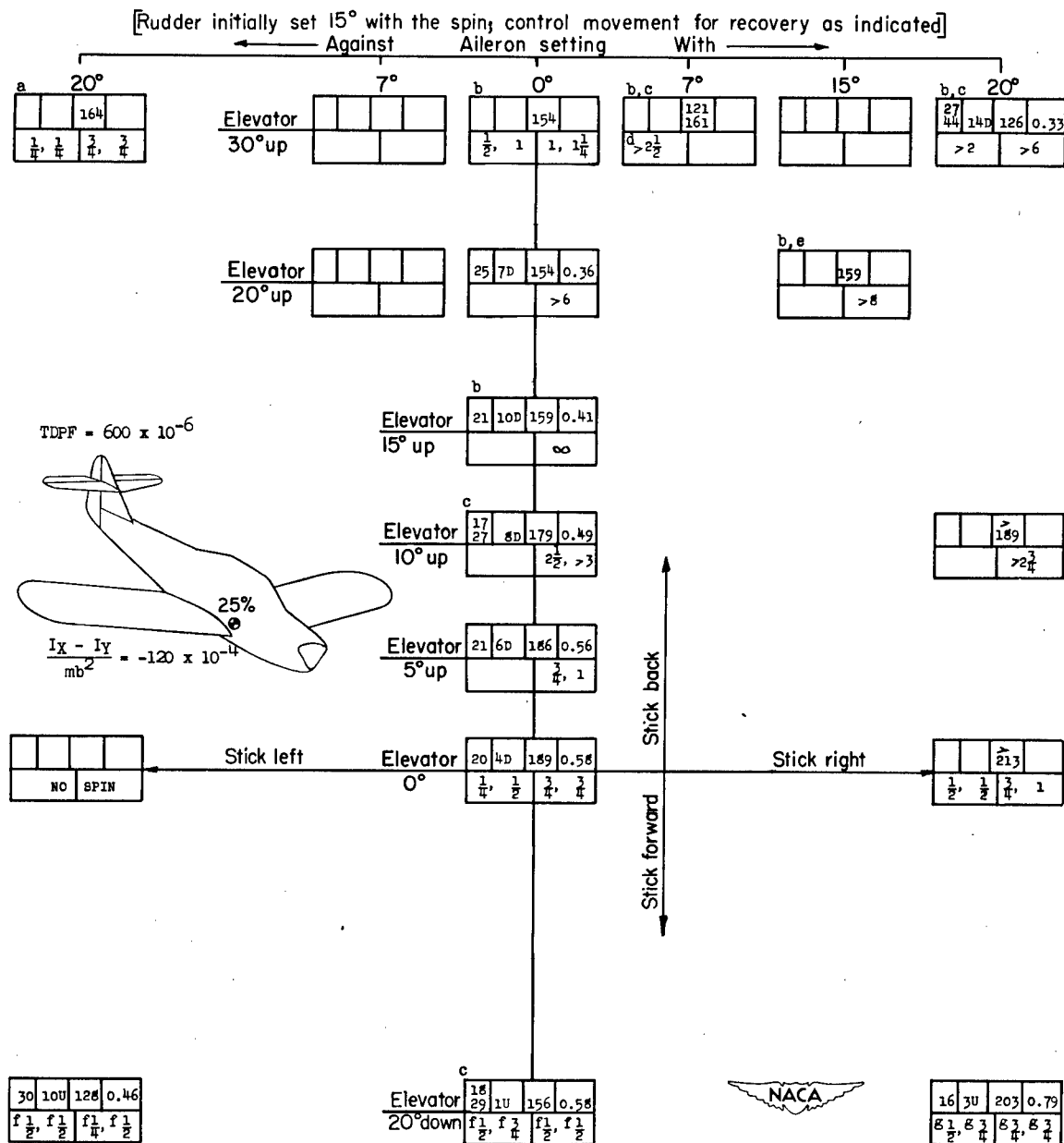
CHART 16.-SPIN AND RECOVERY CHARACTERISTICS OF MODEL FOR TEST CONDITION 16 LISTED IN TABLE III
