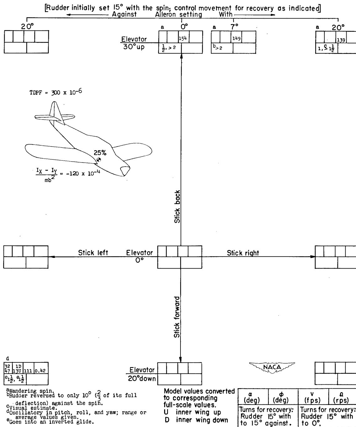
CHART 14.-SPIN AND RECOVERY CHARACTERISTICS OF MODEL FOR TEST CONDITION 14 LISTED IN TABLE III
