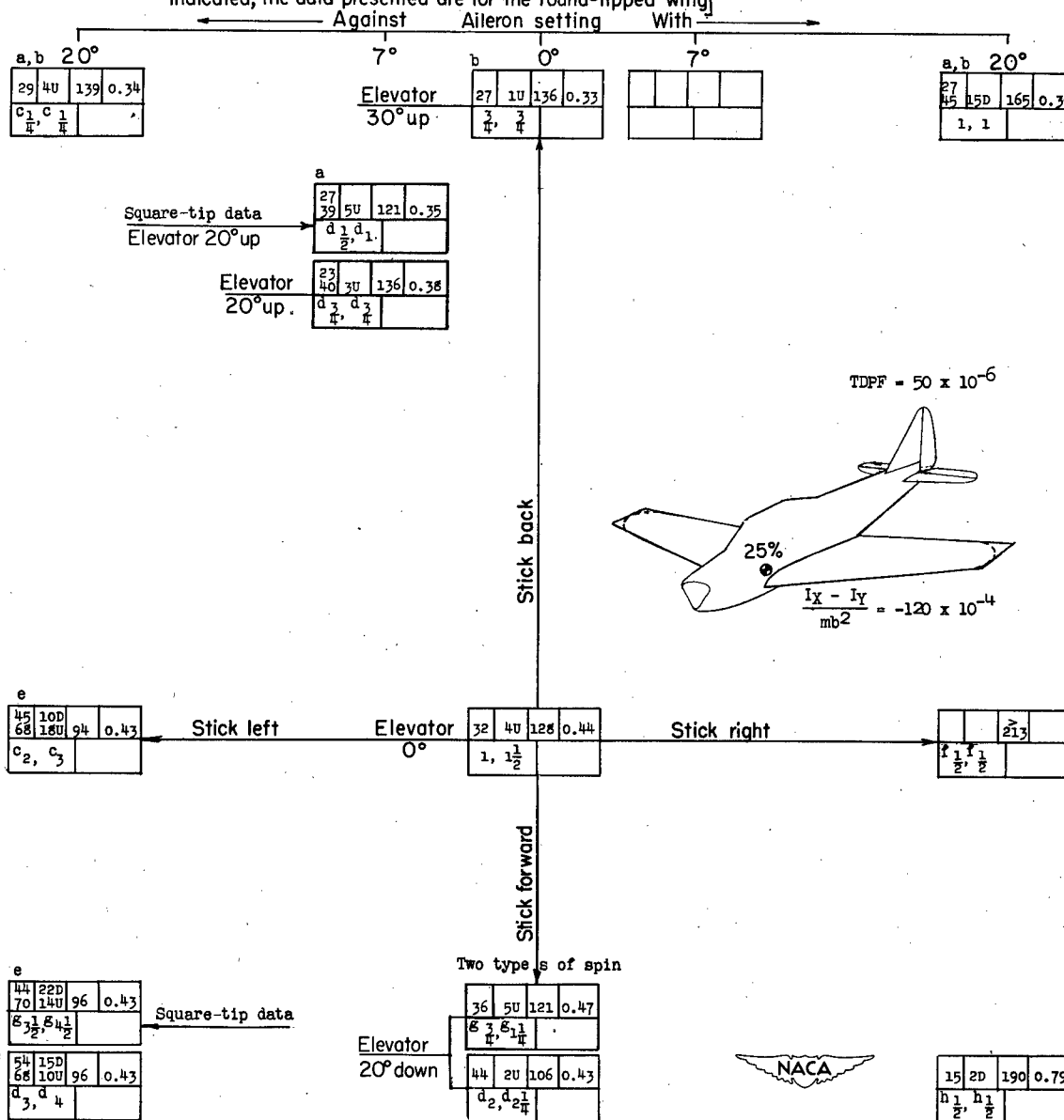
Chart 67-SPIN AND RECOVERY CHARACTERISTICS OF MODEL FOR TEST CONDITIONS 68 AND 75 LISTED IN TABLE III [Rudder initially set 30° with the spin; control movement for recovery as indicated; unless otherwise indicated, the data presented are for the round-tipped wing]
