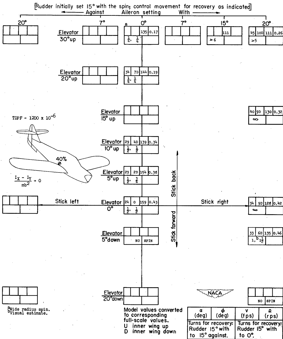
CHART 21.-SPIN AND RECOVERY CHARACTERISTICS OF MODEL FOR TEST CONDITION 21 LISTED IN TABLE III
