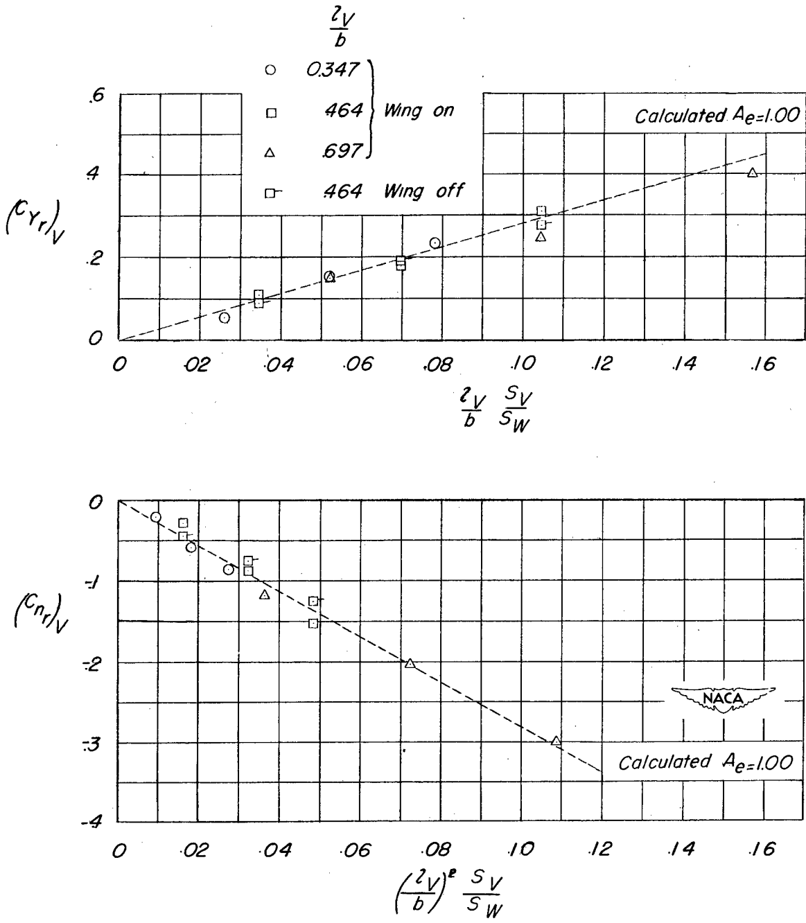
Figure 20.- Effect of tail area and tail length on (C_{Yr})_V and (C_{nr})_V at \alpha = 0^\circ . Horizontal tail off; wing slat off.
