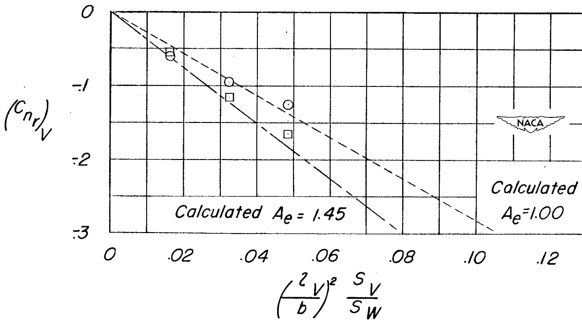
Figure 23.- Effect of horizontal tail on (C_{Y_r})_V and (C_{N_r})_V at \alpha = 0^\circ . Wing slat on; fuselage 2; \frac{z_V}{b} = 0.464 .
