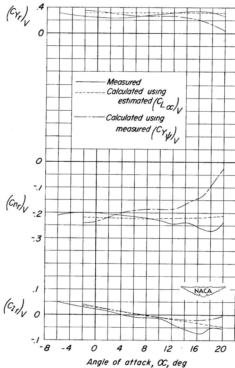
Figure 26.- Comparison of the measured and calculated variation with angle of attack of (C_{Yr})_V , (C_{Nr})_V , and (C_{Lr})_V . Wing on; horizontal tail off; fuselage 3 \left(\frac{l_V}{b} = 0.697\right) ; vertical tail 2 \left(\frac{S_V}{S_W} = 0.150\right) .
