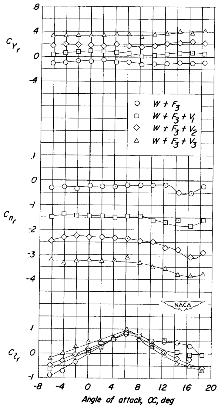
Figure 12.- Effect of vertical tail on C_{Yr} , C_{nr} , and C_{lr} . Wing on; horizontal tail off; fuselage 3; \frac{l_V}{b} = 0.697 .
