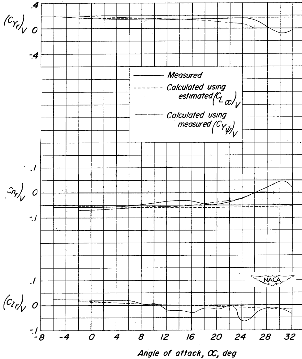
Figure 24.- Comparison of the measured and calculated variation with angle of attack of (C_{Yr})_V , (C_{nr})_V , and (C_{lr})_V . Wing on, horizontal tail off; fuselage 1 \left(\frac{l_V}{b} = 0.347\right) ; vertical tail 2 \left(\frac{S_V}{S_W} = 0.150\right) .
