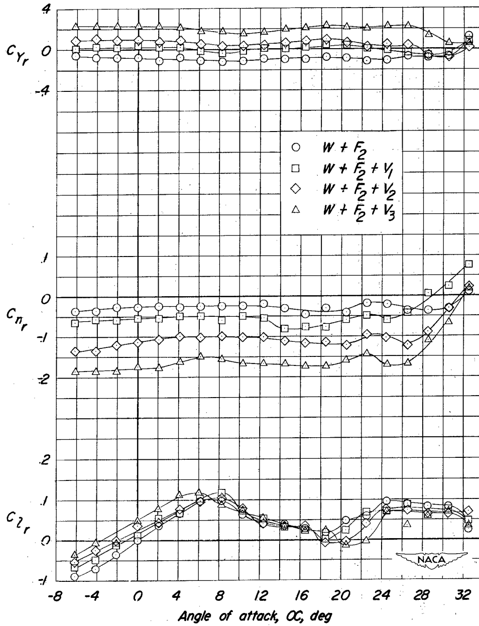
Figure 11.- Effect of vertical tail on C_{Yr} , C_{nr} , and C_{lr} . Wing on; horizontal tail off; fuselage 2; \frac{l_V}{b} = 0.464 .
