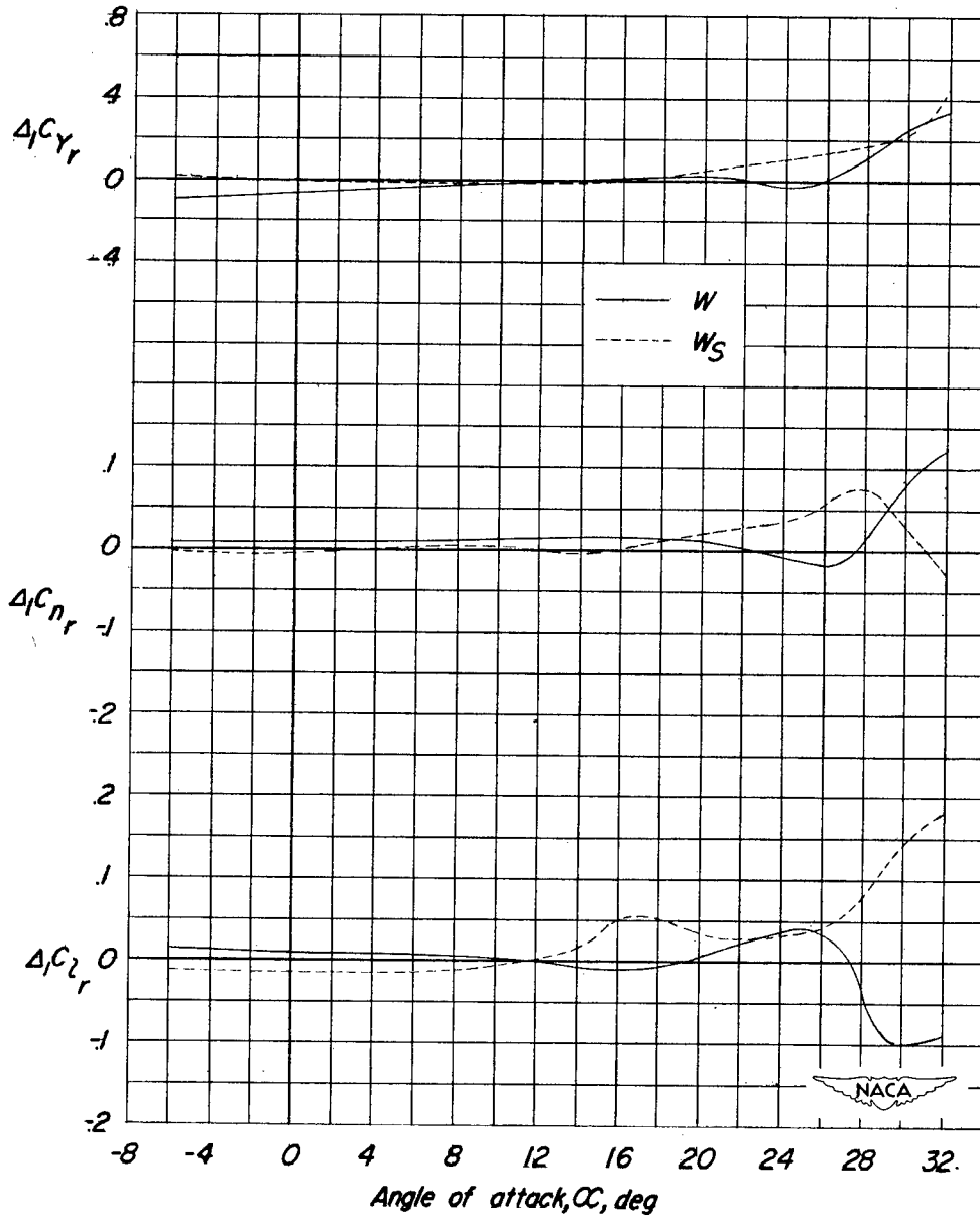
Figure 18.- Variation with angle of attack of the interference increments \Delta C_{Yr} , \Delta C_{Nr} , and \Delta C_{Lr} for plain wing and the wing with slat.
