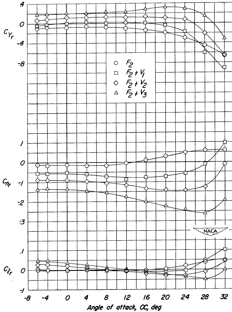
Figure 9.- Effect of vertical tail on C_{Yr} , C_{nr} , and C_{lr} . Wing off;
