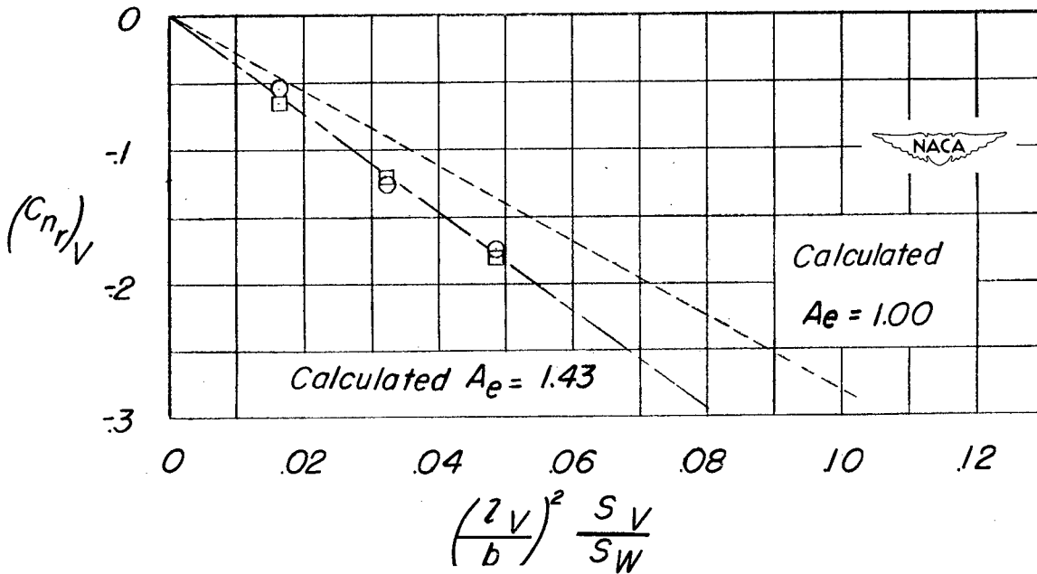
Figure 22.- Effect of tail area (wing on and off) on (C_{Yr})_V and (C_{nr})_V at \alpha = 0^\circ . Horizontal tail on; fuselage 2; \frac{z_V}{b} = 0.464 ; wing slat off.
