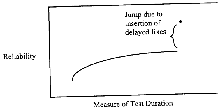
Figure 8. Graph of Reliability in a Test-Fix-Test Program with Delayed Fixes.
