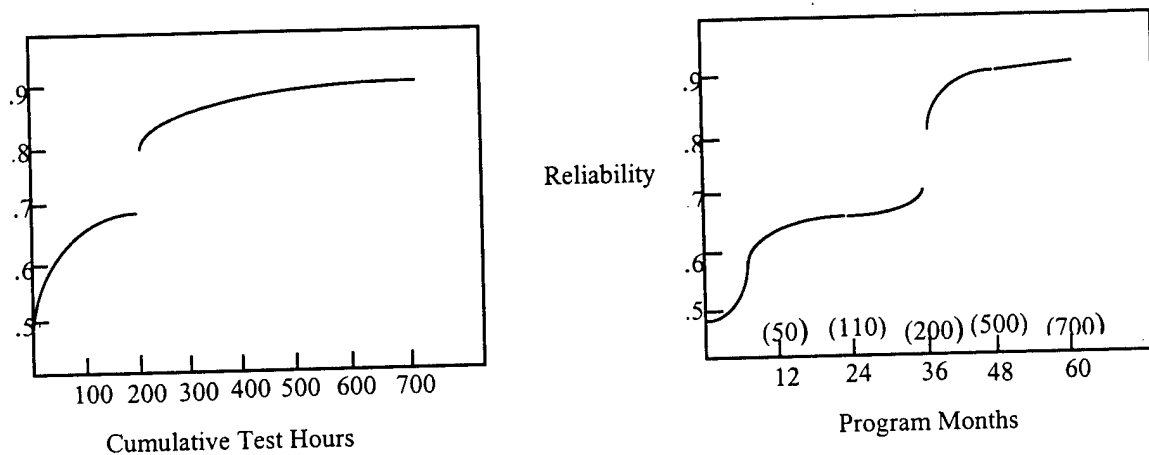
Figure 10. Comparison of Growth Curves Based on Test Duration Vs Calendar Time.
