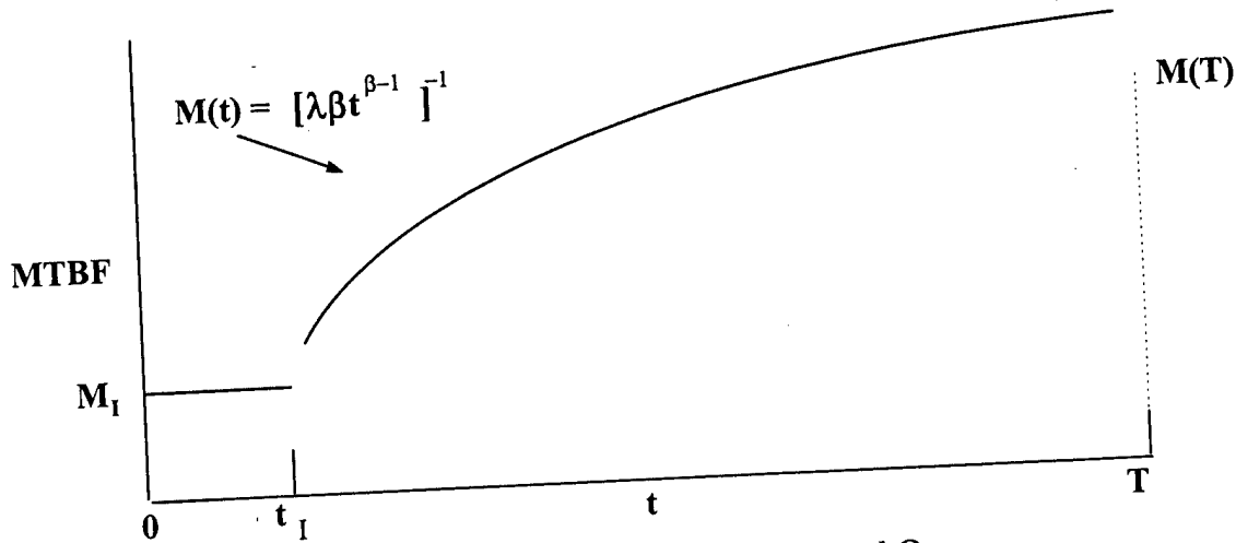
Figure 5. Reliability Growth Based On AMSAA Continuous Tracking Model.
