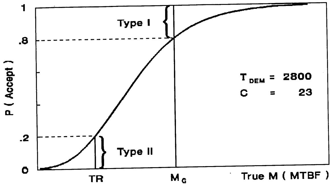
Figure 1. Example OC Curve for Reliability Demonstration Test.
