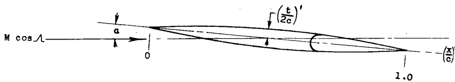
Wing at angle of attack Section B-B
