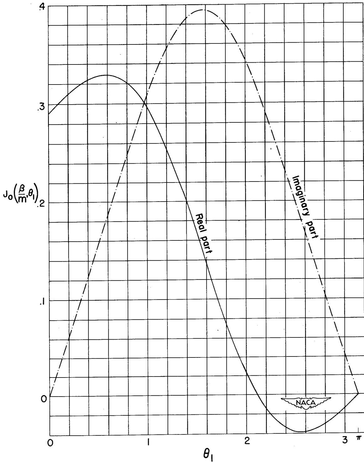
Figure 20.- Incomplete Bessel function of zero order J_0\left(\frac{\beta}{m}, \theta_1\right) for M = 1.5 and \beta = \pi/2 .
