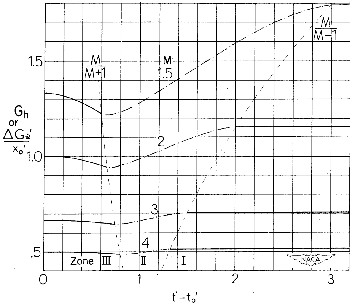
Figure 4.- Plot of G_h or \frac{\Delta G_{a'}}{x_0'} as a function of t' - t_0' at various Mach
