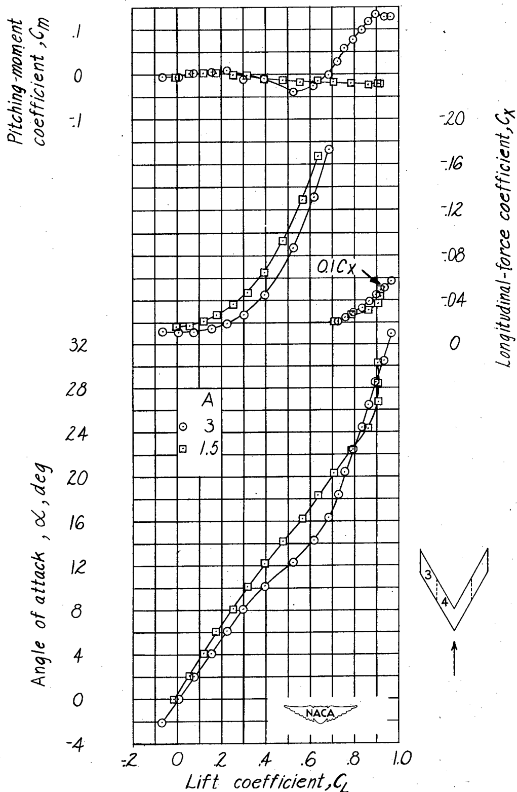
Figure 9.- Aerodynamic characteristics of sweptback wings. \Lambda_{c/4} = 60^\circ ; A = 3 and 1.5 ; \lambda = 1 ; NACA 0015 airfoil section; models 3 and 4.
