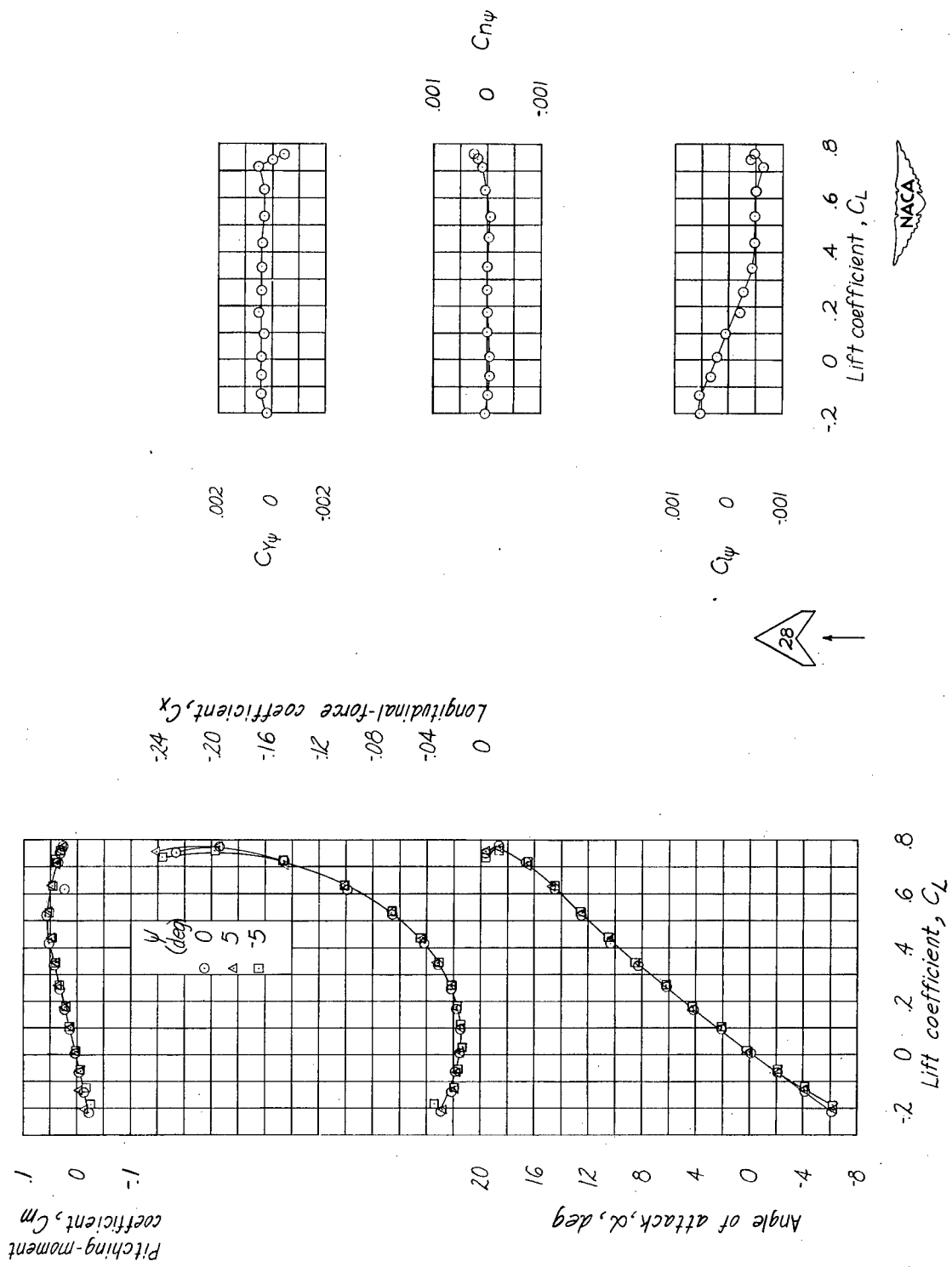
Figure 32.- Aerodynamic characteristics of a sweptforward wing. \Lambda_c/4 = -45^\circ ; A = 2.1 ; \lambda = 3.88 ; NACA 23012 airfoil section; model 28.
