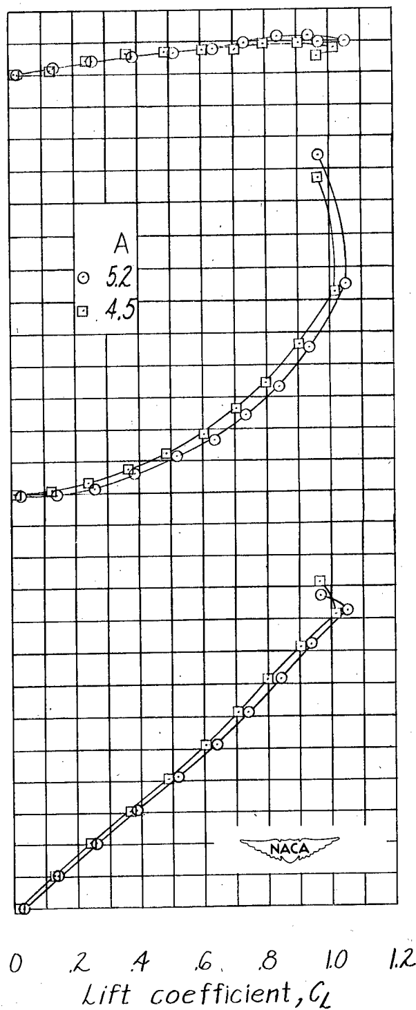
Figure 15.- Aerodynamic characteristics of sweptback wings. \Lambda_c/4 = 30^\circ ; A = 5.2 and 4.5 ; \lambda = 1 ; NACA 0015 airfoil section; models 10 and 11.
