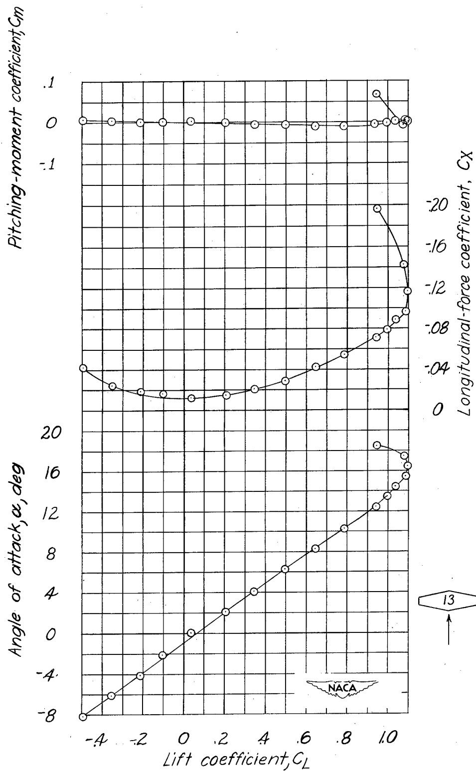
Figure 17.- Aerodynamic characteristics of a sweptback wing. \Lambda_{c/4} = 60^\circ ; A = 6 ; \lambda = 5 ; NACA 23012 airfoil section; model 13.
