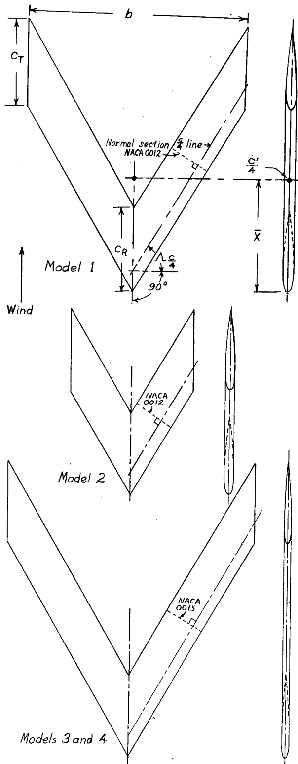
Figure 2.- Plan forms and dimensions of wing models.
