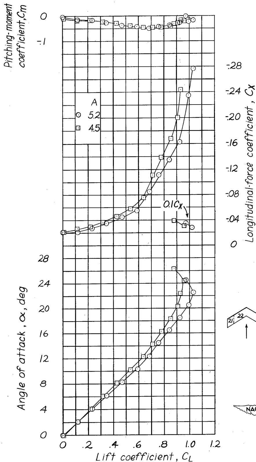
Figure 25.- Aerodynamic characteristics of sweptforward wings. \Lambda_{c/4} = -30^\circ ; A = 5.2 and 4.5 ; \lambda = 1 ; NACA 0015 airfoil section; models 21 and 22.
