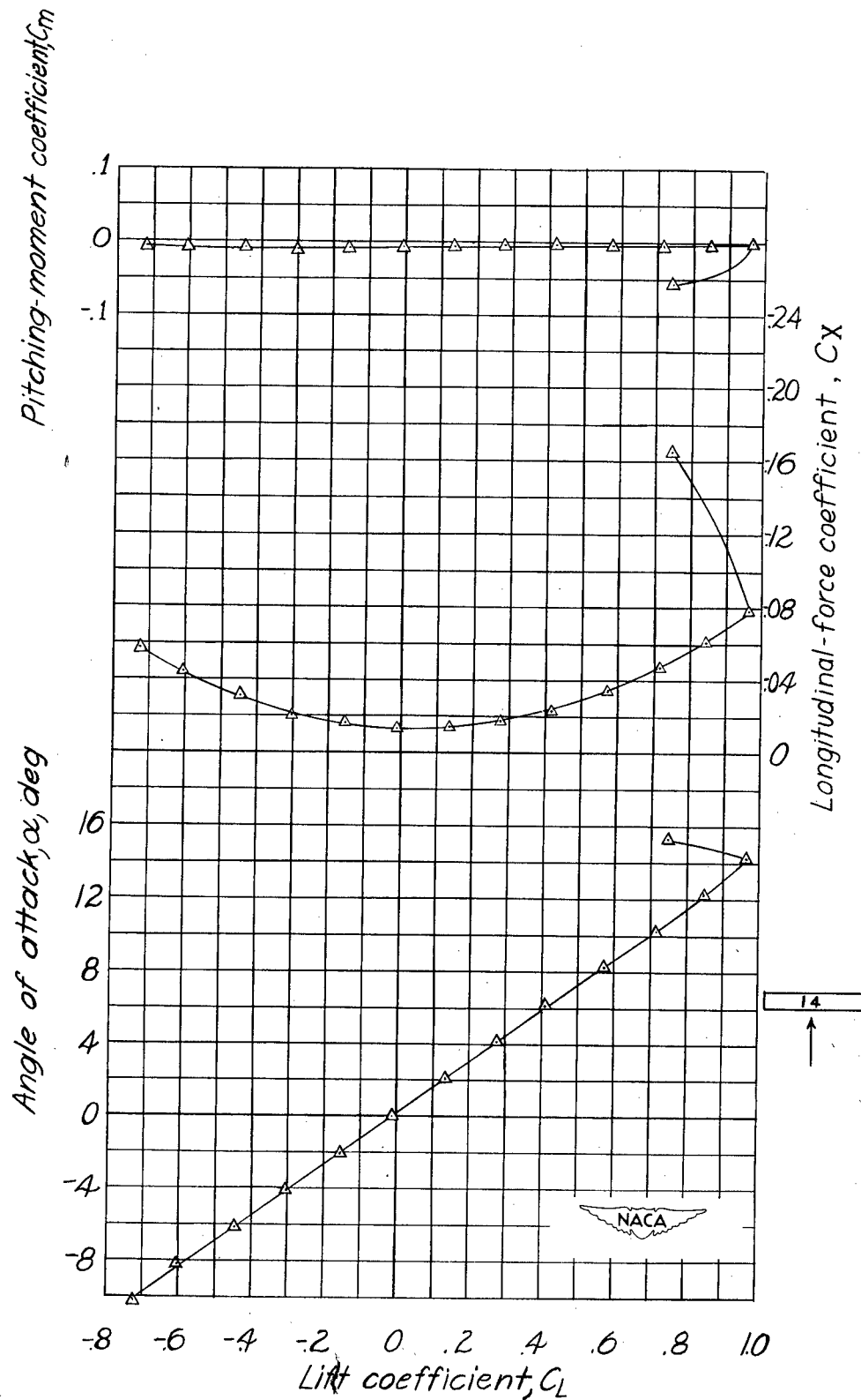
Figure 18.- Aerodynamic characteristics of an unswept wing. \Lambda_{c/4} = 0^\circ ; A = 6 ; \lambda = 1 ; NACA 0012 airfoil section; model 14.
