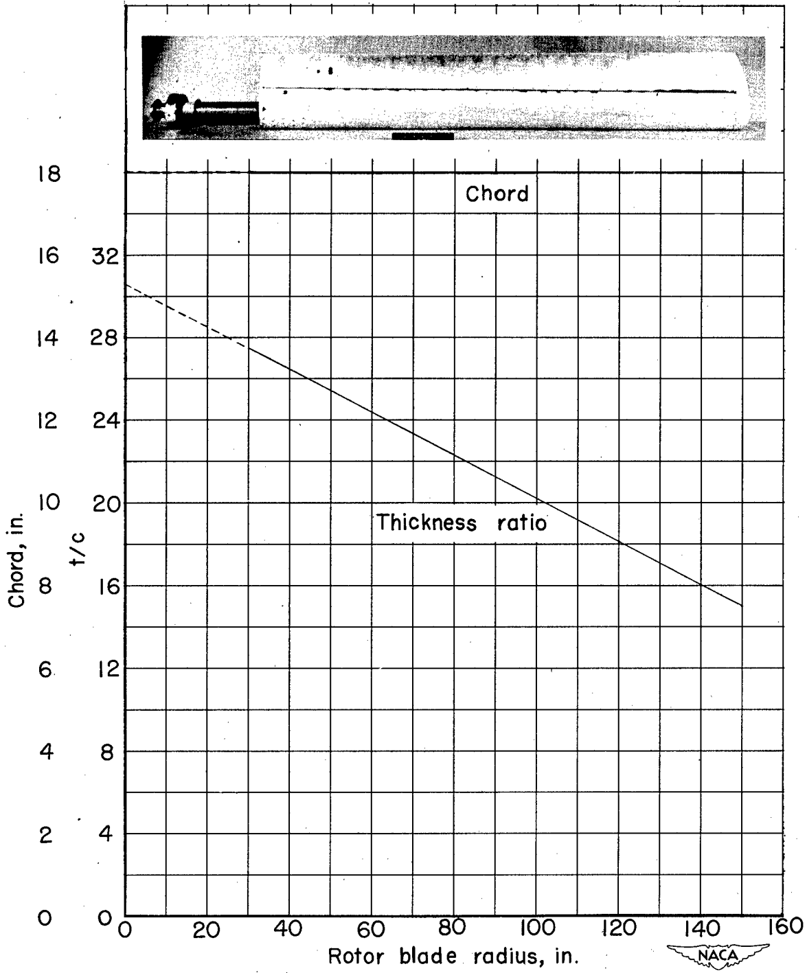
(b) Rotor 2.
