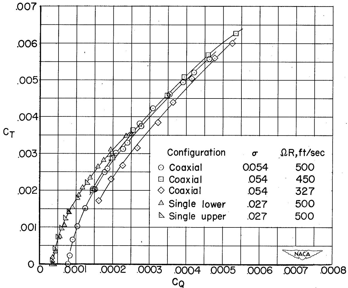
Figure 4.—Variation of thrust coefficient C_T and torque coefficient C_Q for a coaxial helicopter rotor (rotor I) in static thrust; yawing moments trimmed. c_r/c_t=2.92 .
