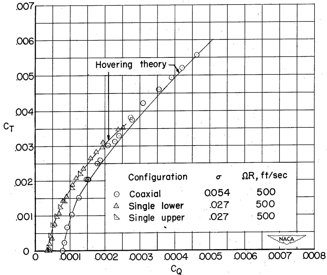
Figure 7.—Comparison of the theoretical and experimental static-thrust performance of a coaxial helicopter rotor (rotor 1) with blades tapered both in plan form and thickness ratio. c_r/c_t=2.92 .
