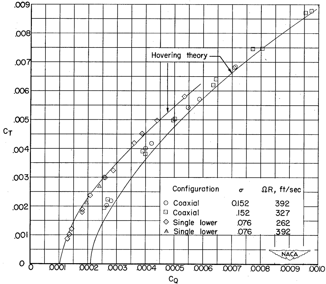
Figure 10.—Comparison of the theoretical and experimental static-thrust performance of a coaxial helicopter rotor (rotor 2) with blades tapered in thickness ratio only. c_r/c_f=1 .
