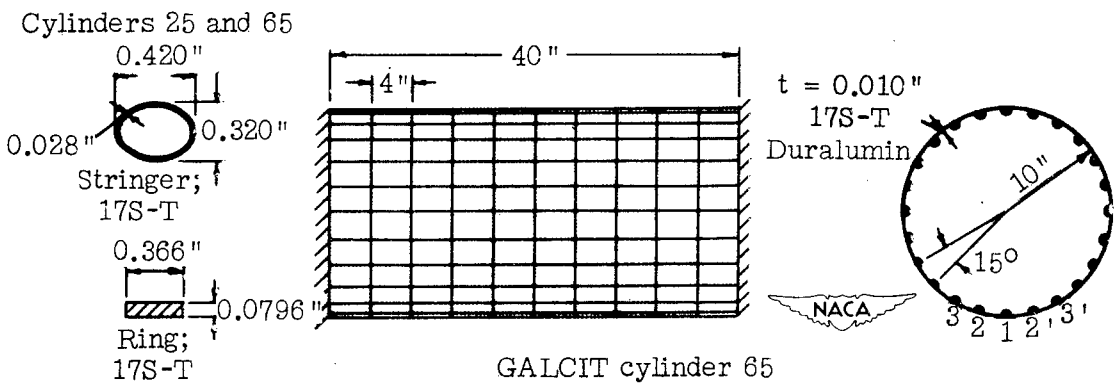
Figure 1.- Cylinder characteristics.
