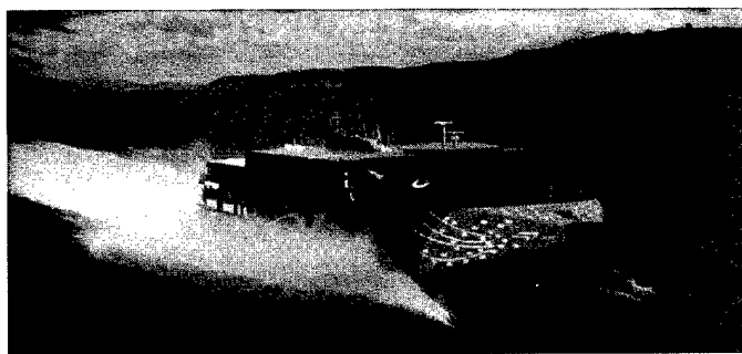
Figure 5. Bow View of 91-Meter Wave-Piercing Ferry INCAT-046 Running at 43 Knots
